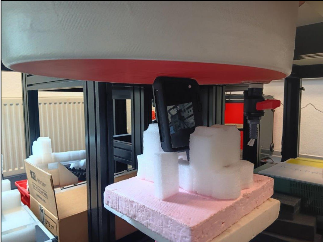
Photo 11: Test position - Top side with 0mm distance
