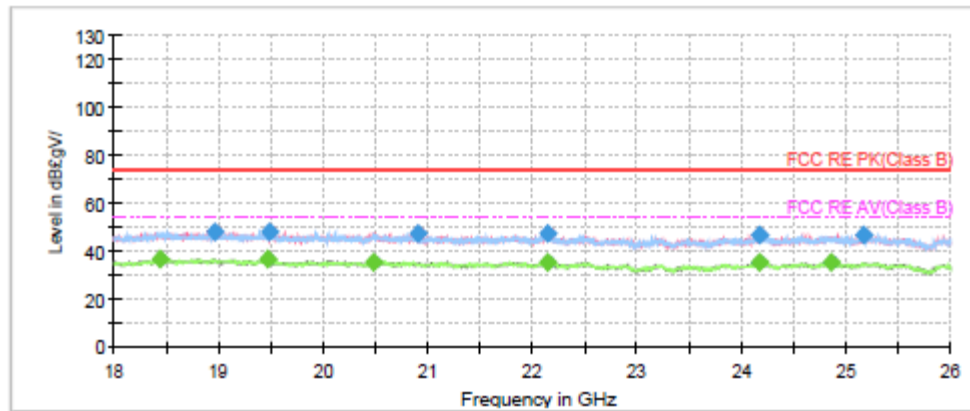
Radiates Emission from 18GHz to 26GHz
