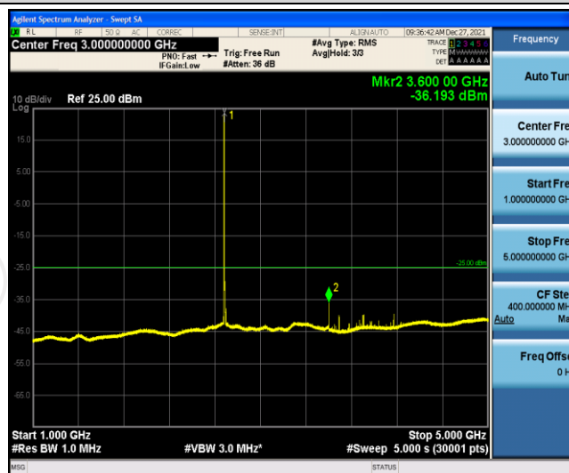
Band41-10MHz-16QAM-41540-1RB#0-Range5:5000~12000MHz
