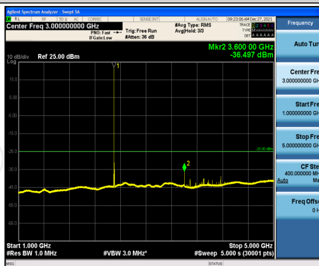
Band41-10MHz-QPSK-39700-1RB#0-Range5:5000~12000MHz
