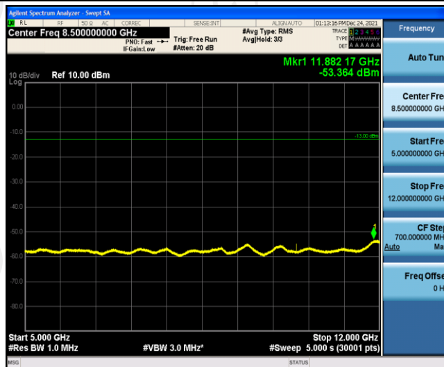
Band4-15MHz-QPSK-20175-1RB#0-Range6:12000~26500MHz
