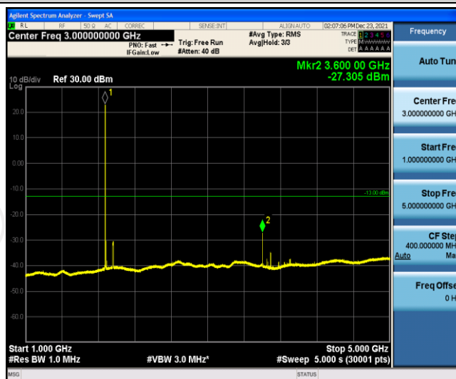
Band2-10MHz-16QAM-18900-1RB#0-Range5:5000~12000MHz
