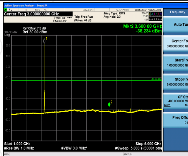
Band2-5MHz-QPSK-18900-1RB#0-Range5:5000~12000MHz
