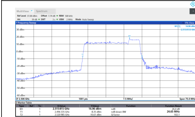
41-41-20MHz-5MHz-QPSK-QPSK-41440-41557-100R B#0-25RB#0
