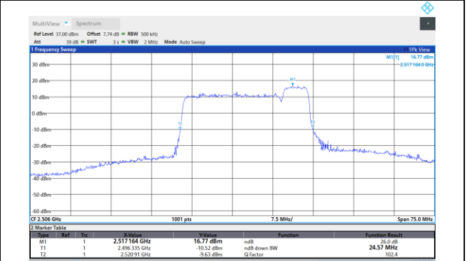
41-41-20MHz-5MHz-16QAM-16QAM-41440-41557-10 ORB#0-25RB#0
