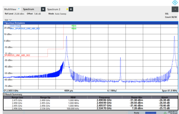
41-41-20MHz-20MHz-QPSK-QPSK-41292-4149 0-100RB#0-100RB#0
