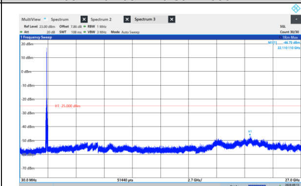
41-41-20MHz-20MHz-16QAM-16QAM-39750-39948 -100RB#0-100RB#0-30~27000MHz
