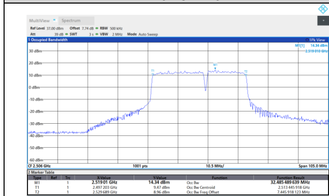
41-41-20MHz-15MHz-QPSK-QPSK-41341-41512-100 RB#0-75RB#0
