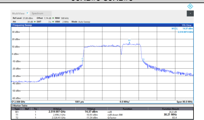
41-41-20MHz-10MHz-64QAM-64QAM-41391-41535-1 00RB#0-50RB#0
