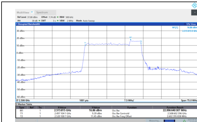
41-41-20MHz-5MHz-QPSK-QPSK-41440-41557-100R B#0-25RB#0
