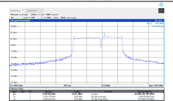
41-41-20MHz-15MHz-16QAM-16QAM-39750-39921-1 00RB#0-75RB#0
