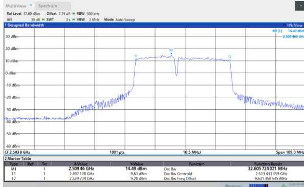
41-41-15MHz-20MHz-QPSK-QPSK-41319-41490-75R B#0-100RB#0
