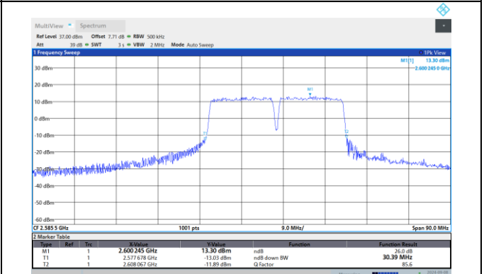
41-41-15MHz-15MHz-64QAM-64QAM-39725-39875-7 5RB#0-75RB#0
