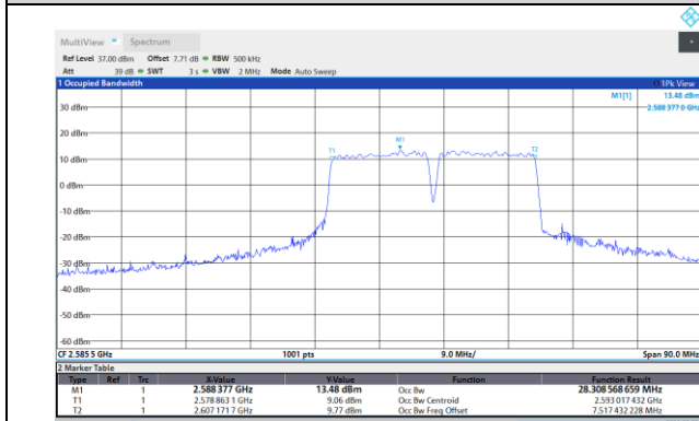
41-41-15MHz-20MHz-QPSK-QPSK-39728-39899-75R
