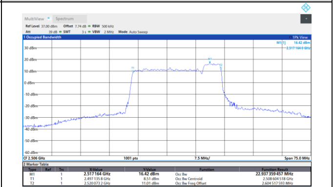
41-41-20MHz-5MHz-16QAM-16QAM-41440-41557-10ORB#0-25RB#0
