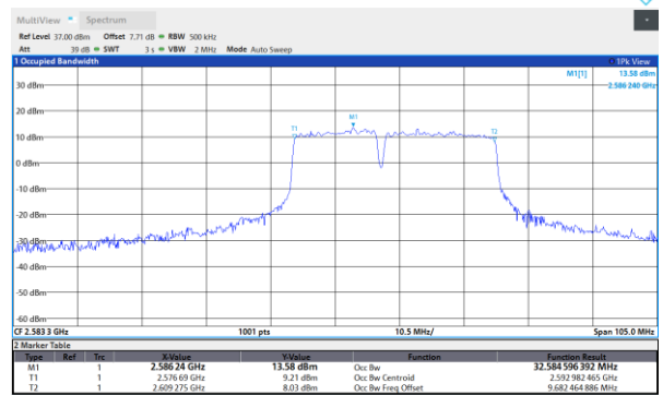
41-41-15MHz-20MHz-64QAM-64QAM-40523-40694-7 5RB#0-100RB#0
