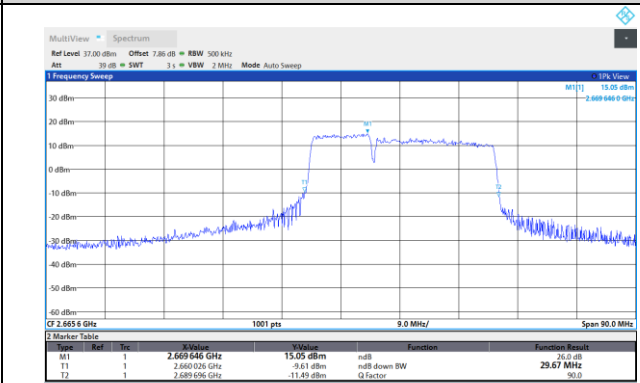
41-41-10MHz-20MHz-16QAM-16QAM-40526-40670-5
