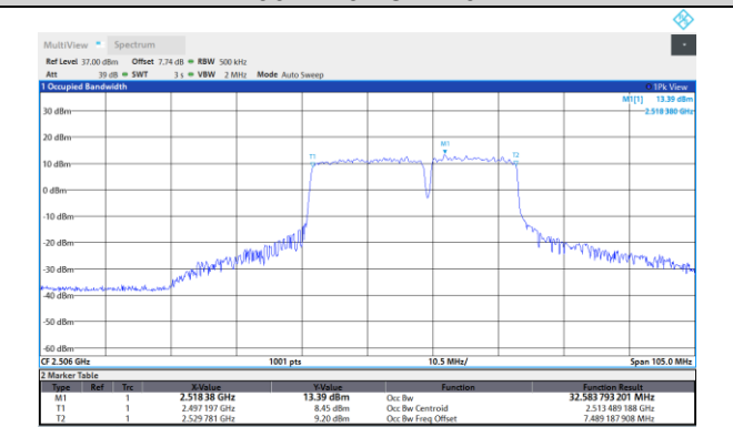
41-41-20MHz-15MHz-16QAM-16QAM-41341-41512-1
