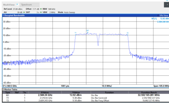
41-41-15MHz-20MHz-64QAM-64QAM-39728-39899-7 5RB#0-100RB#0
