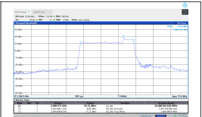
41-41-20MHz-5MHz-16QAM-16QAM-39750-39867-10ORB#0-25RB#0
