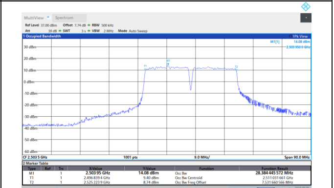
41-41-15MHz-15MHz-64QAM-64QAM-41365-41515-7 5RB#0-75RB#0
