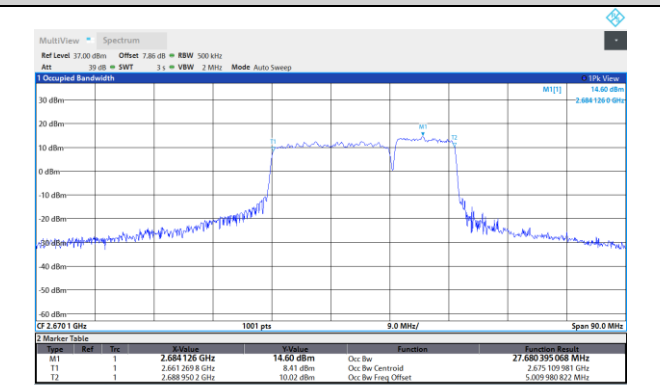
41-41-20MHz-15MHz-QPSK-QPSK-40546-40717-100 RB#0-75RB#0
