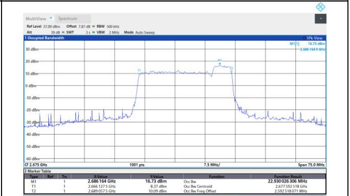
41-41-20MHz-5MHz-64QAM-64QAM-40595-40712-10ORB#0-25RB#0
