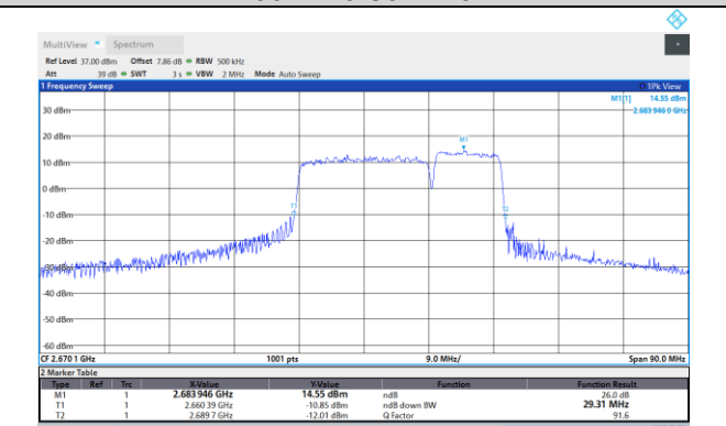
41-41-20MHz-15MHz-QPSK-QPSK-40546-40717-100 RB#0-75RB#0
