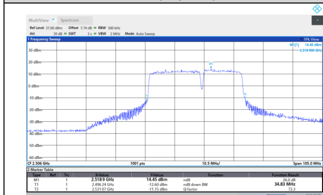
41-41-20MHz-15MHz-QPSK-QPSK-41341-41512-100
