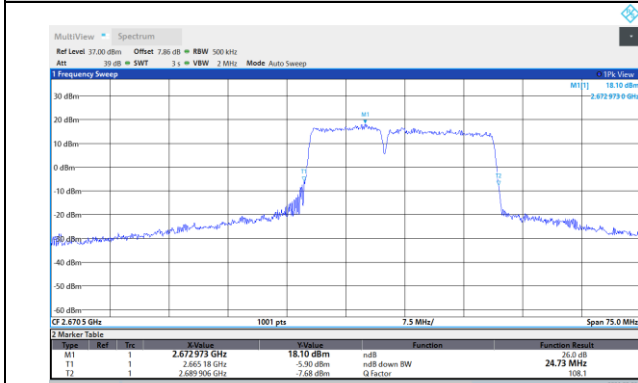
41-41-10MHz-20MHz-QPSK-QPSK-40526-40670-50R B#0-100RB#0
