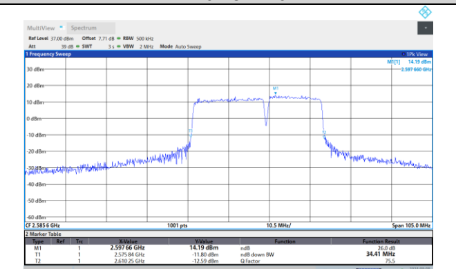
41-41-20MHz-15MHz-16QAM-16QAM-39750-39921-1
