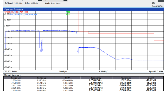
7-7-20MHz-20MHz-64QAM-64QAM-21152-21350-21048-1RB#99-1RB#0
