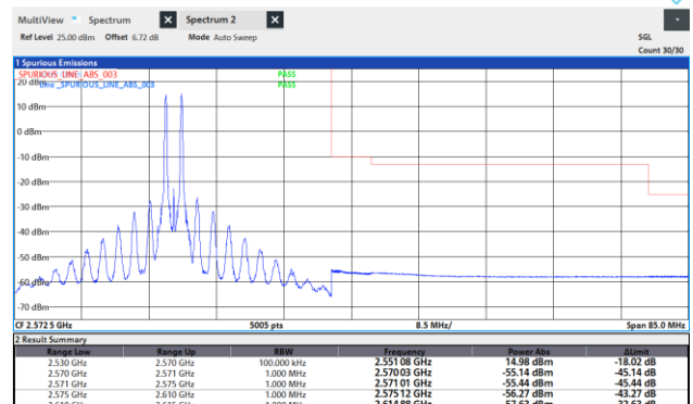
7-7-20MHz-20MHz-16QAM-16QAM-20850-21048-2 1048-1RB#0-1RB#99
