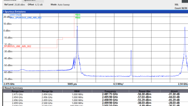
7-7-20MHz-20MHz-16QAM-16QAM-21152-21350-21048-100RB#0-100RB#0
