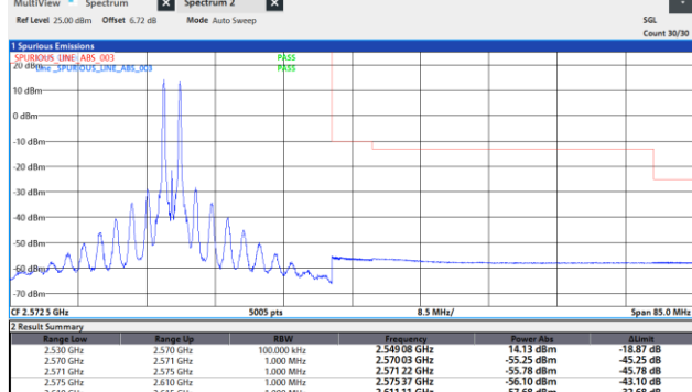
7-7-20MHz-20MHz-64QAM-64QAM-20850-21048-21048-1RB#0-1RB#99
