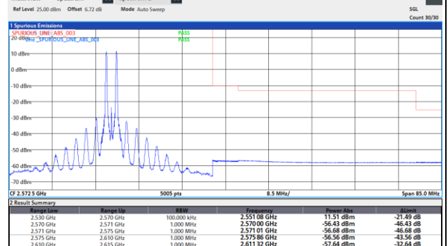
7-7-20MHz-20MHz-64QAM-64QAM-21152-21350-21048-1RB#99-1RB#0
