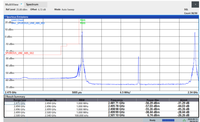
7-7-20MHz-20MHz-QPSK-QPSK-21152-21350-210 48-100RB#0-100RB#0
