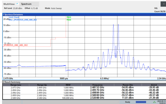
7-7-20MHz-20MHz-64QAM-64QAM-21152-21350-21048-1RB#0-1RB#99
