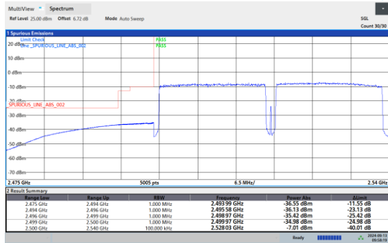
7-7-20MHz-20MHz-64QAM-64QAM-20850-21048-1RB#99-1RB#0
