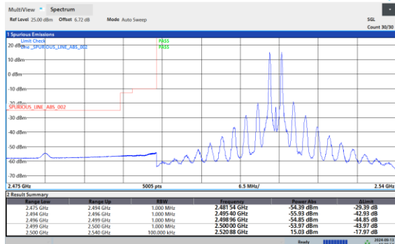
7-7-20MHz-20MHz-QPSK-QPSK-21152-21350-21048-1R B#0-1RB#99
