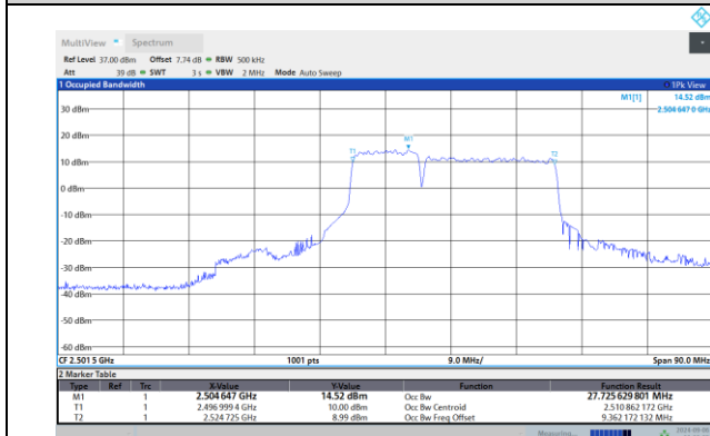
41-41-10MHz-20MHz-16QAM-16QAM-41346-41490-5
