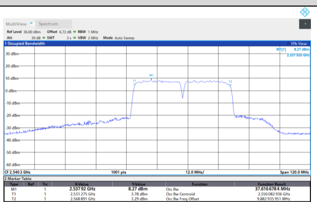
7-7-20MHz-20MHz-16QAM-16QAM-21152-21350-10 ORB#0-100RB#0
