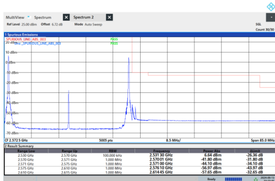
7-7-20MHz-20MHz-16QAM-16QAM-20850-21048-21048- 100RB#0-100RB#0
