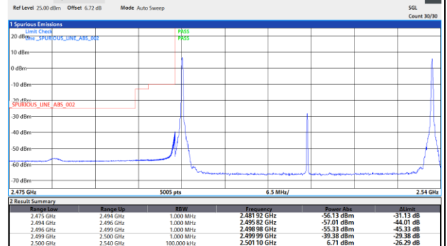
7-7-20MHz-20MHz-64QAM-64QAM-21152-21350-21048-100RB#0-100RB#0
