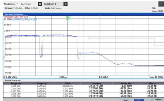
7-7-20MHz-20MHz-QPSK-QPSK-21152-21350-210 48-1RB#99-1RB#0
