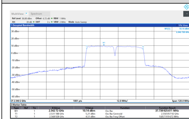
7-7-20MHz-20MHz-16QAM-16QAM-21001-21199-10 ORB#0-100RB#0
