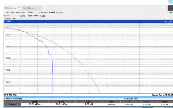
Band41-20MHz-16QAM-40620-100RB#0
