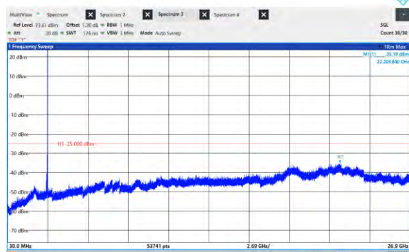
Band41-5MHz-64QAM-40620-1RB#0-Range:30~26900 0MHz
