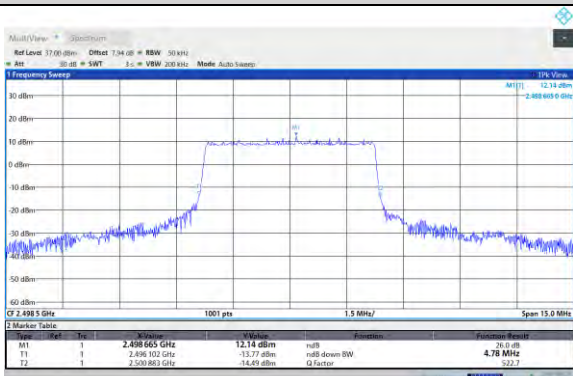
Band41-5MHz-64QAM-41565-25RB#0
