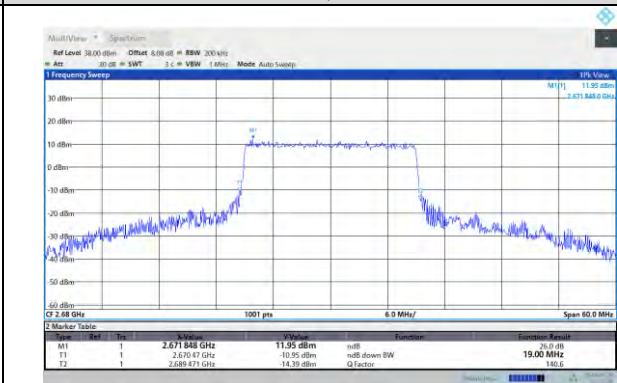
Band41-20MHz-64QAM-41490-100RB#0
