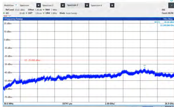
Band41-5MHz-16QAM-39675-1RB#0-Range:30~26900 0MHz
