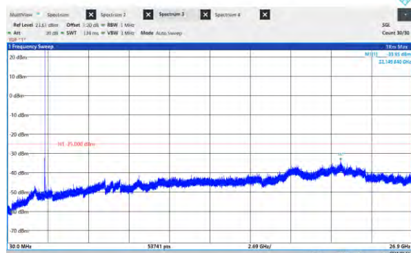
Band41-5MHz-16QAM-41565-1RB#0-Range:30~26900 0MHz
