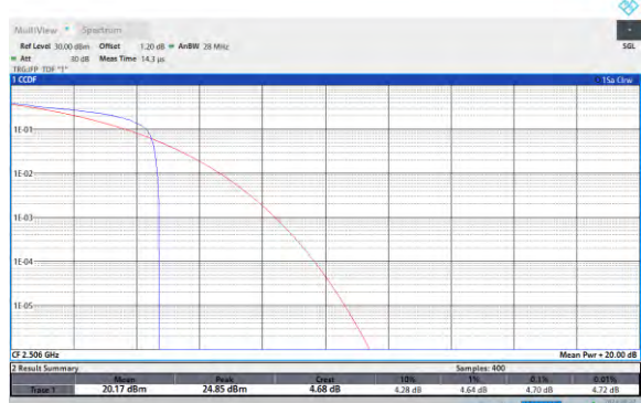
Band41-20MHz-64QAM-40620-1RB#0
