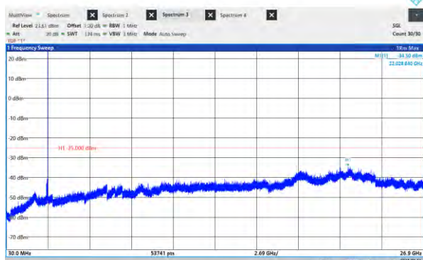
Band41-5MHz-16QAM-40620-1RB#0-Range:30~26900 MHz
