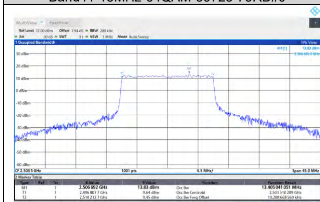
Band41-15MHz-64QAM-41515-75RB#0
