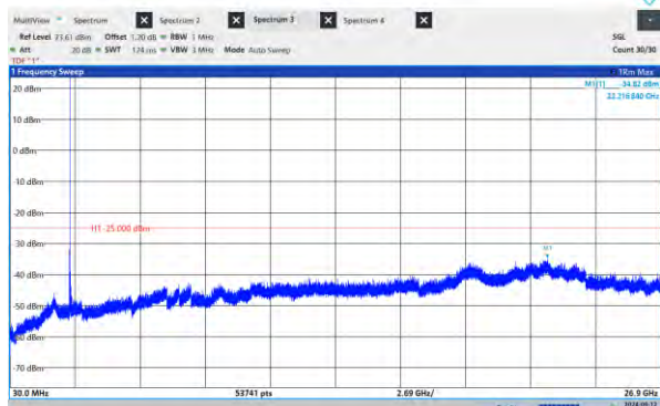
Band41-5MHz-QPSK-41565-1RB#0-Range:30~26900 MHz
