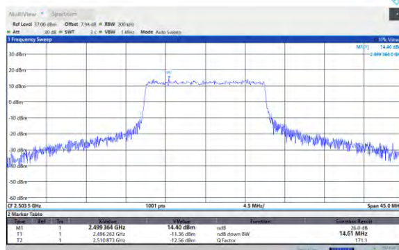
Band41-15MHz-16QAM-41515-75RB#0
