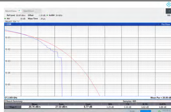
Band41-15MHz-16QAM-41515-75RB#0
