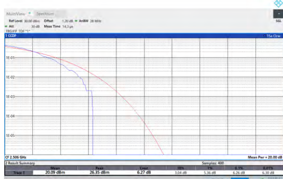
Band41-20MHz-64QAM-40620-100RB#0
