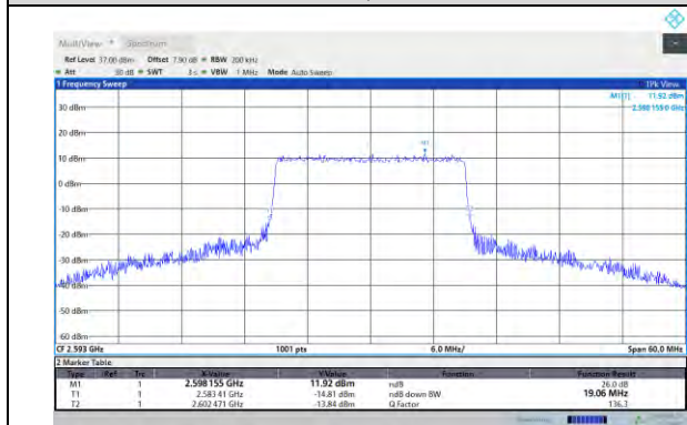
Band41-20MHz-64QAM-40620-100RB#0
