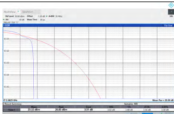
Band41-15MHz-16QAM-39725-1RB#0
