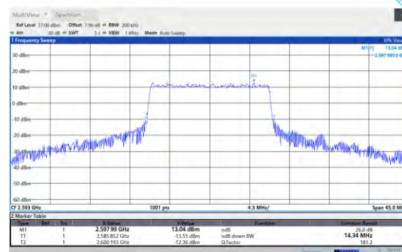
Band41-20MHz-QPSK-39750-100RB#0
