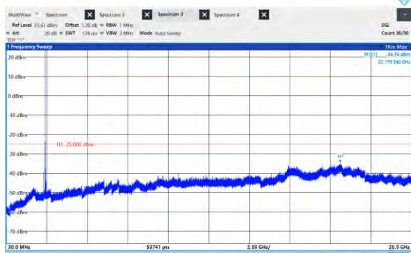
Band41-5MHz-64QAM-39675-1RB#0-Range:30~26900 MHz
