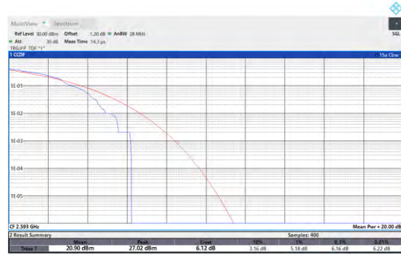
Band41-20MHz-16QAM-41490-100RB#0
