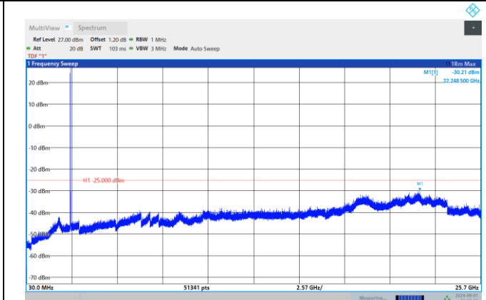
Band7-20MHz-QPSK-21350-1RB#0-Range:30~25700M Hz
