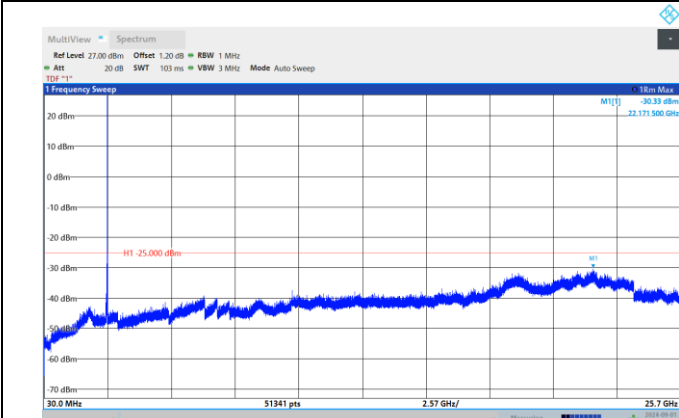
Band7-20MHz-64QAM-21100-1RB#0-Range:30~25700M Hz
