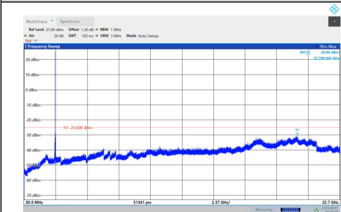
Band7-20MHz-64QAM-21100-1RB#0-Range:30~25700M Hz
