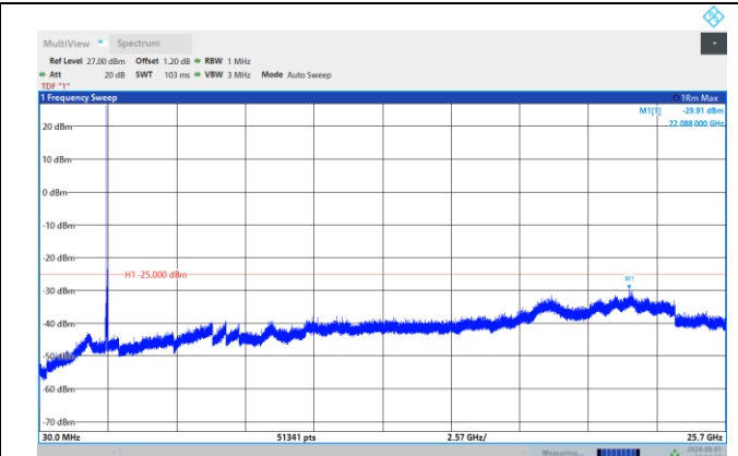
Band7-20MHz-64QAM-20850-1RB#0-Range:30~25700 MHz
