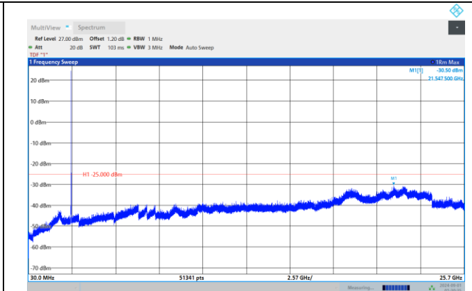
Band7-20MHz-QPSK-20850-1RB#0-Range:30~25700M Hz
