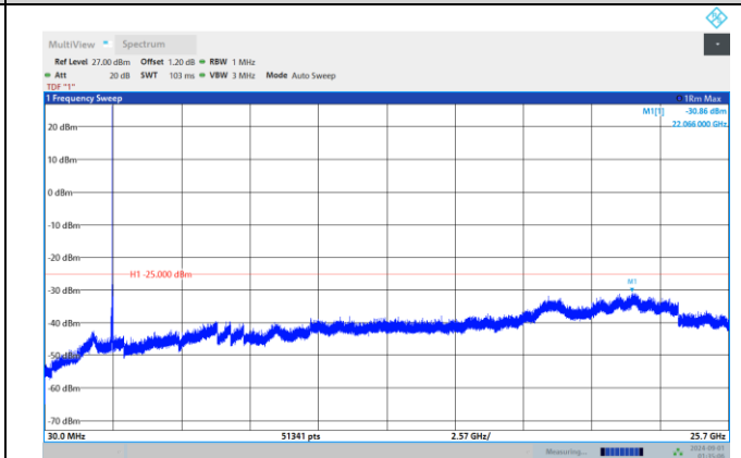
Band7-20MHz-16QAM-21100-1RB#0-Range:30~25700 MHz
