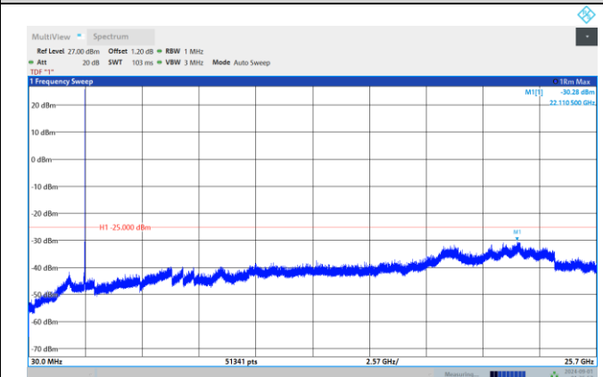
Band7-20MHz-64QAM-21350-1RB#0-Range:30~25700 MHz
