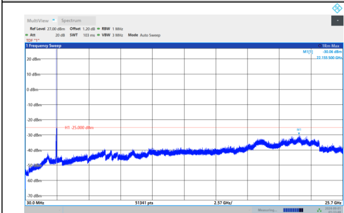
Band7-20MHz-16QAM-20850-1RB#0-Range:30~25700M Hz
