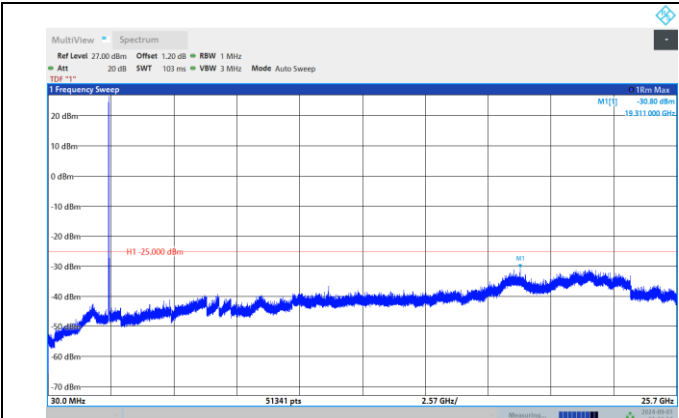
Band7-20MHz-16QAM-21350-1RB#0-Range:30~25700M Hz
