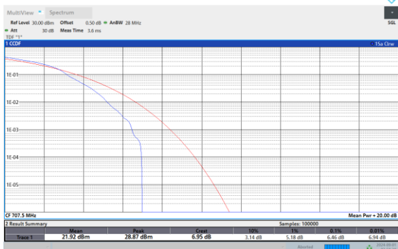
Band12-1.4MHz-16QAM-23173-1RB#0
