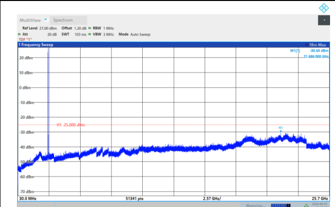
Band7-20MHz-64QAM-21350-1RB#0-Range:30~25700 MHz
