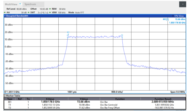
Band2-3MHz-64QAM-19185-15RB#0
