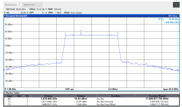
Band2-20MHz-64QAM-18700-100RB#0
