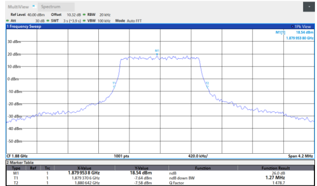
Band2-1.4MHz-16QAM-18607-6RB#0
