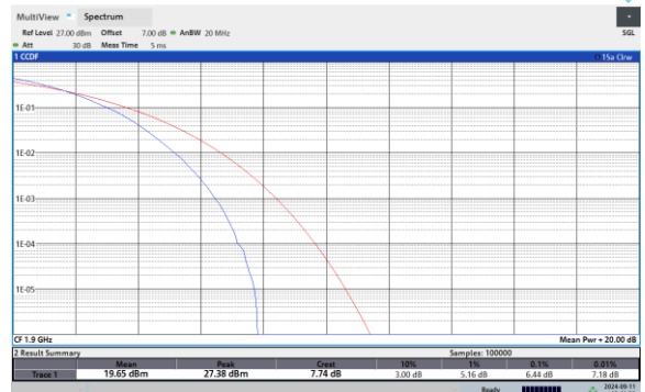
Band2-20MHz-64QAM-19100-100RB#0
