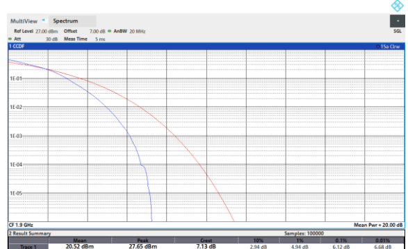
Band2-20MHz-64QAM-18700-100RB#0
