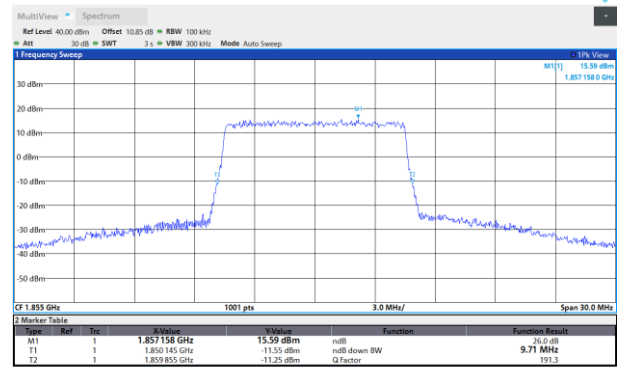
Band2-10MHz-64QAM-19150-50RB#0
