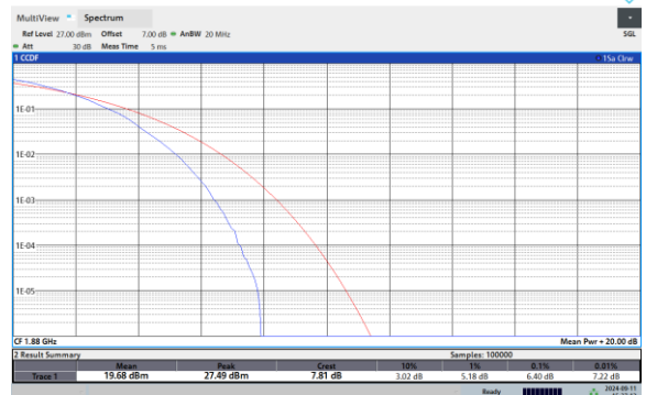
Band2-20MHz-64QAM-19100-100RB#0
