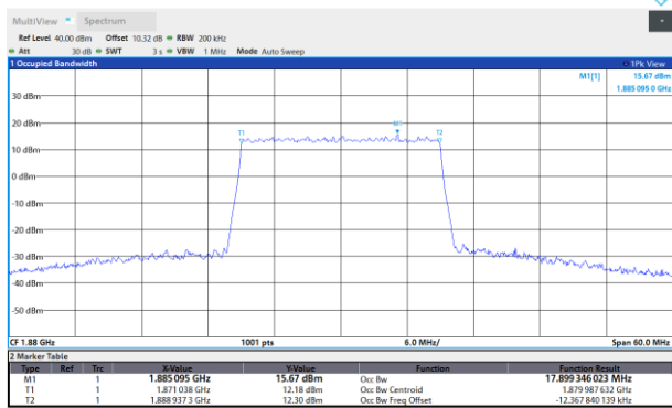
Band2-20MHz-64QAM-18900-100RB#0
