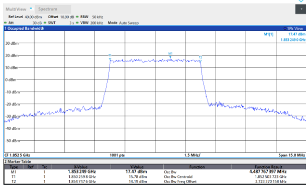
Band2-5MHz-QPSK-19175-25RB#0
