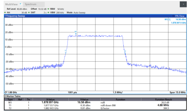
Band2-5MHz-16QAM-18625-25RB#0
