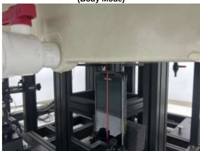
Bottom Side of EUT with 1.2 cm Gap (Body Mode)
