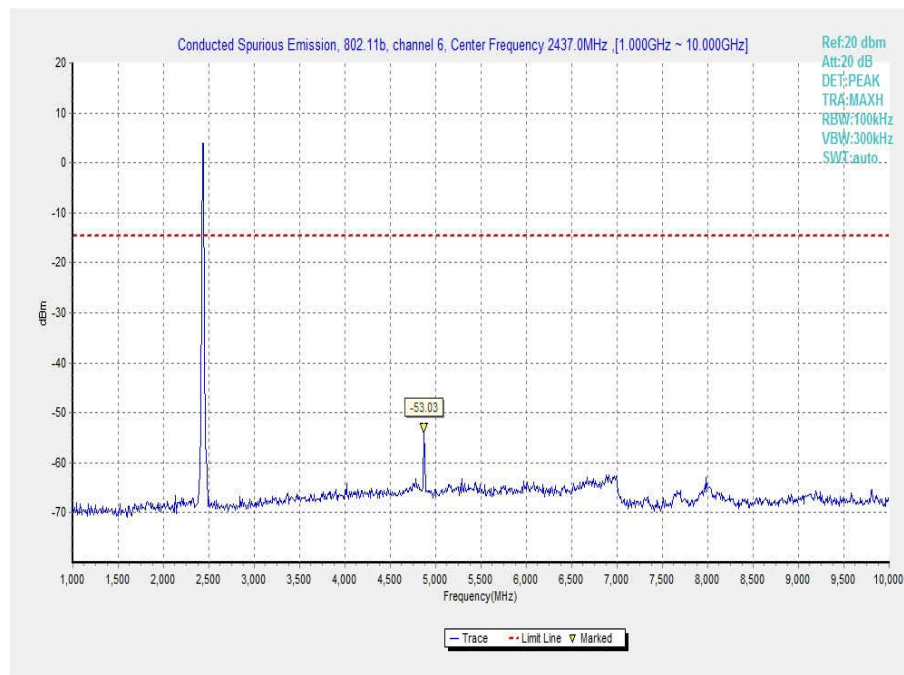
Fig.39 Conducted Spurious Emission (802.11b, Ch6, 1 GHz-10 GHz)
