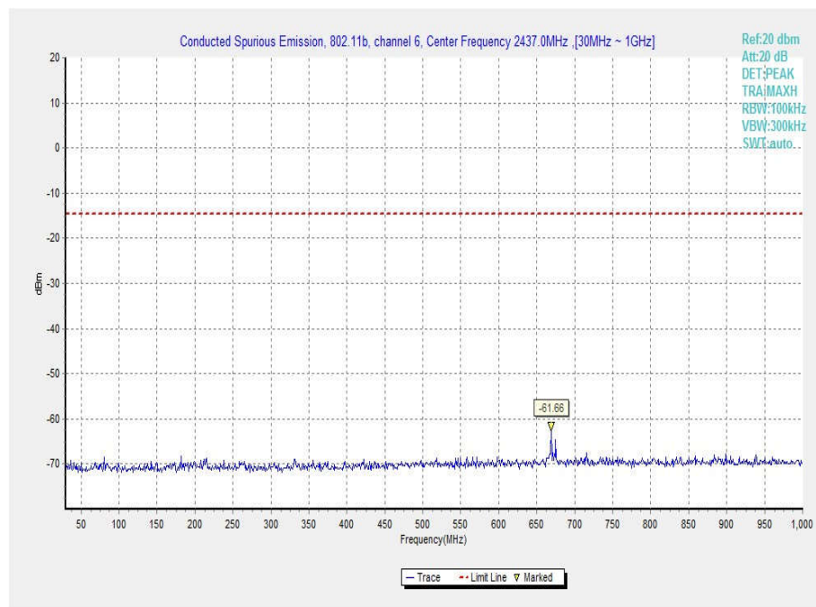
Fig.38 Conducted Spurious Emission (802.11b, Ch6, 30 MHz-1 GHz)
