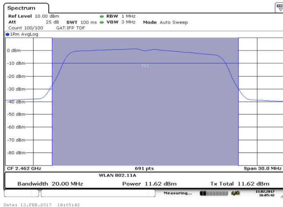
Fig.6 Maximum Average Output Power (802.11g, Ch 11, 18Mbps)
