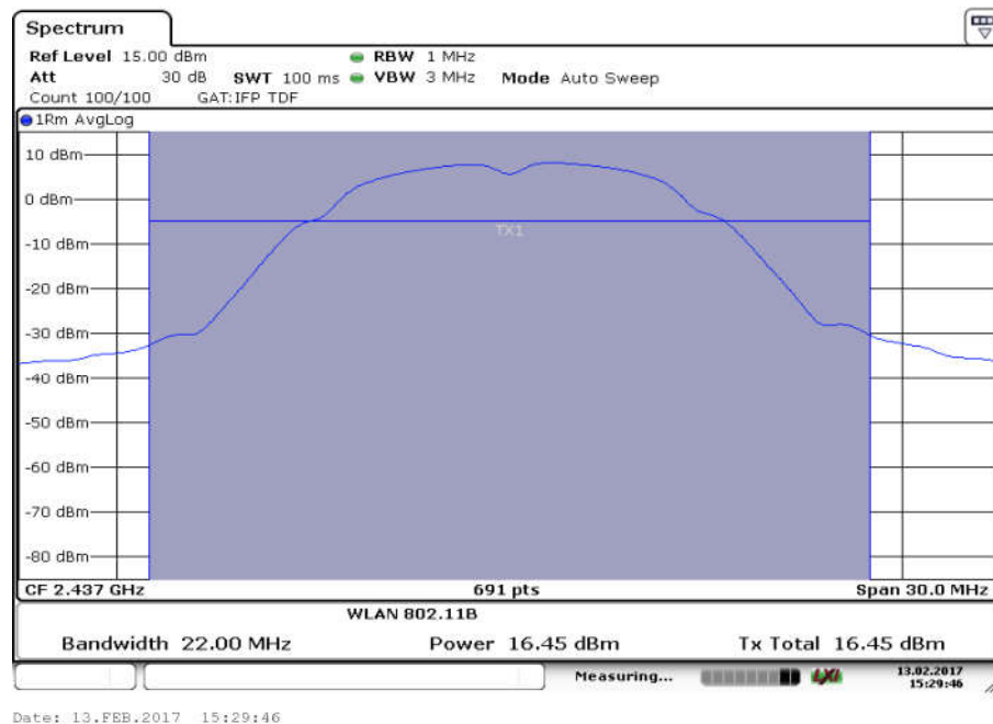
Fig.2 Maximum Average Output Power (802.11b, Ch 6, 5.5Mbps)
