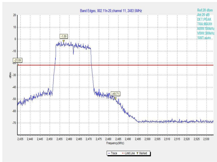
Fig.33 Band Edges (802.11 n-20MHz, Ch 11)
