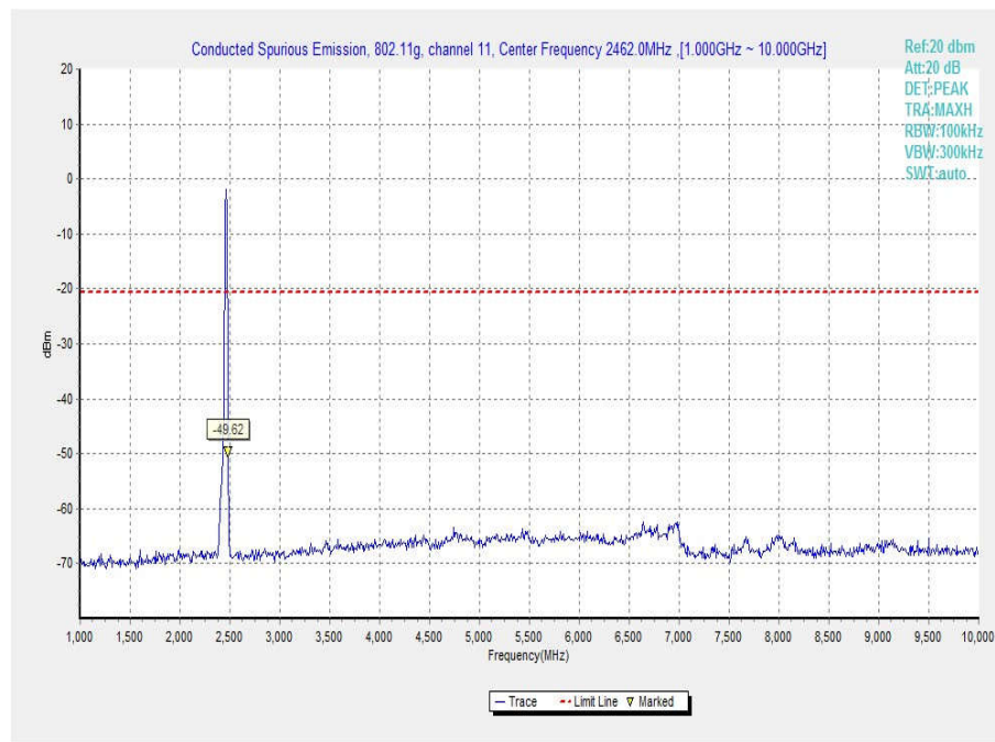
Fig.51 Conducted Spurious Emission (802.11g, Ch11, 1 GHz-10 GHz)
