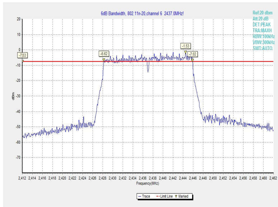
Fig.26 6dB Bandwidth (802.11 n-20MHz, Ch 6)
