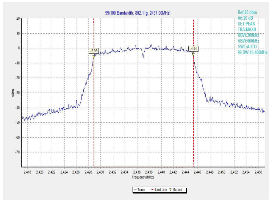
Fig.90 99% Occupied Bandwidth (802.11g, Ch 6)
