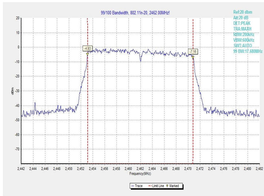
Fig.94 99% Occupied Bandwidth (802.11n-20MHz, Ch 11)
