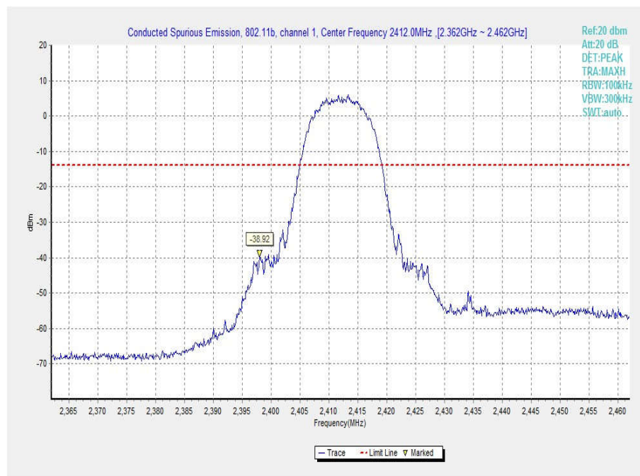
Fig.34 Conducted Spurious Emission (802.11b, Ch1, Center Frequency)
