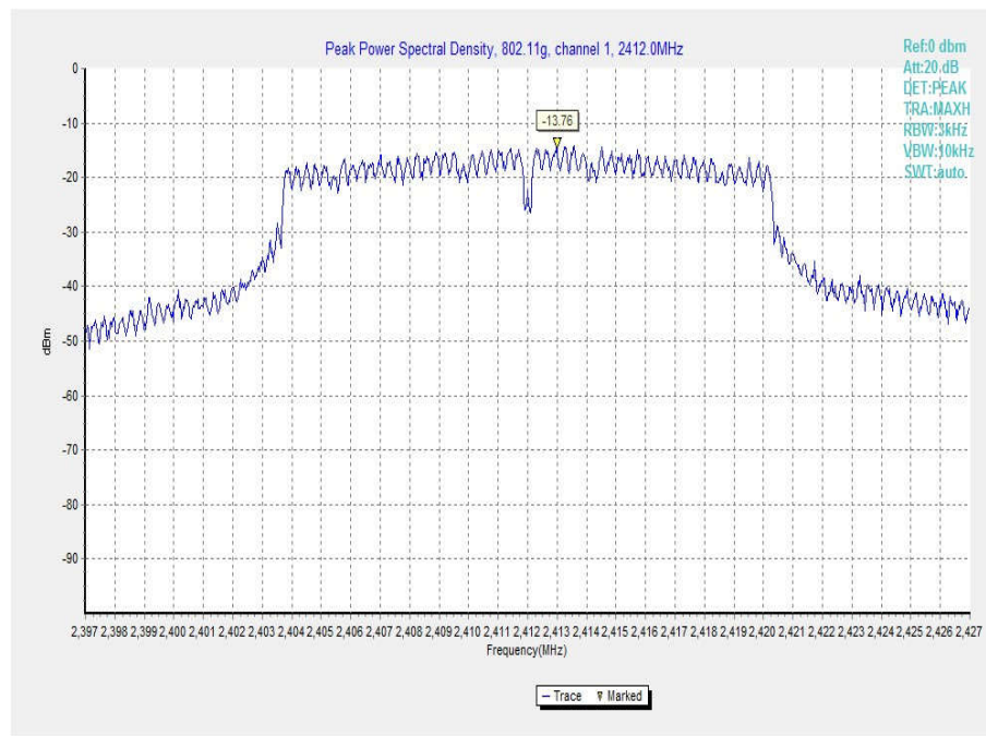
Fig.13 Power Spectral Density (802.11g, Ch 1)
