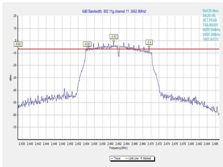
Fig.24 6dB Bandwidth (802.11g, Ch 11)
