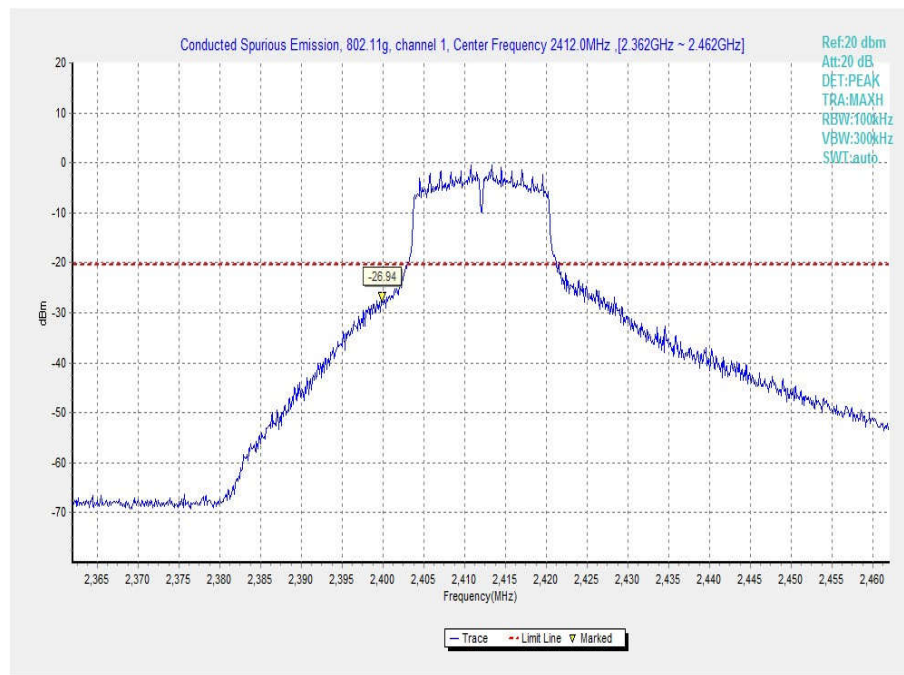
Fig.43 Conducted Spurious Emission (802.11g, Ch1, Center Frequency)
