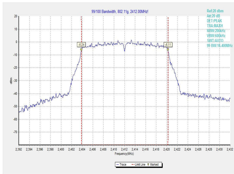
Fig.89 99% Occupied Bandwidth (802.11g, Ch 1)
