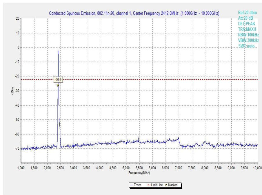
Fig.54 Conducted Spurious Emission (802.11n-20MHz, Ch1, 1 GHz-10 GHz)
