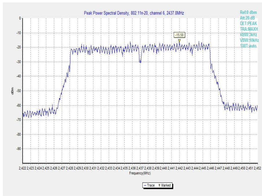
Fig.17 Power Spectral Density (802.11n-20MHz, Ch 6)
