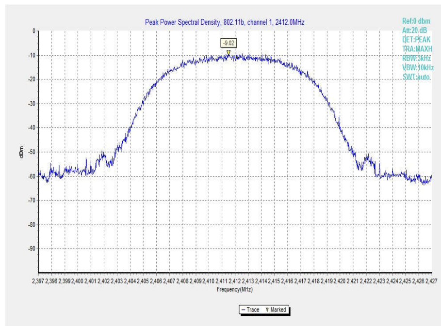
Fig.10 Power Spectral Density (802.11b, Ch 1)
