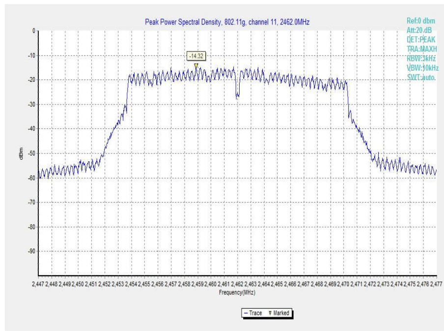
Fig.15 Power Spectral Density (802.11g, Ch 11)
