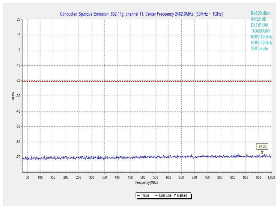
Fig.50 Conducted Spurious Emission (802.11g, Ch11, 30 MHz-1 GHz)
