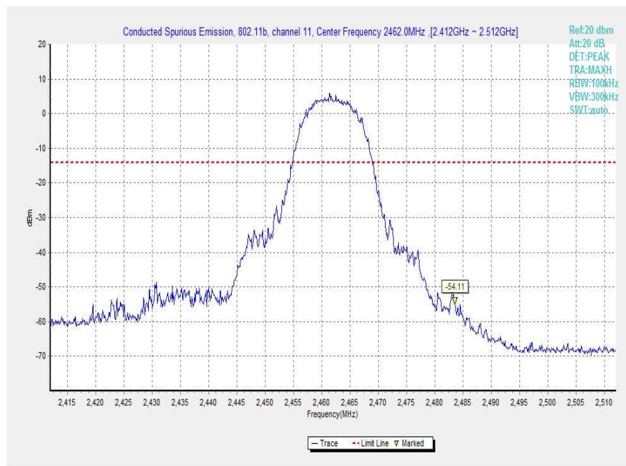
Fig.40 Conducted Spurious Emission (802.11b, Ch11, Center Frequency)
