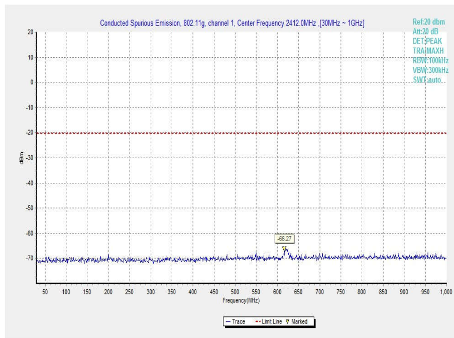
Fig.44 Conducted Spurious Emission (802.11g, Ch1, 30 MHz-1 GHz)
