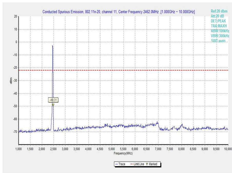
Fig.60 Conducted Spurious Emission (802.11n-20MHz, Ch11, 1 GHz-10 GHz)
