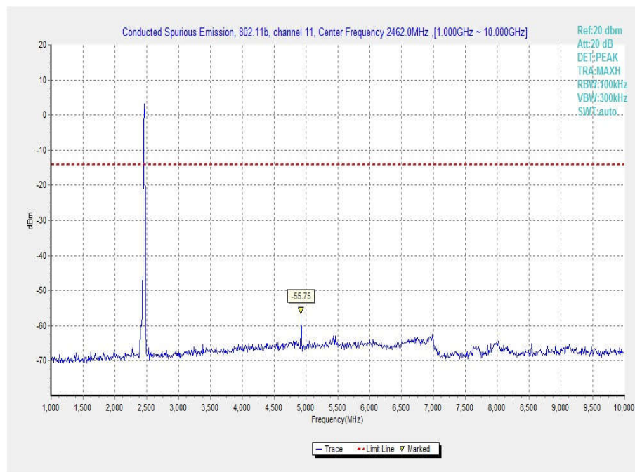
Fig.42 Conducted Spurious Emission (802.11b, Ch11, 1 GHz-10 GHz)
