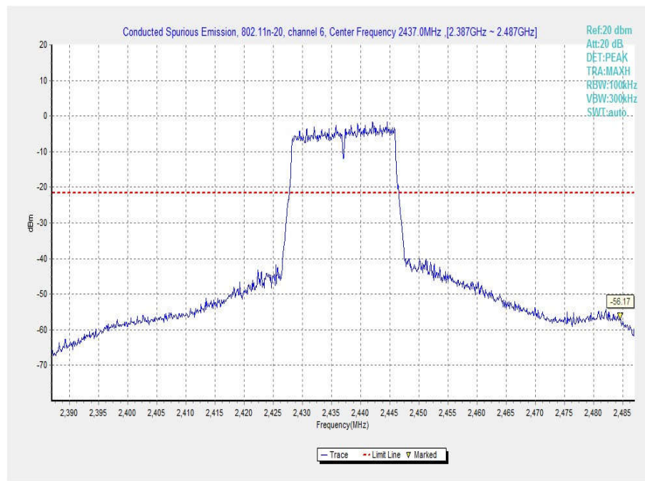
Fig.55 Conducted Spurious Emission (802.11n-20MHz, Ch6, Center Frequency)
