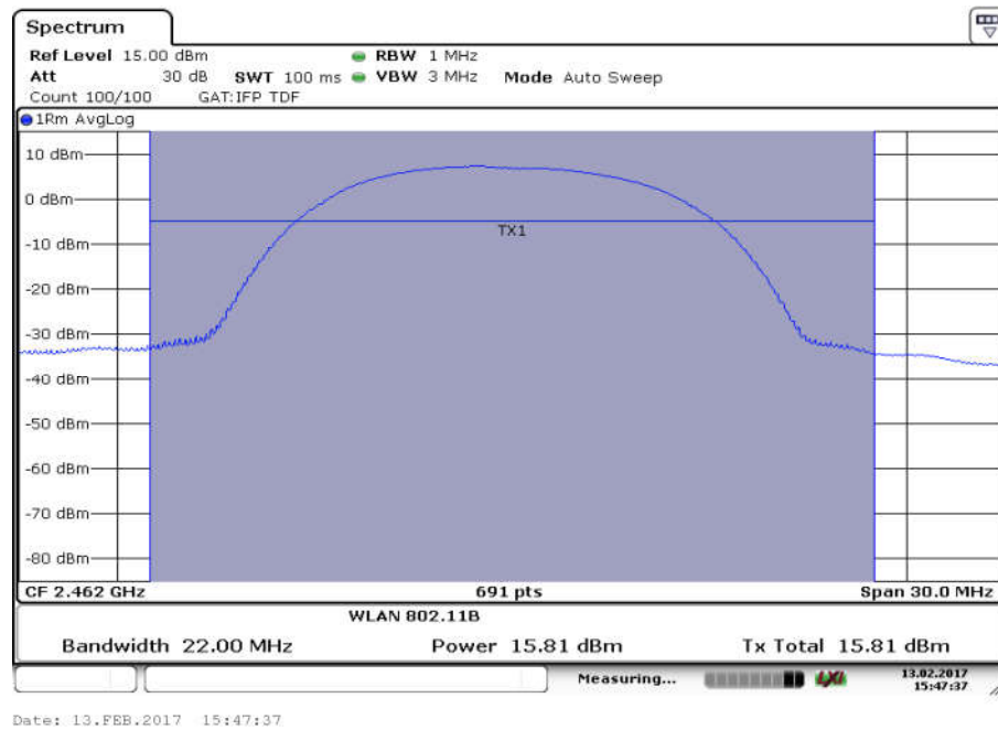
Fig.3 Maximum Average Output Power (802.11b, Ch 11, 5.5Mbps)
