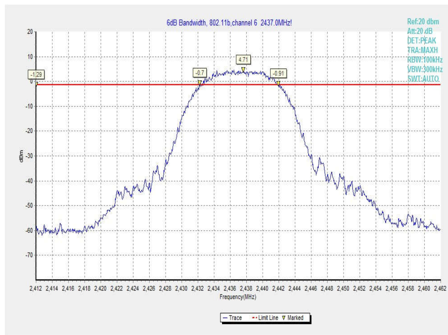
Fig.20 6dB Bandwidth (802.11b, Ch 6)
