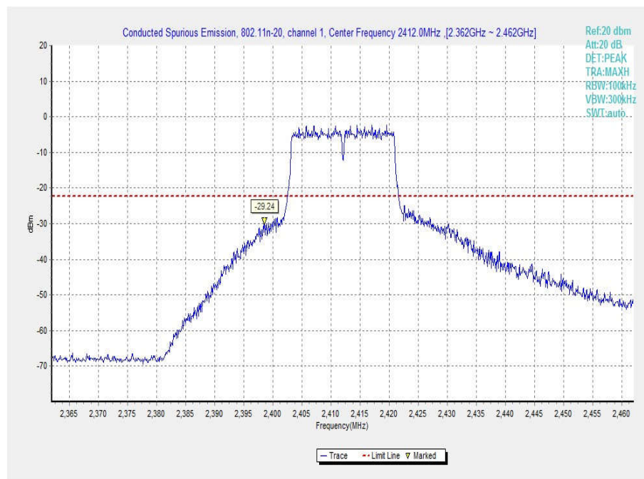
Fig.52 Conducted Spurious Emission (802.11n-20MHz, Ch1, Center Frequency)
