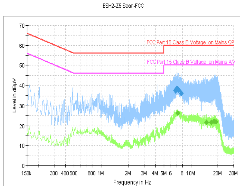
Fig.97 AC Powerline Conducted Emission (Traffic, AE1)
