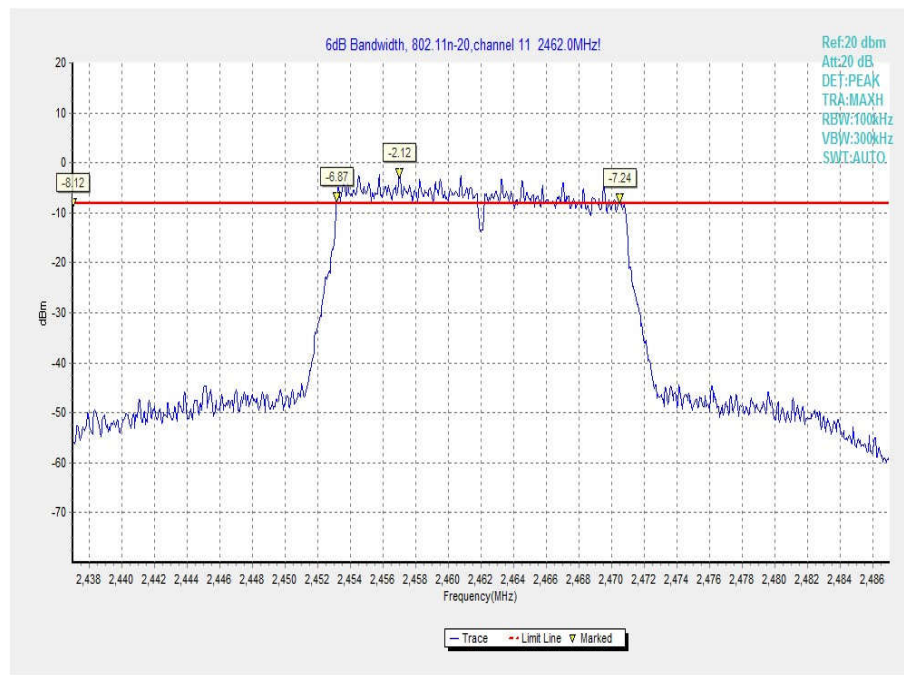
Fig.27 6dB Bandwidth (802.11 n-20MHz, Ch 11)
