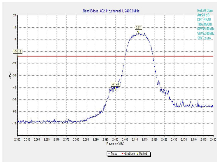
Fig.28 Band Edges (802.11b, Ch 1)
