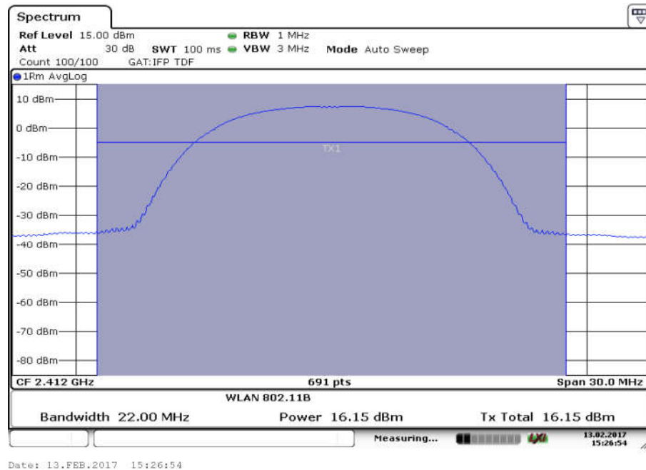
Fig.1 Maximum Average Output Power (802.11b, Ch 1, 5.5Mbps)
