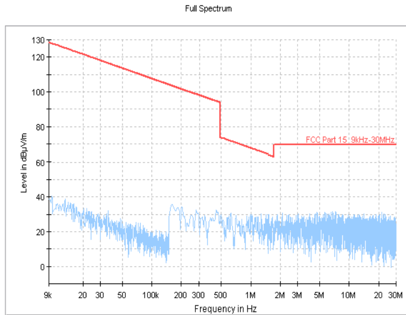
Fig.71 Radiated Spurious Emission (802.11g, Ch6, 9kHz-30MHz)
