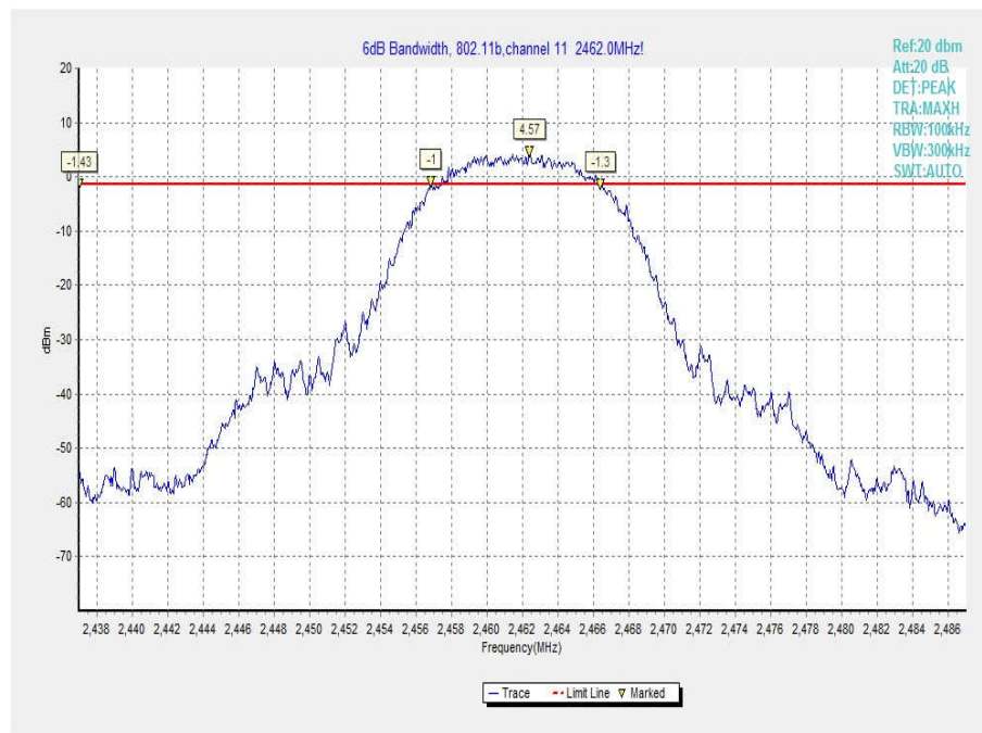
Fig.21 6dB Bandwidth (802.11b, Ch 11)
