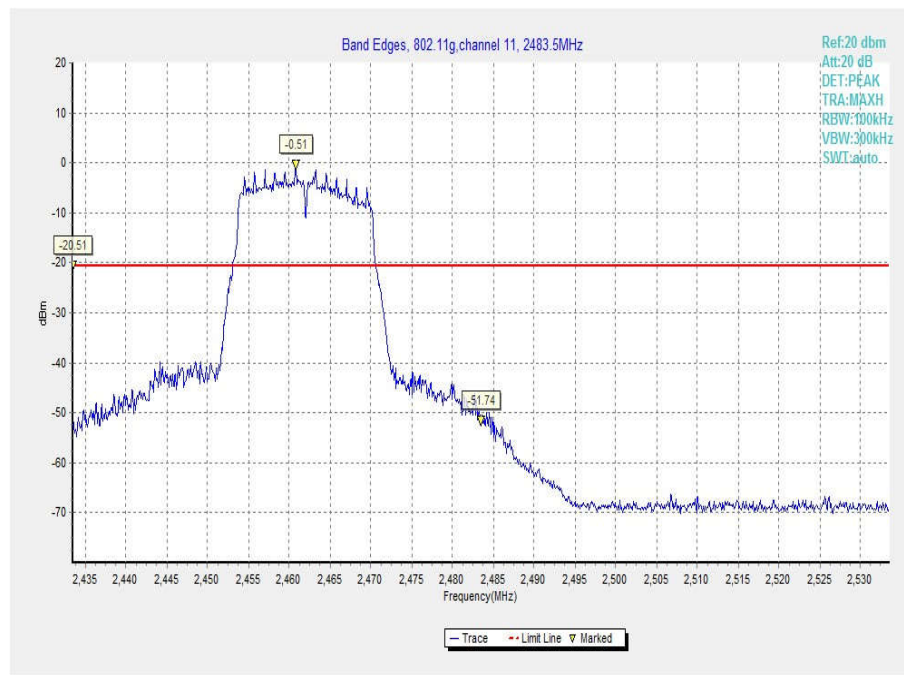
Fig.31 Band Edges (802.11g, Ch 11)
