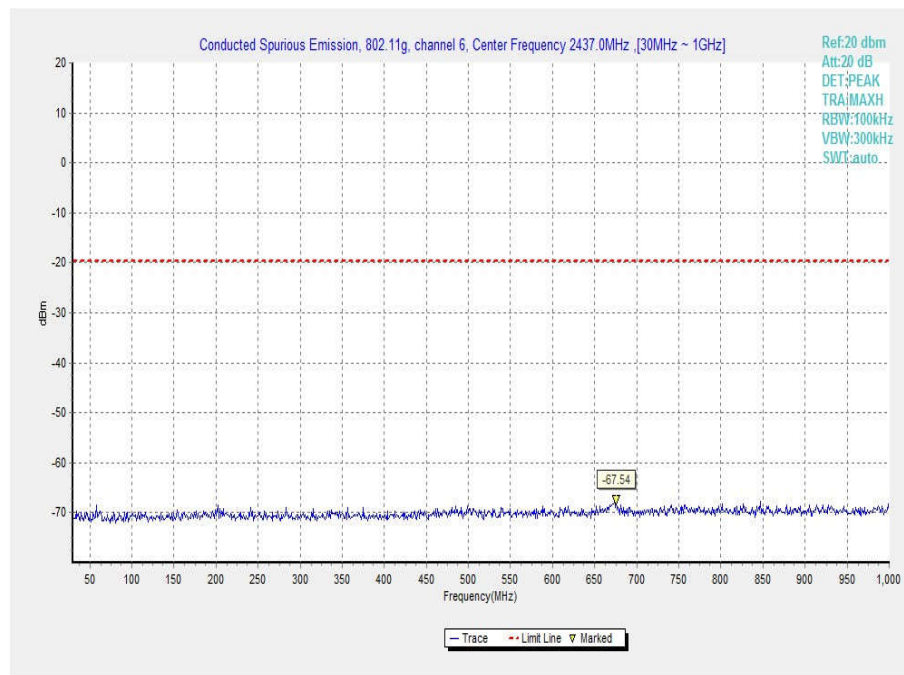
Fig.47 Conducted Spurious Emission (802.11g, Ch6, 30 MHz-1 GHz)
