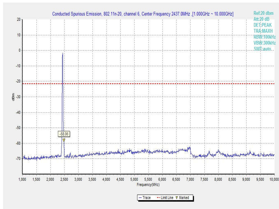
Fig.57 Conducted Spurious Emission (802.11n-20MHz, Ch6, 1 GHz-10 GHz)
