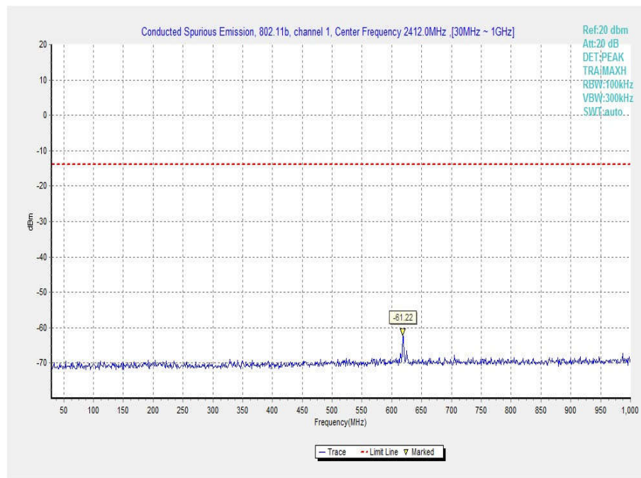
Fig.35 Conducted Spurious Emission (802.11b, Ch1, 30 MHz-1 GHz)
