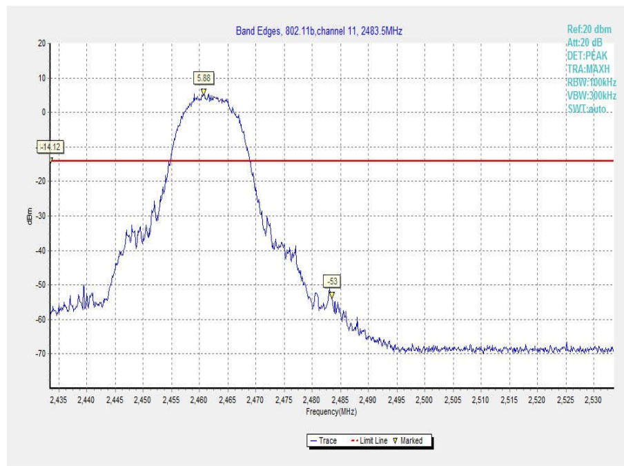
Fig.29 Band Edges (802.11b, Ch 11)
