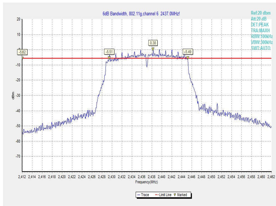
Fig.23 6dB Bandwidth (802.11g, Ch 6)
