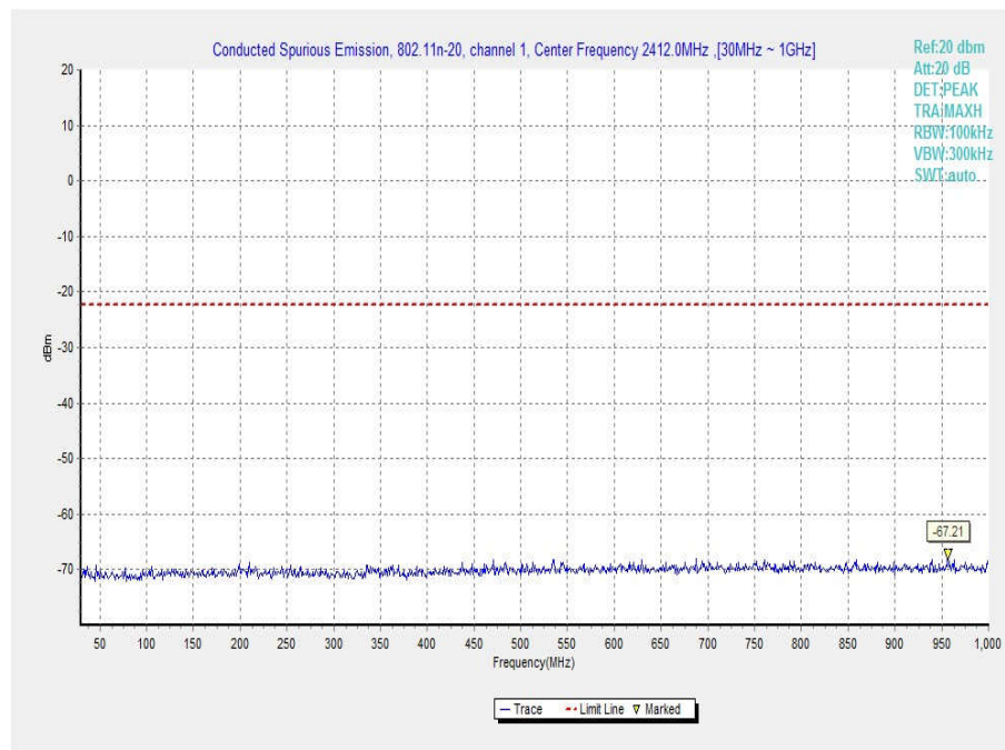
Fig.53 Conducted Spurious Emission (802.11n-20MHz, Ch1, 30 MHz-1 GHz)
