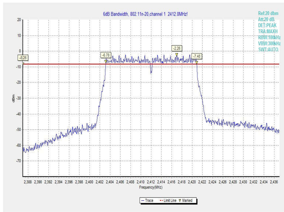
Fig.25 6dB Bandwidth (802.11 n-20MHz, Ch 1)
