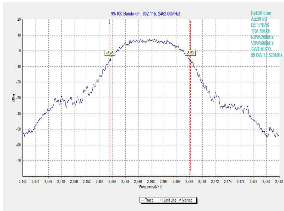
Fig.88 99% Occupied Bandwidth (802.11b, Ch 11)
