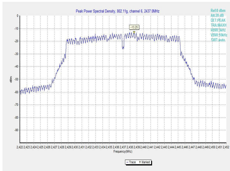
Fig.14 Power Spectral Density (802.11g, Ch 6)
