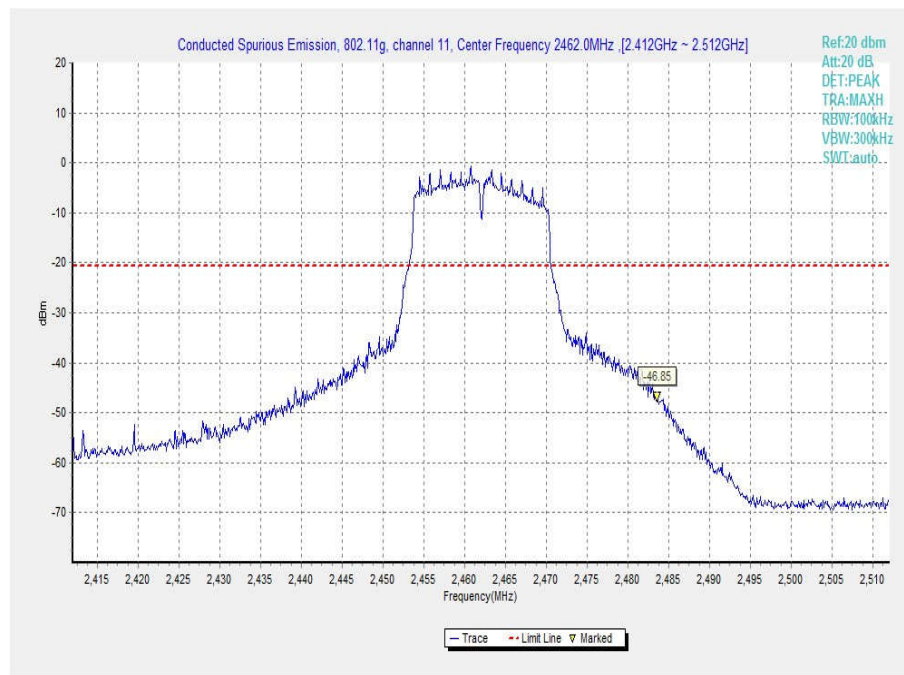
Fig.49 Conducted Spurious Emission (802.11g, Ch11, Center Frequency)
