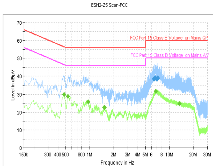
Fig.96 AC Power line Conducted Emission (Idle, AE1)
