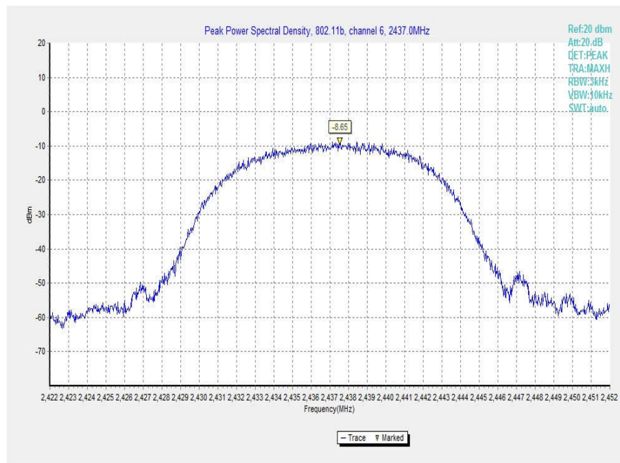
Fig.11 Power Spectral Density (802.11b, Ch 6)
