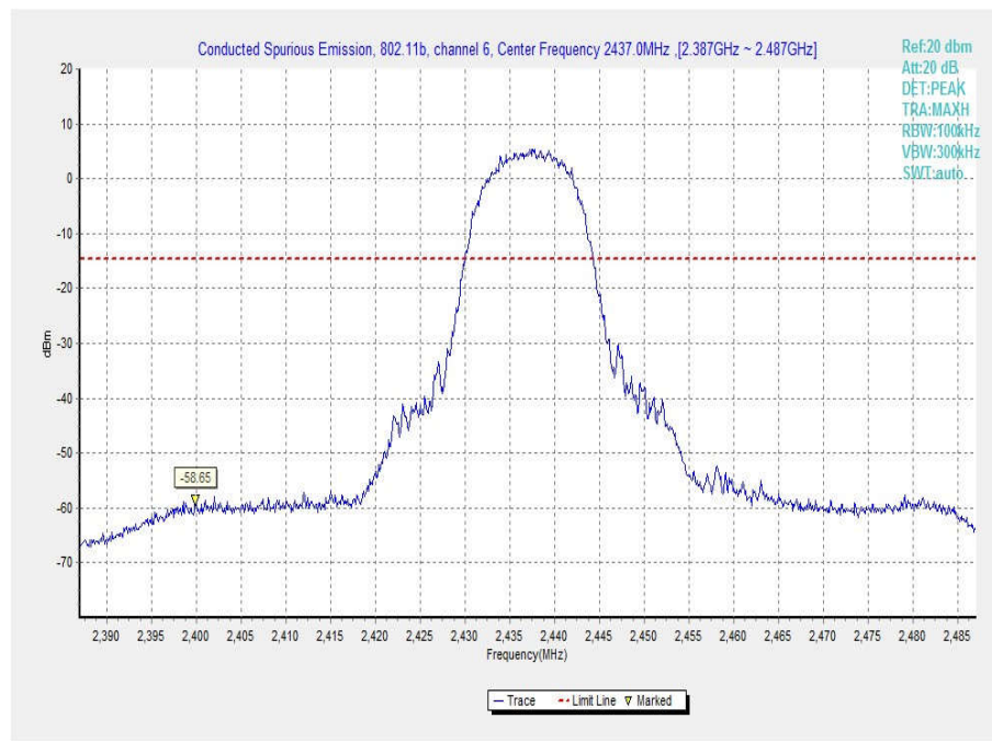
Fig.37 Conducted Spurious Emission (802.11b, Ch6, Center Frequency)
