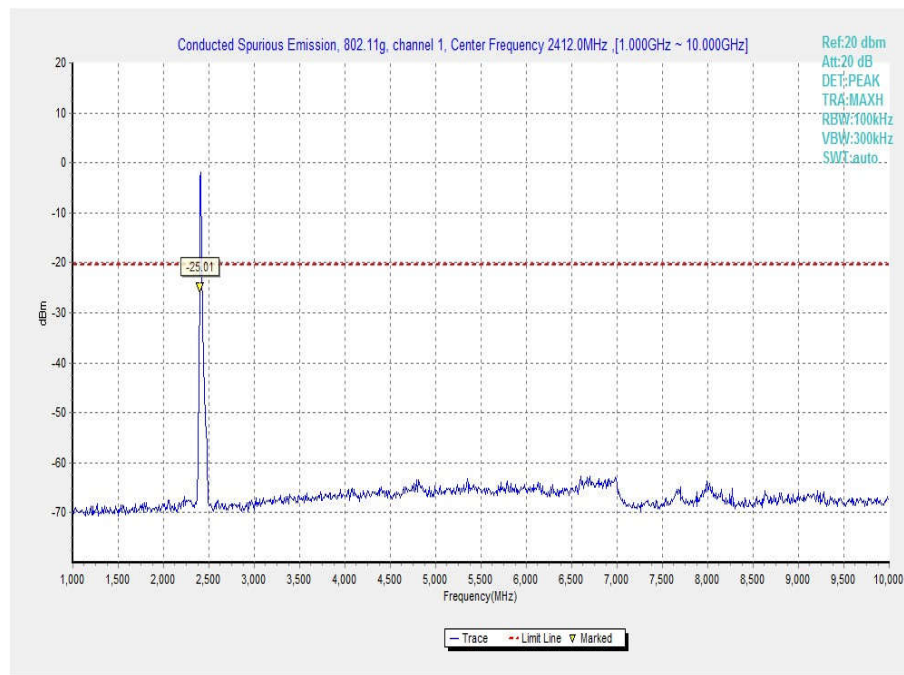
Fig.45 Conducted Spurious Emission (802.11g, Ch1, 1 GHz-10 GHz)
