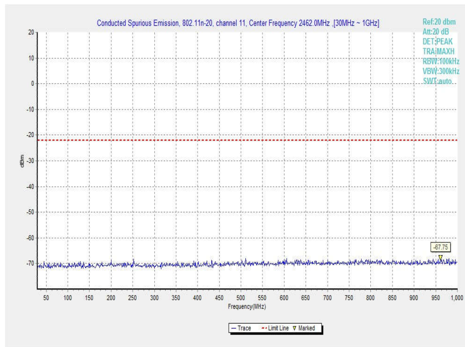
Fig.59 Conducted Spurious Emission (802.11n-20MHz, Ch11, 30 MHz-1 GHz)
