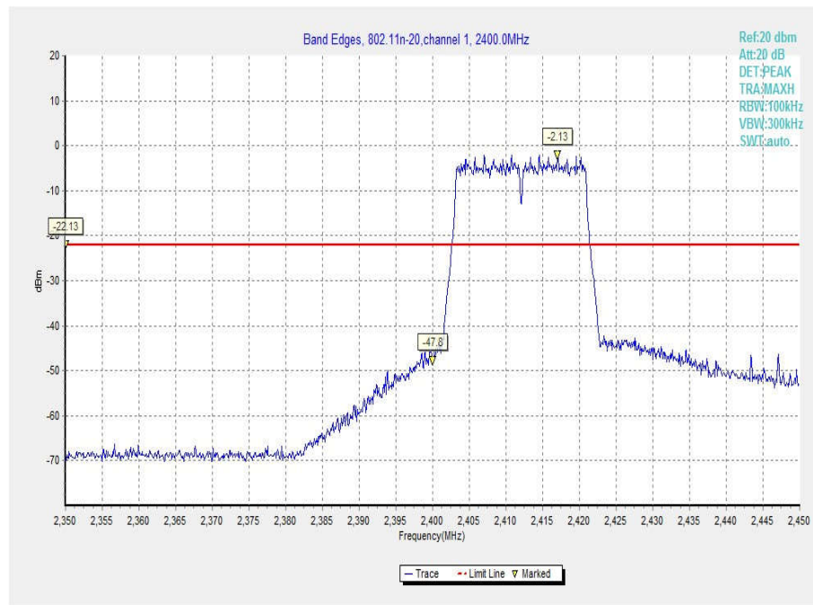
Fig.32 Band Edges (802.11 n-20MHz, Ch 1)
