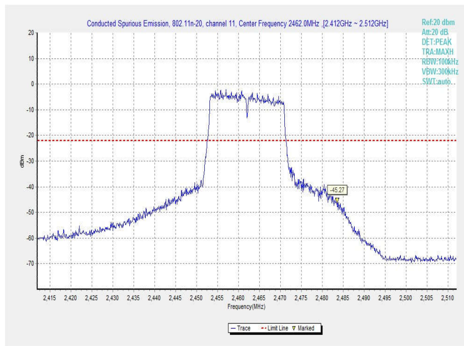
Fig.58 Conducted Spurious Emission (802.11n-20MHz, Ch11, Center Frequency)
