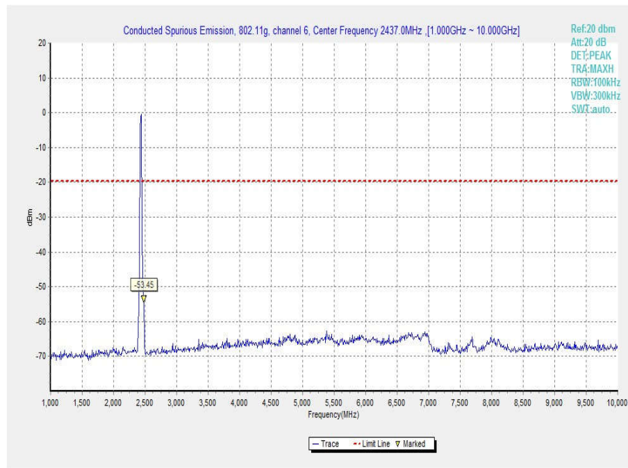
Fig.48 Conducted Spurious Emission (802.11g, Ch6, 1 GHz-10 GHz)
