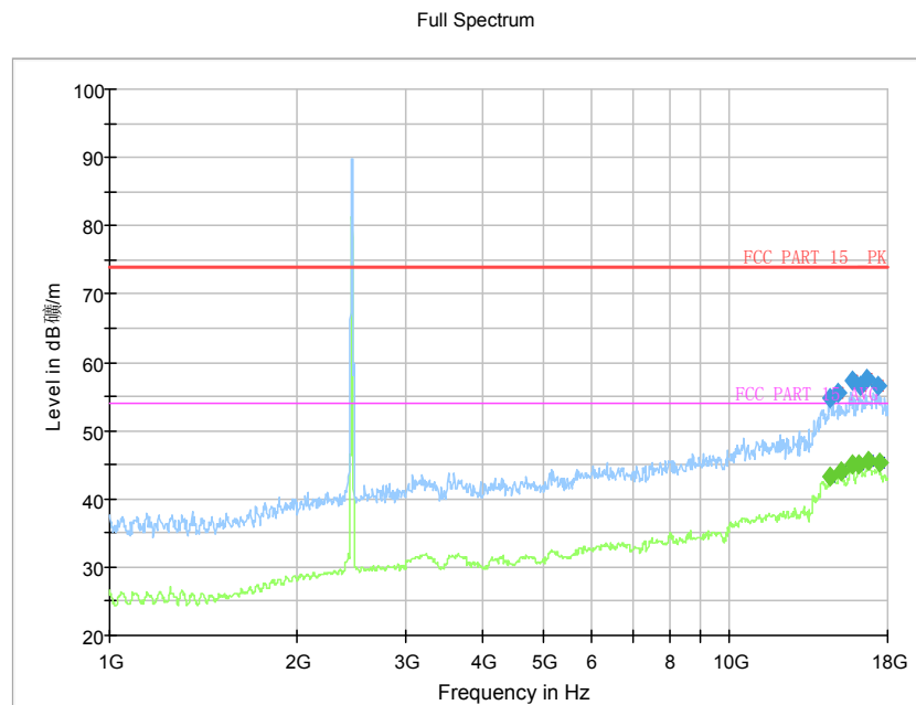
Fig.83 Radiated Spurious Emission (802.11n-20MHz, Ch11, 1 GHz-18 GHz)
