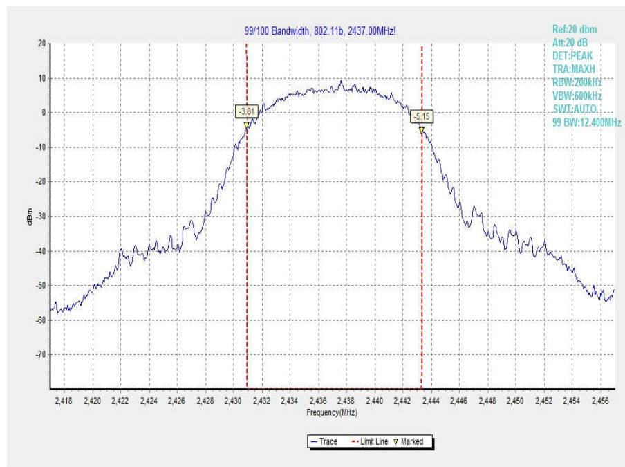
Fig.87 99% Occupied Bandwidth (802.11b, Ch 6)
