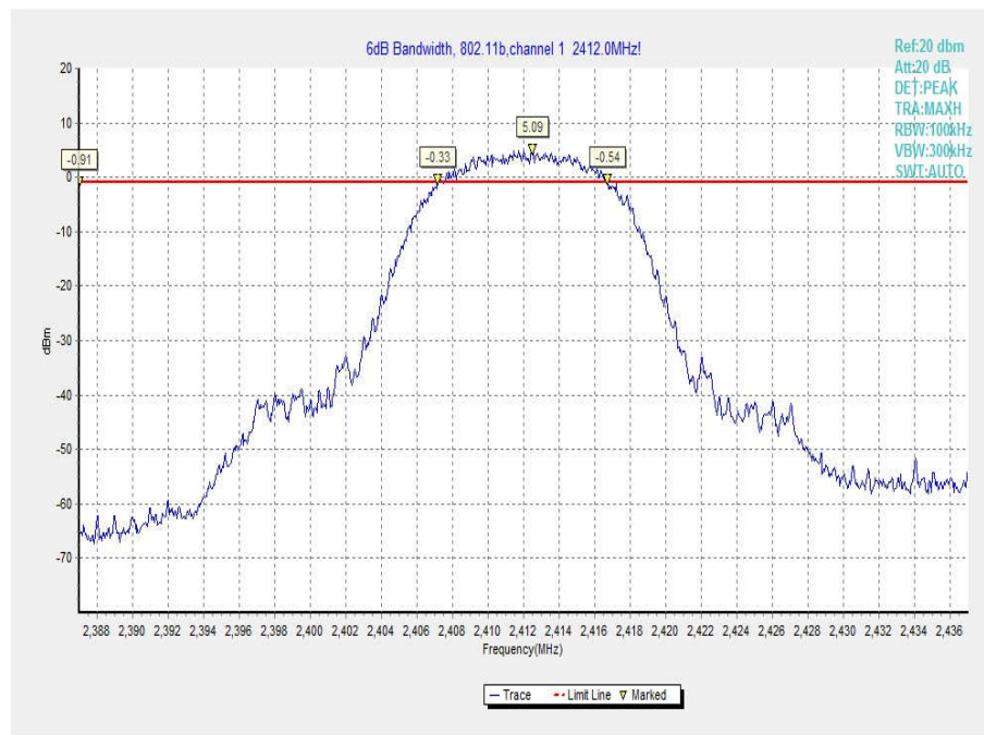
Fig.19 6dB Bandwidth (802.11b, Ch 1)
