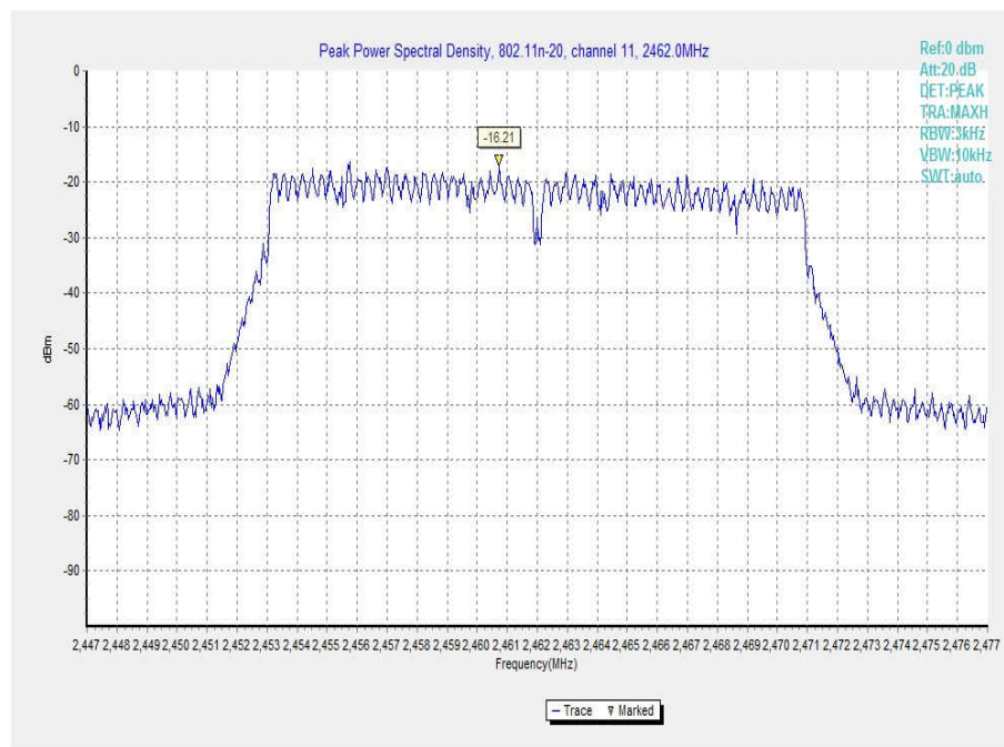
Fig.18 Power Spectral Density (802.11n-20MHz, Ch 11)
