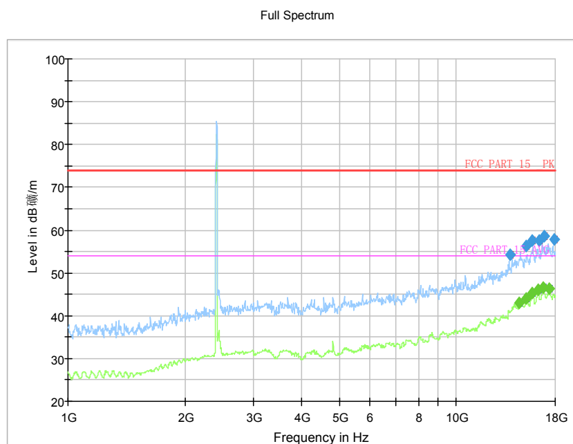
Fig.62 Radiated Spurious Emission (802.11b, Ch1, 1 GHz-18GHz)
