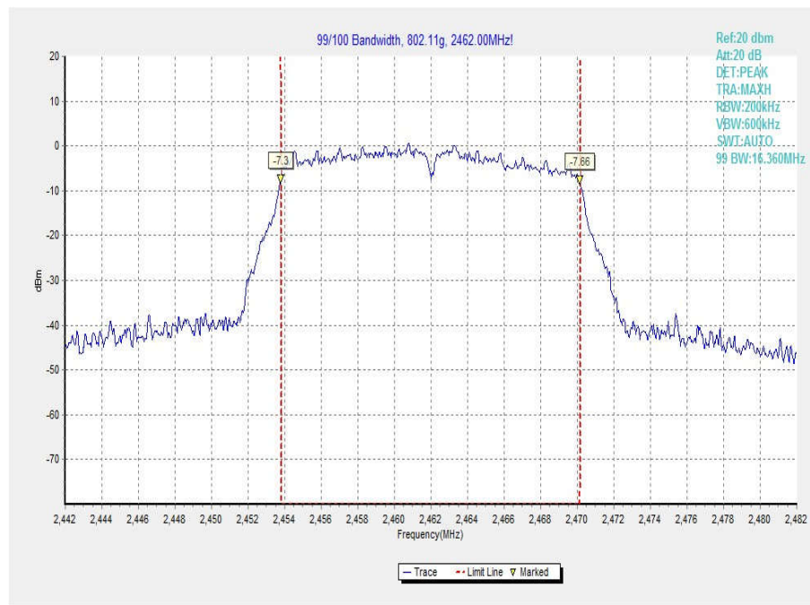
Fig.91 99% Occupied Bandwidth (802.11g, Ch 11)
