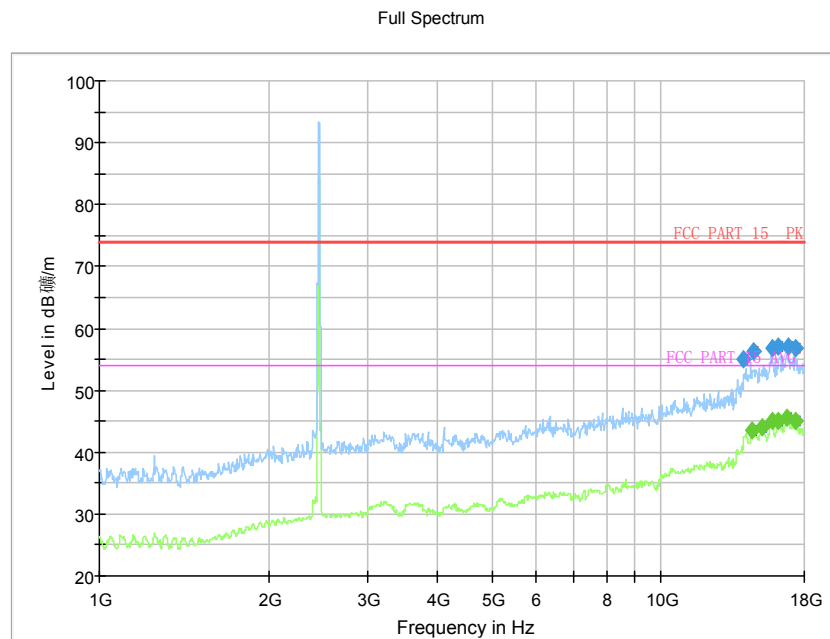
Fig.75 Radiated Spurious Emission (802.11g, Ch11, 1 GHz-18 GHz)
