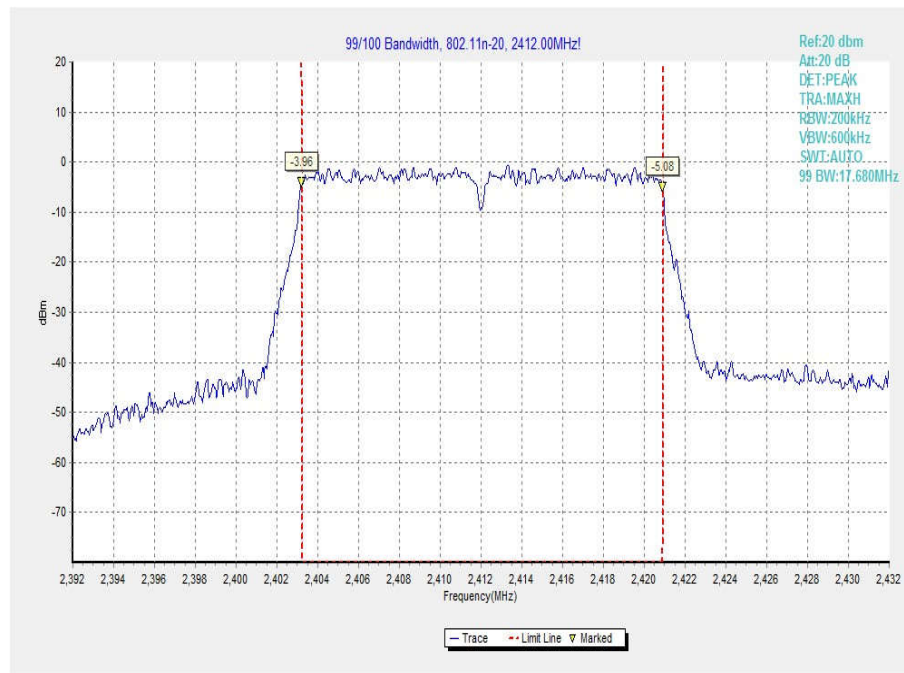
Fig.92 99% Occupied Bandwidth (802.11n-20MHz, Ch 1)
