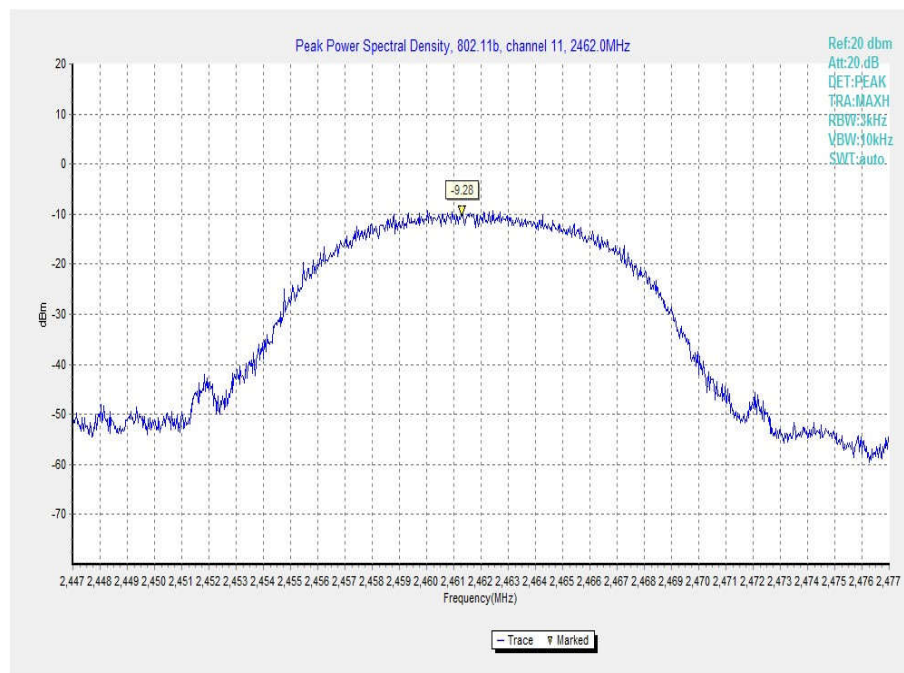
Fig.12 Power Spectral Density (802.11b, Ch 11)
