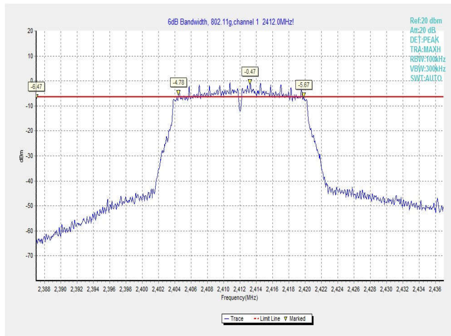
Fig.22 6dB Bandwidth (802.11g, Ch 1)
