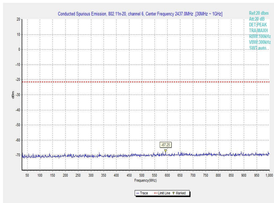
Fig.56 Conducted Spurious Emission (802.11n-20MHz, Ch6, 30 MHz-1 GHz)
