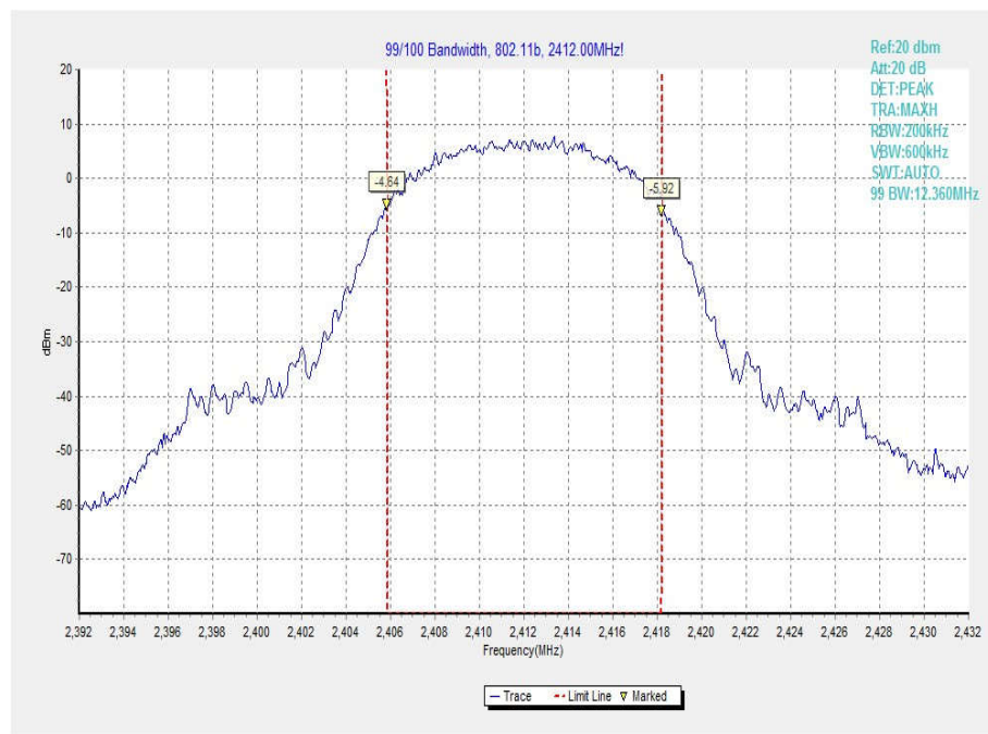
Fig.86 99% Occupied Bandwidth (802.11b, Ch 1)
