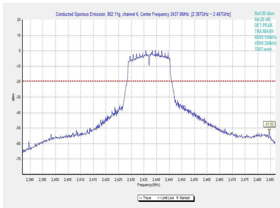
Fig.46 Conducted Spurious Emission (802.11g, Ch6, Center Frequency)
