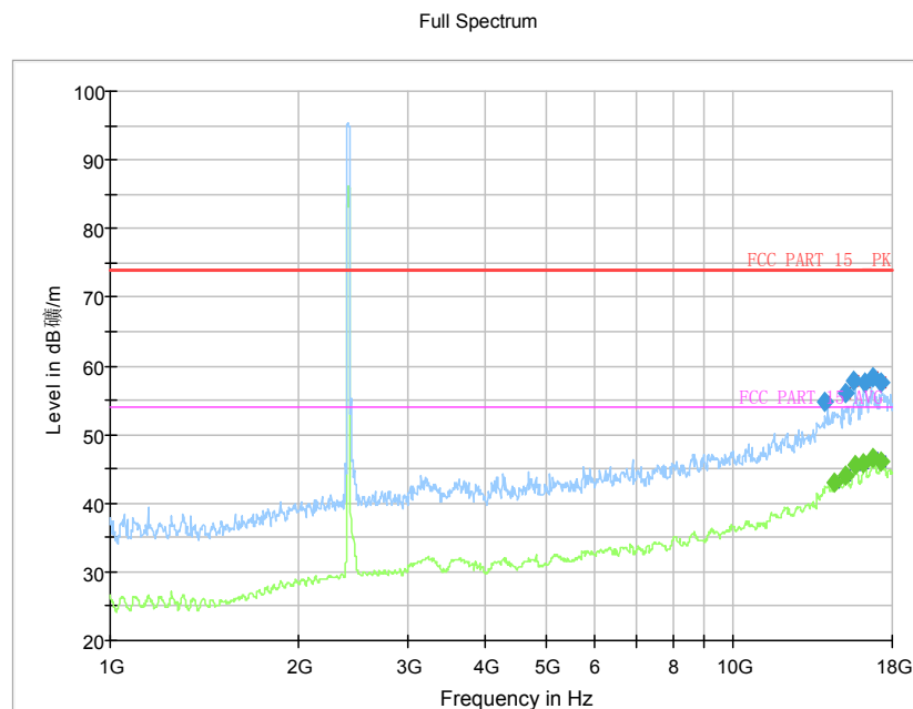
Fig.78 Radiated Spurious Emission (802.11n-20MHz, Ch1, 1 GHz-18 GHz)
