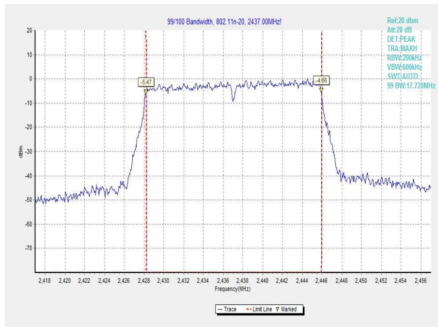
Fig.93 99% Occupied Bandwidth (802.11n-20MHz, Ch 6)
