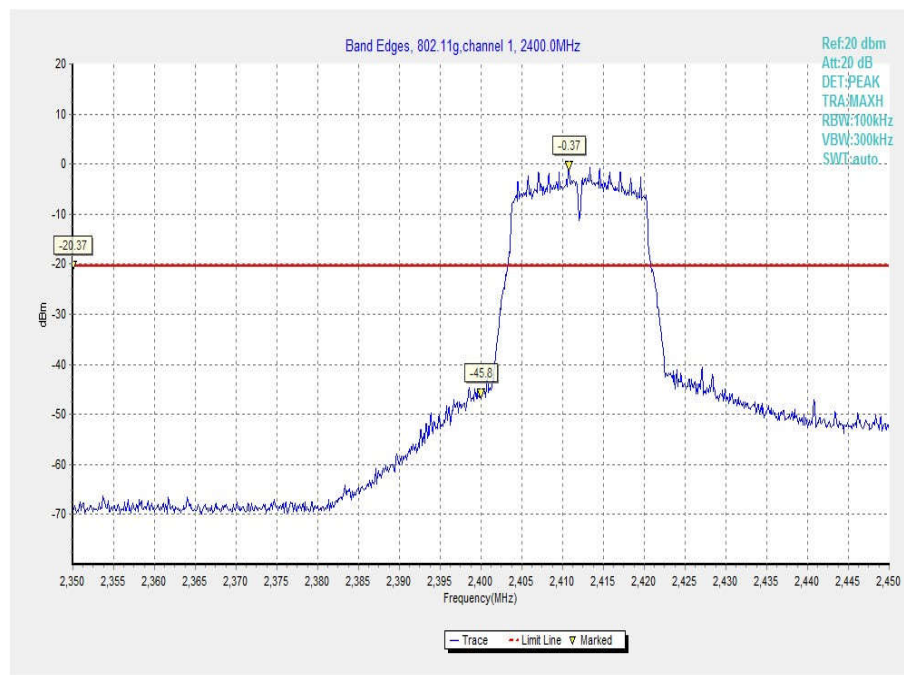
Fig.30 Band Edges (802.11g, Ch 1)
