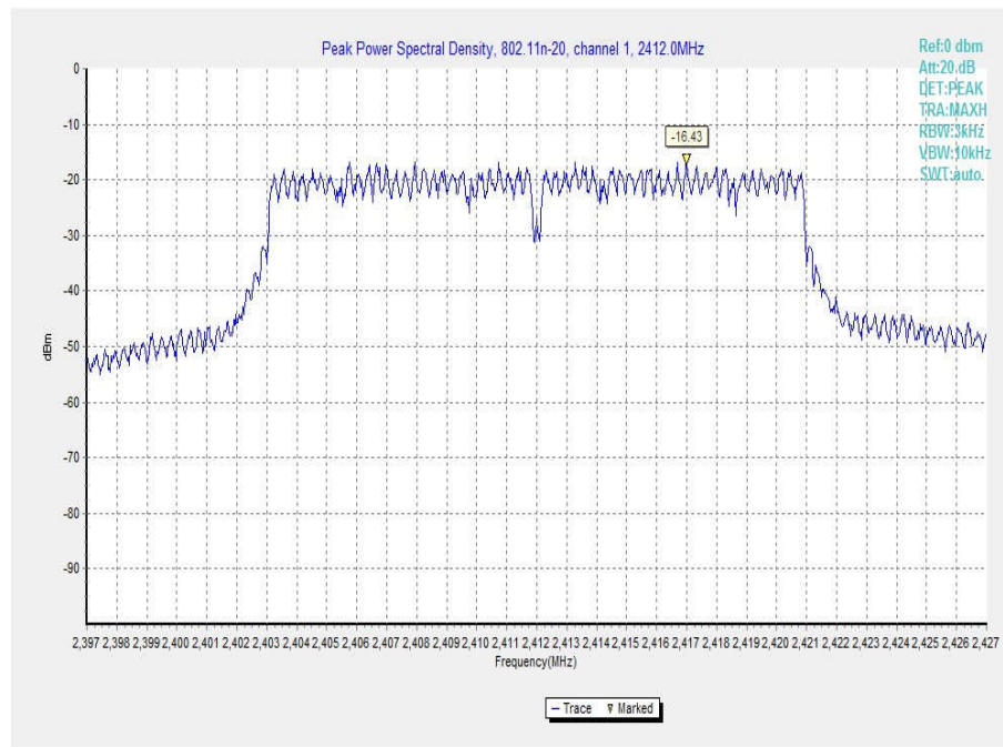
Fig.16 Power Spectral Density (802.11n-20MHz, Ch 1)
