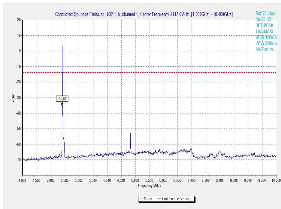
Fig.36 Conducted Spurious Emission (802.11b, Ch1, 1 GHz-10 GHz)
