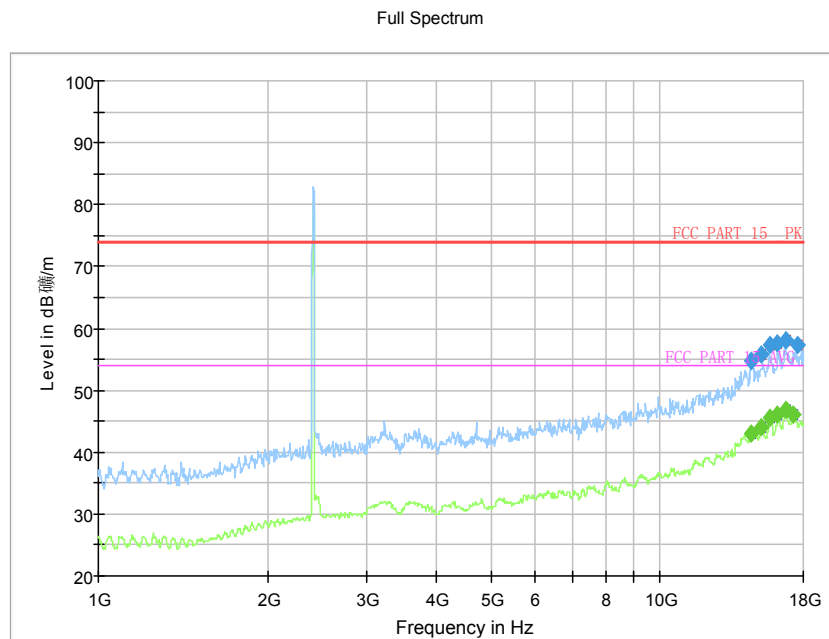
Fig.65 Radiated Spurious Emission (802.11b, Ch6, 1 GHz-18GHz)
