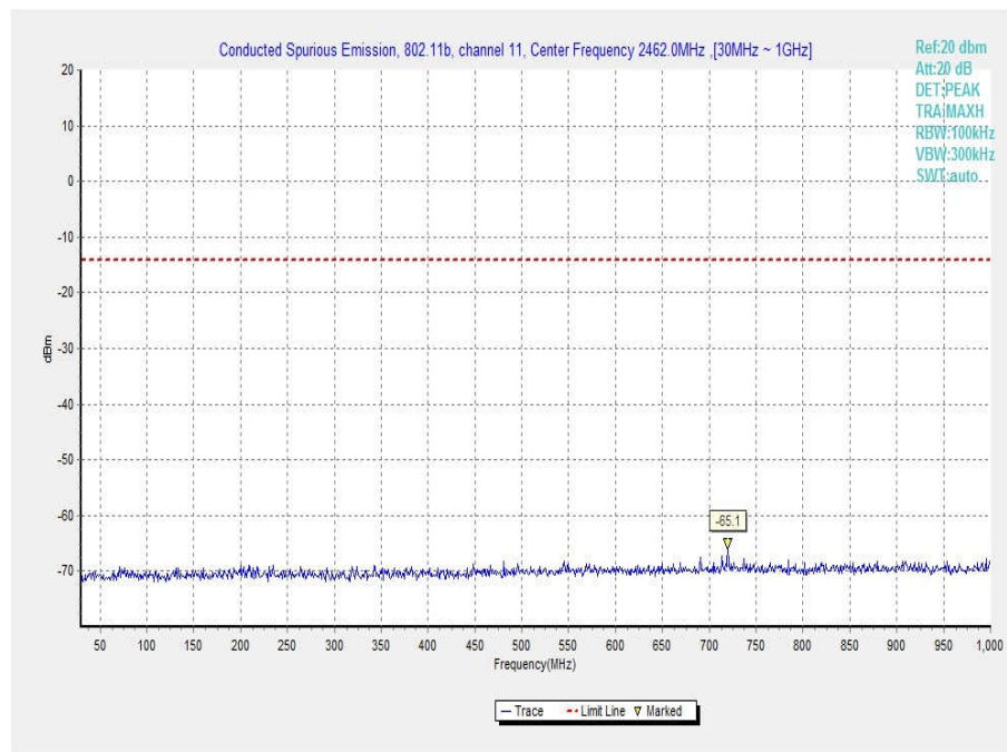
Fig.41 Conducted Spurious Emission (802.11b, Ch11, 30 MHz-1 GHz)
