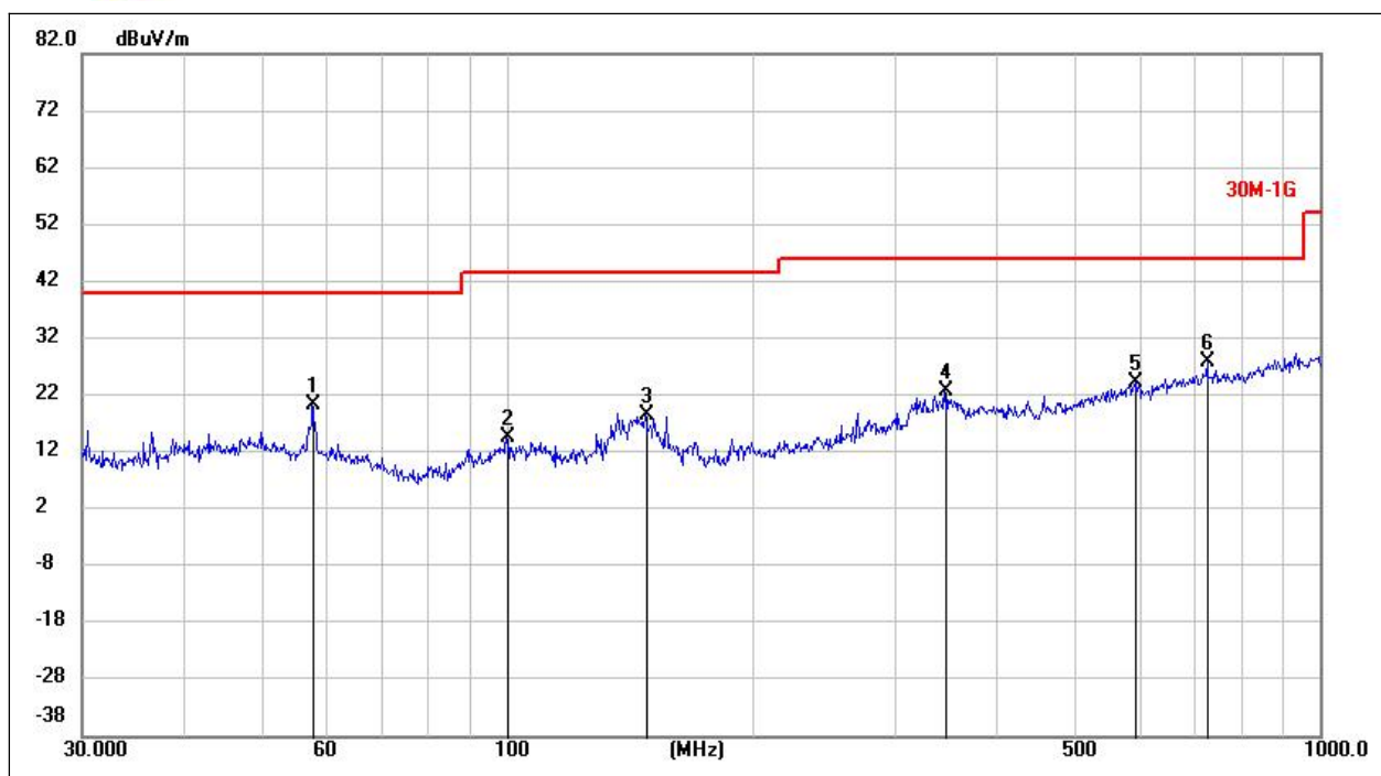
( \pi/4 -DQPSK_2480MHz, Antenna Horizontal, 30MHz to 1GHz)
