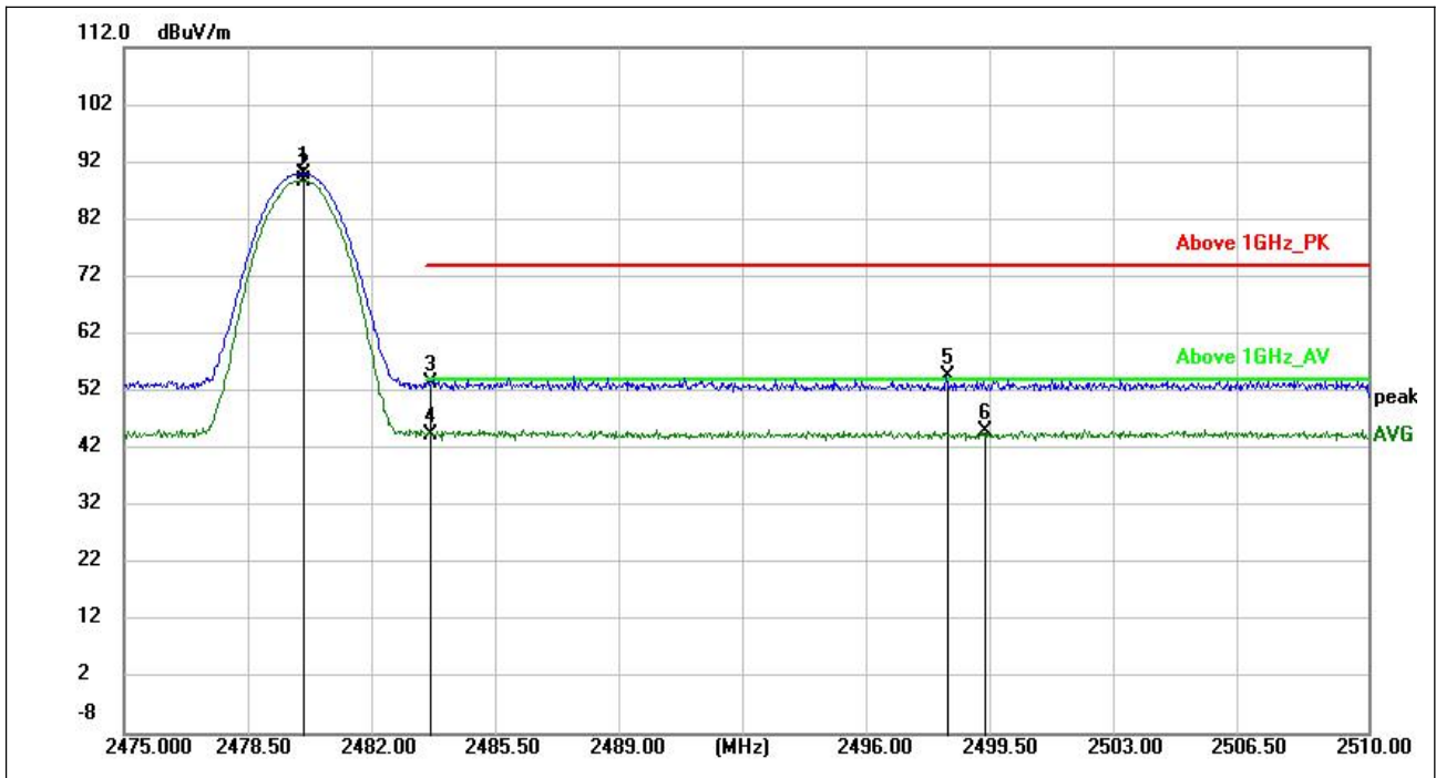
(3DH5_2480MHz, Antenna Vertical)
