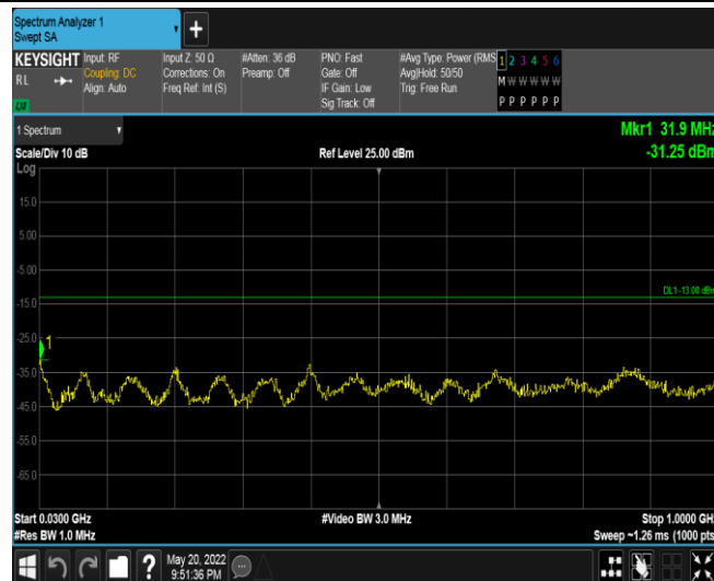
Band66-5MHz-16QAM-132647-1RB#0-Range2:30~1000MHz
