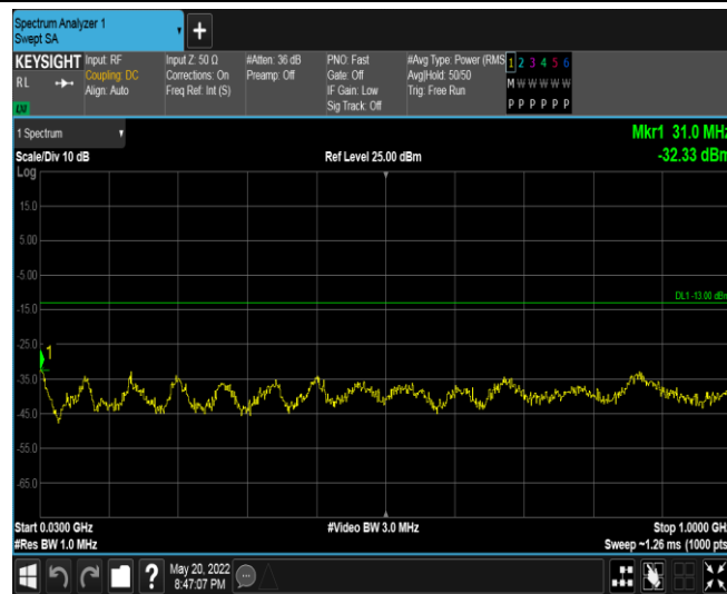
Band66-1.4MHz-QPSK-131979-1RB#0-Range1:30~1000MHz
