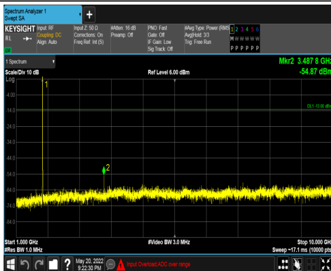
Band66-3MHz-16QAM-132322-1RB#0-Range3:1000~10000MHz
