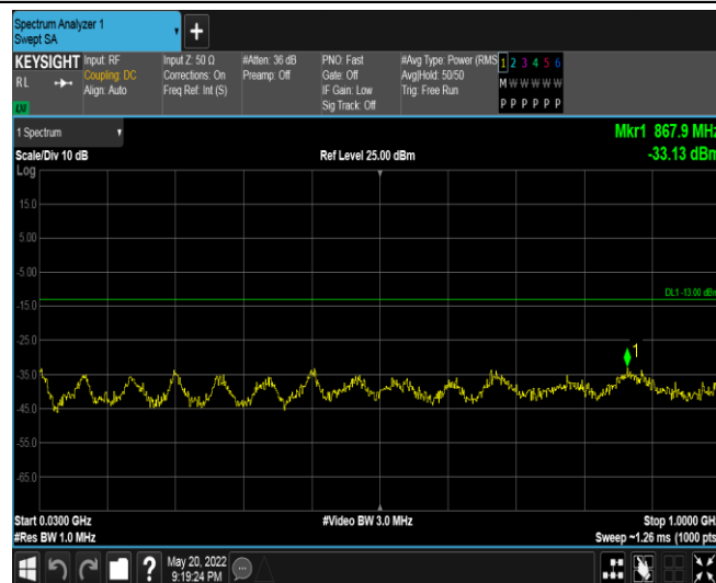
Band66-3MHz-16QAM-131987-1RB#0-Range1:30~1000MHz
