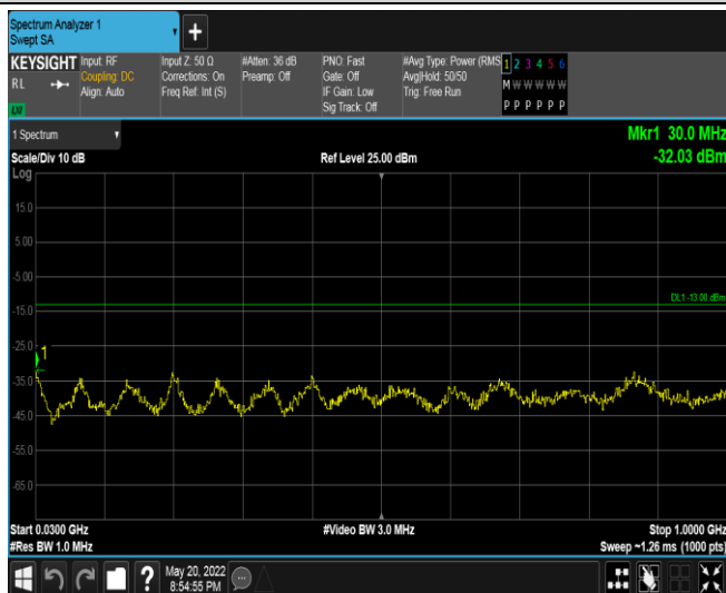
Band66-1.4MHz-QPSK-132665-1RB#0-Range2:30~1000MHz
