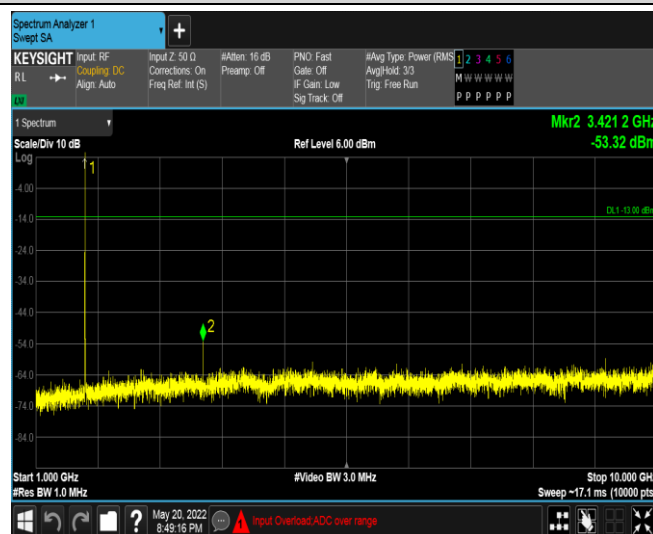
Band66-1.4MHz-QPSK-131979-1RB#0-Range3:1000~10000MHz
