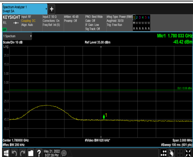
Band66-10MHz-QPSK-132622-1RB#0
