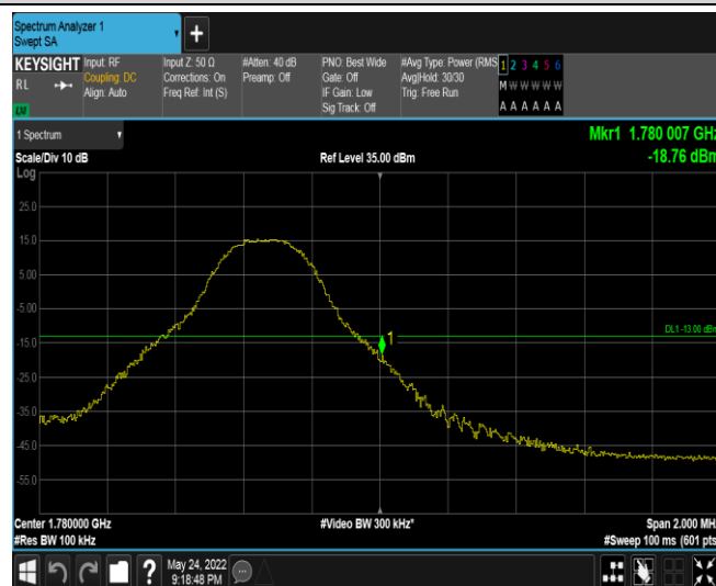
Band66-5MHz-16QAM-132647-1RB#24
