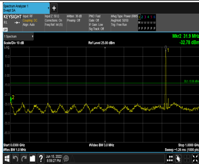
Band26-15MHz-16QAM-26865-1RB#0-Range2:30~1000MHz
