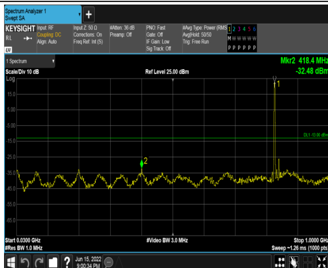
Band26-15MHz-QPSK-26915-1RB#0-Range2:30~1000MHz
