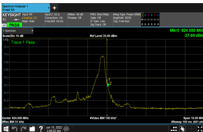
Band26-3MHz-16QAM-26775-15RB#0
