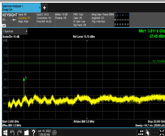
Band25-10MHz-QPSK-26640-1RB#0-Range3:2000~20000MHz
