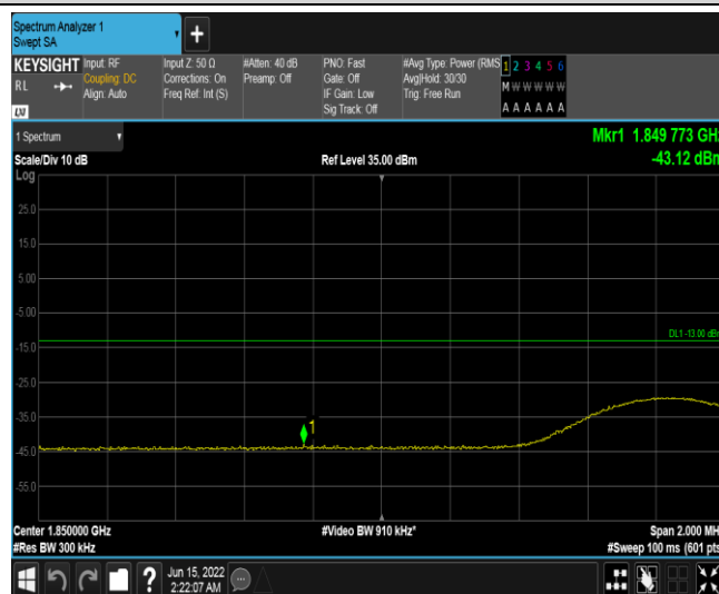
Band25-15MHz-QPSK-26115-1RB#74
