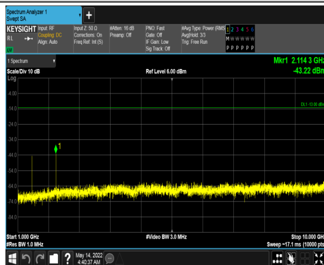
Band17-10MHz-16QAM-23780-1RB#0-Range3:1000~10000MHz
