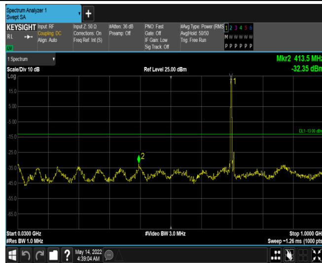
Band17-10MHz-16QAM-23780-1RB#0-Range2:30~1000MHz
