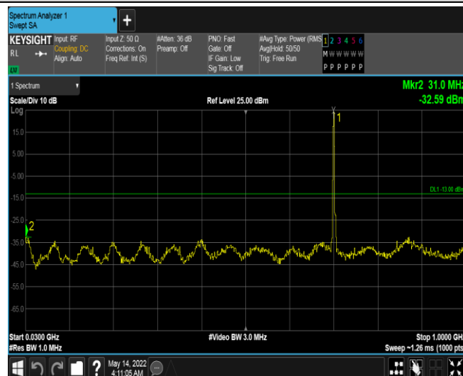
Band17-5MHz-QPSK-23790-1RB#0-Range2:30~1000MHz
