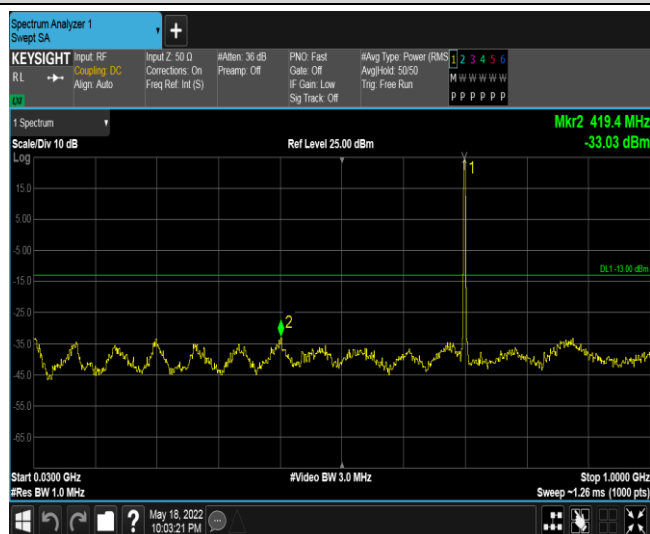
Band12-1.4MHz-QPSK-23095-1RB#0-Range2:30~1000MHz
