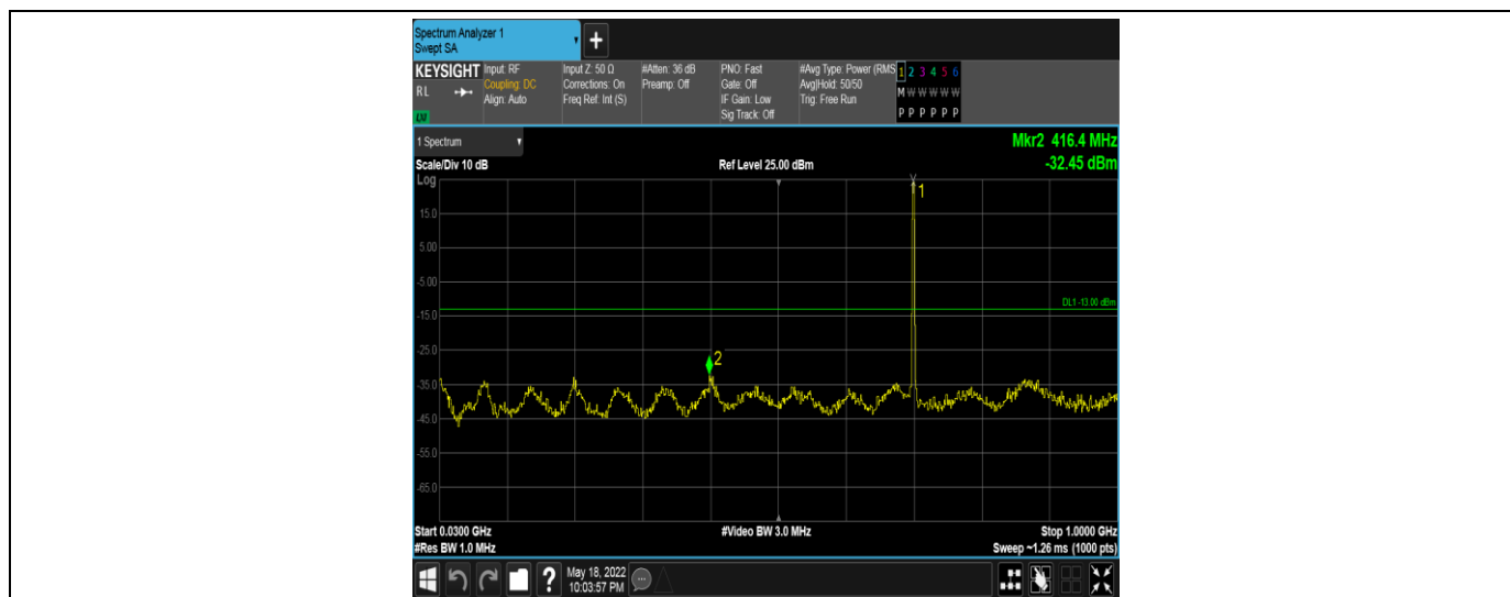
Band12-1.4MHz-16QAM-23095-1RB#0-Range2:30~1000MHz
