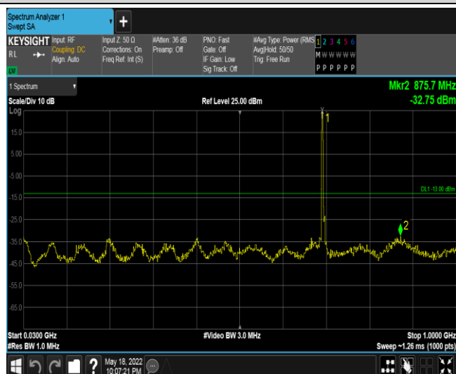
Band12-3MHz-QPSK-23025-1RB#0-Range2:30~1000MHz
