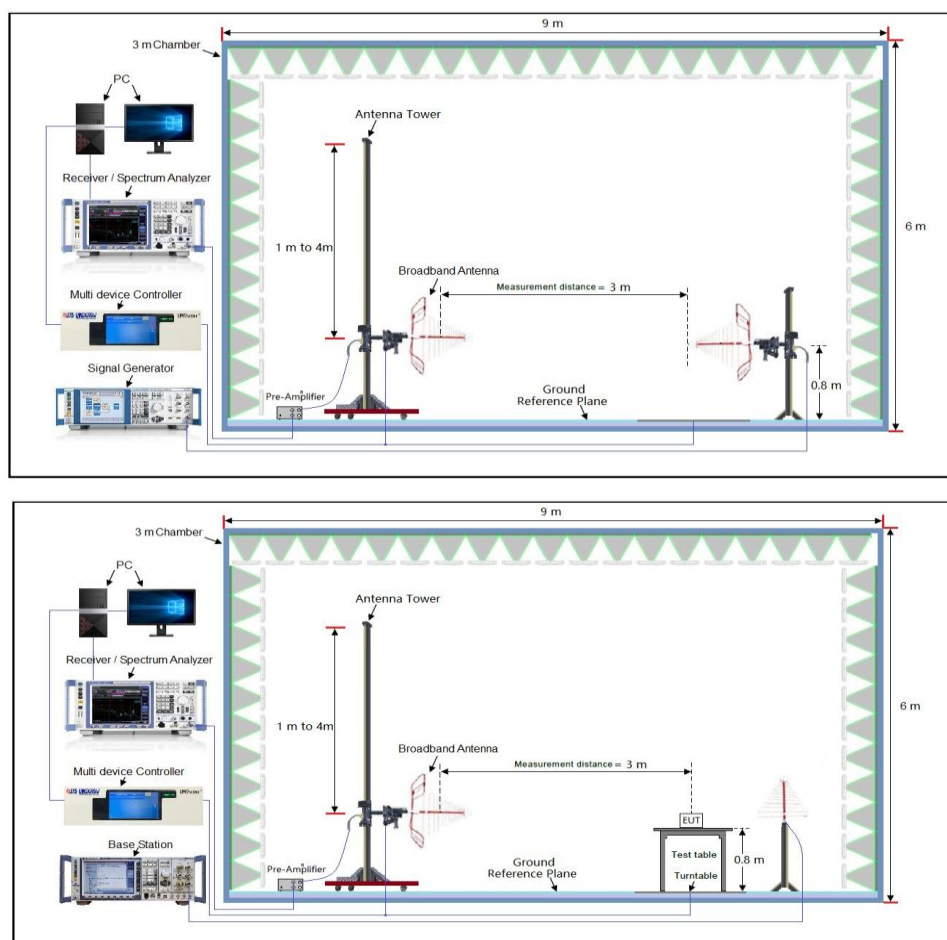
Radiated Power 30MHz to 1GHz Test setup
