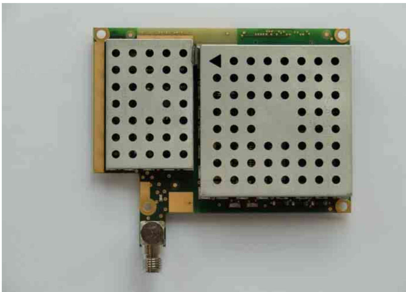
RF Board top and bottom (see next page for view with shield removed)
