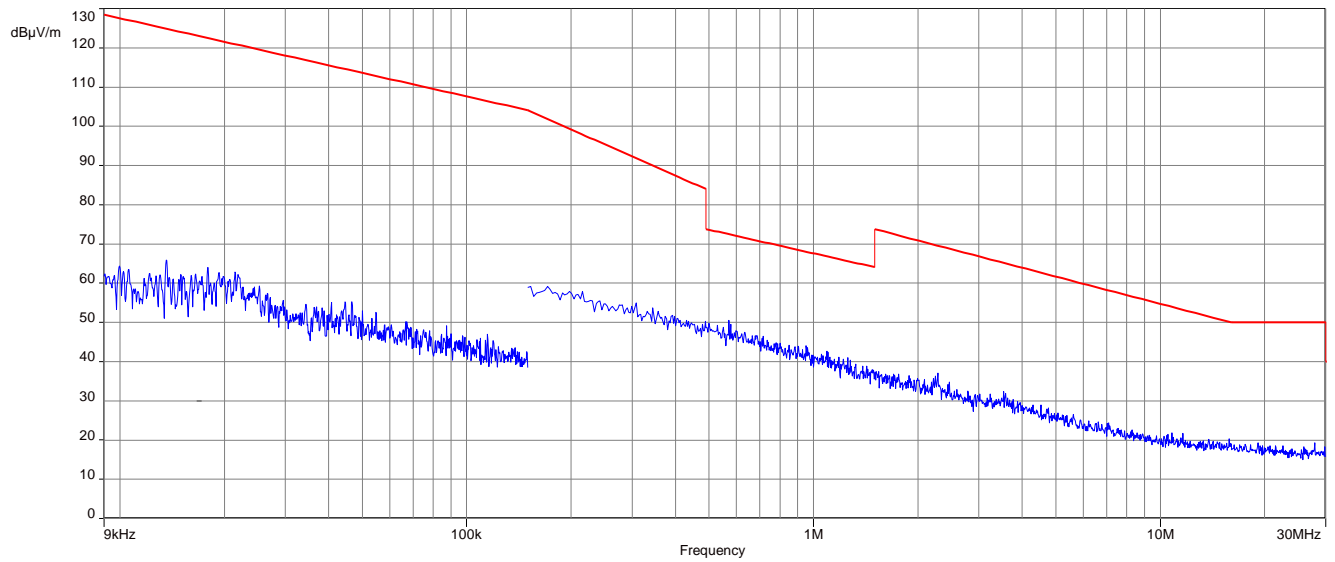
Plot 1: TX-Mode 902.4 MHz
