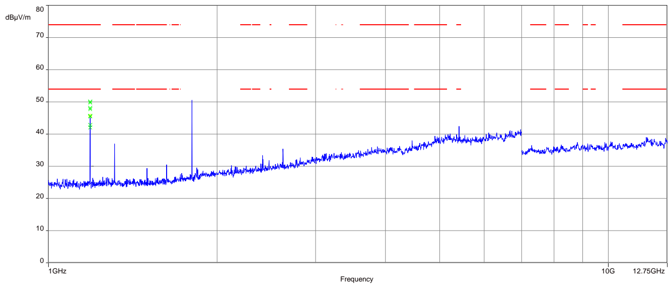
Plot 1: 1 GHz – 12.75 GHz, horizontal &amp; vertical polarisation 902.4 MHz
