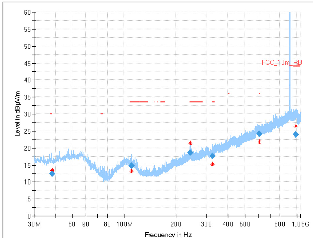
Plot 2: 30 MHz – 1 GHz, horizontal &amp; vertical polarisation 912.0 MHz
