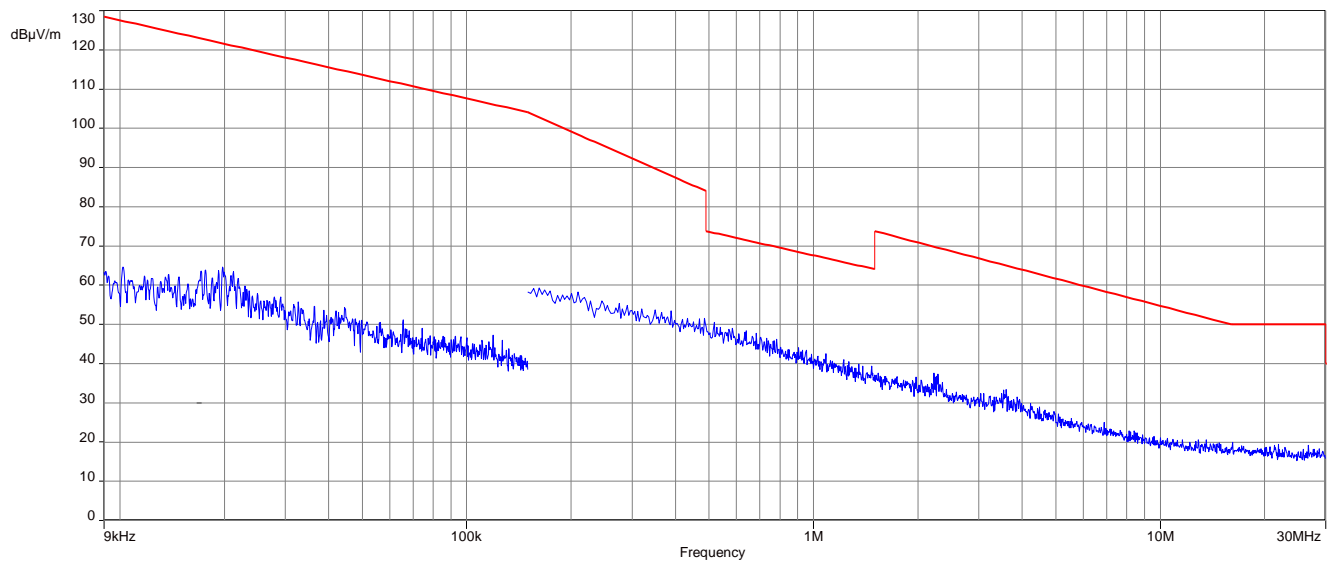
Plot 3: TX-Mode 922.0 MHz
