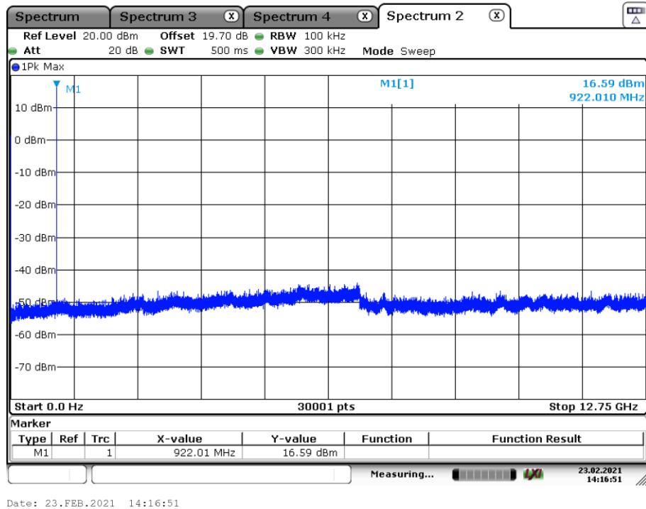
Plot 3: 922.0 MHz, 9 kHz – 12.75 GHz
