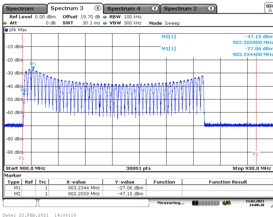
Plot 1: 20 dB – hopping on, lower bandedge
