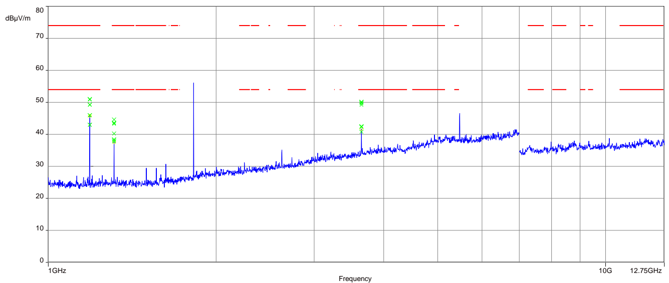
Plot 2: 1 GHz – 12.75 GHz, horizontal &amp; vertical polarisation 912.0 MHz
