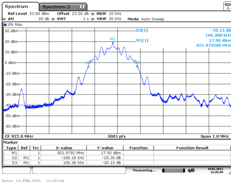
Plot 5: 922.0MHz, 20 dB-BW
