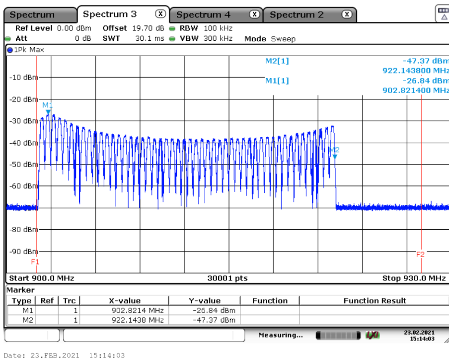
Plot 1: 20 dB – hopping on, upper bandedge
