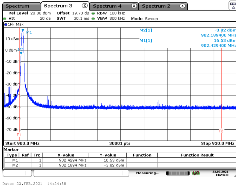
Plot 3: 20 dB – hopping off, lowest channel lower bandedge
