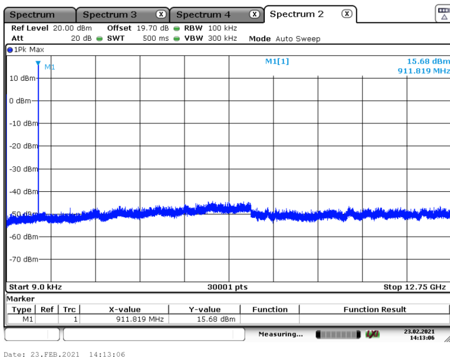
Plot 2: 912.0 MHz, 9 kHz – 12.75 GHz
