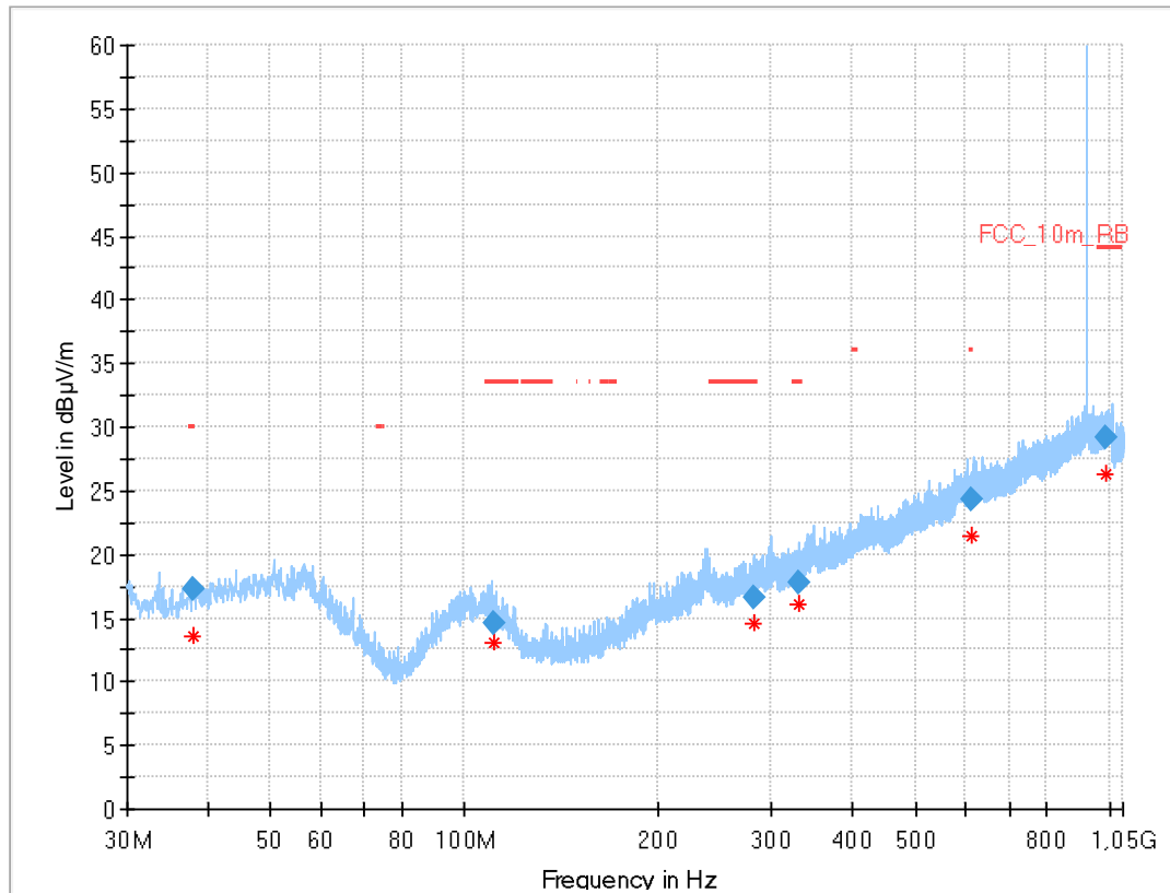
Plot 3: 30 MHz – 1 GHz, horizontal &amp; vertical polarisation 922.0 MHz
