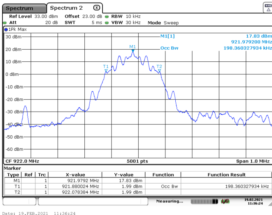
Plot 6: 922.0 MHz, 99%OBW
