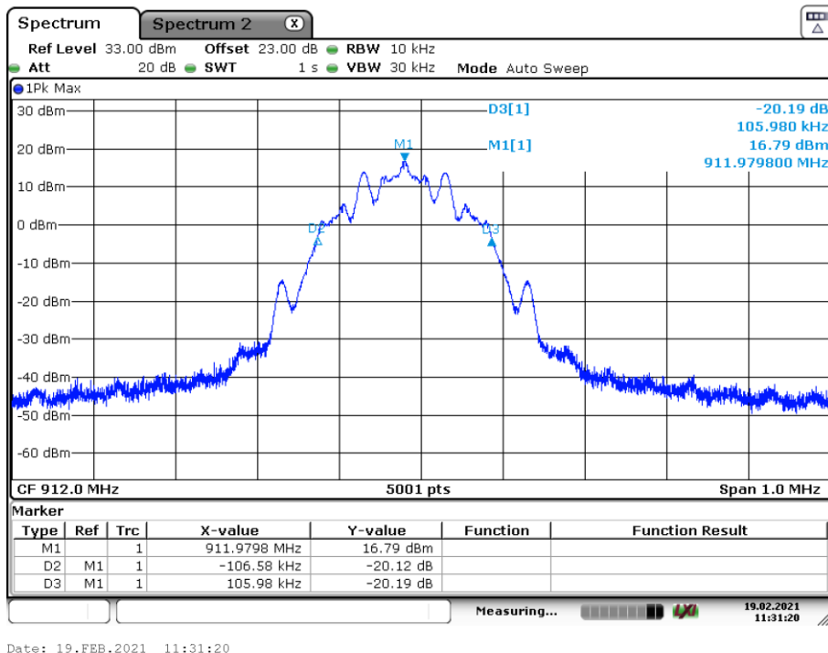
Plot 3: 912.0 MHz, 20 dB-BW
