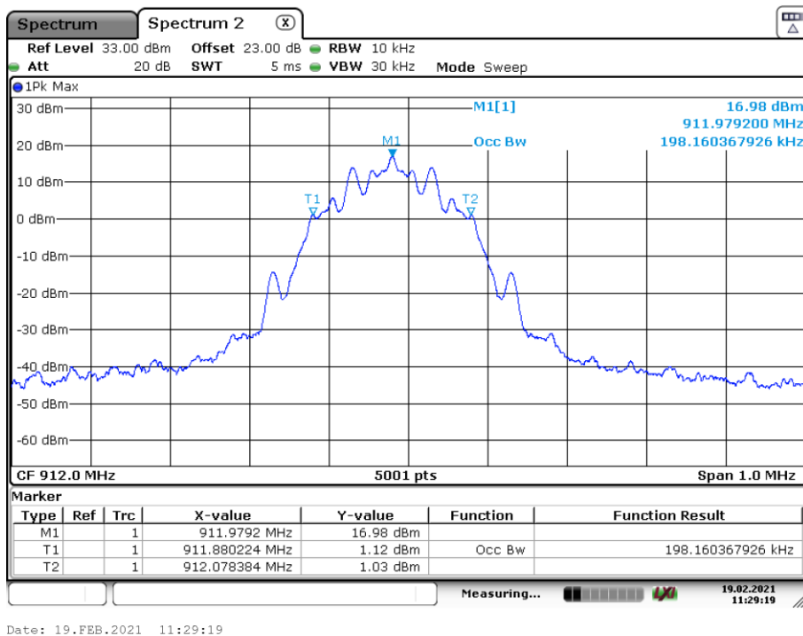
Plot 4: 912.0 MHz, 99%OBW
