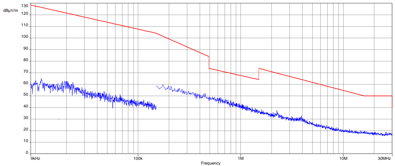
Plot 2: TX-Mode 912.0 MHz
