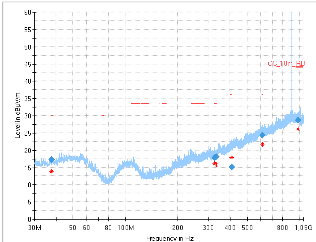
Plot 1: 30 MHz – 1 GHz, horizontal &amp; vertical polarisation 902.4 MHz
