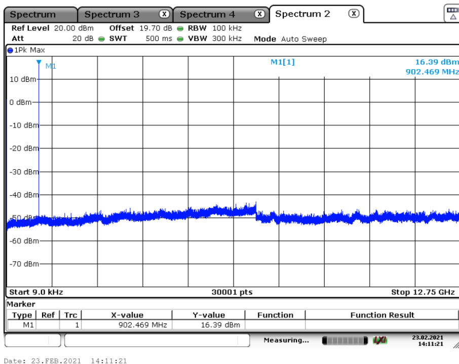
Plot 1: 902.40 MHz, 9 kHz – 12.75 GHz
