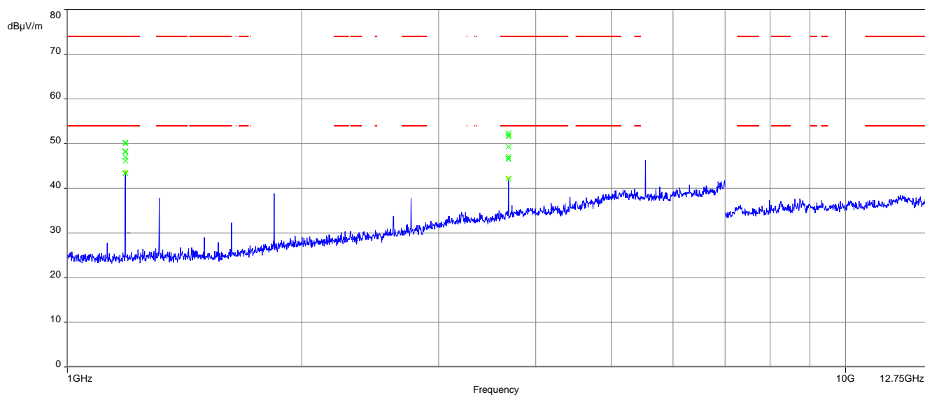
Plot 3: 1 GHz – 12.75 GHz, horizontal & vertical polarisation 922.0 MHz
