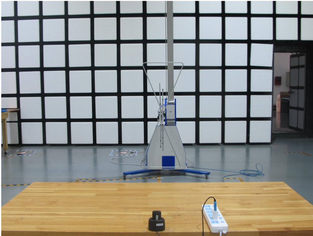
RE_30MHz-1GHz
