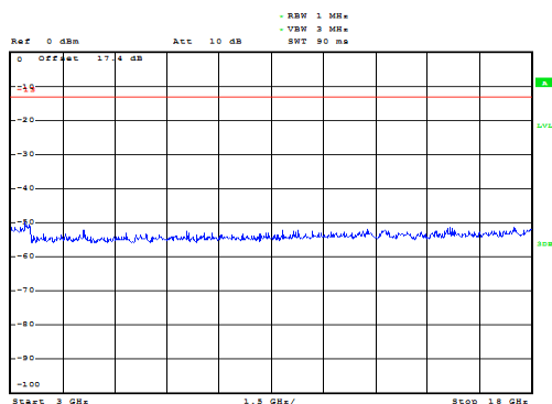
LTE Band 4 1.4MHz CH-Low 3GHz~18GHz
