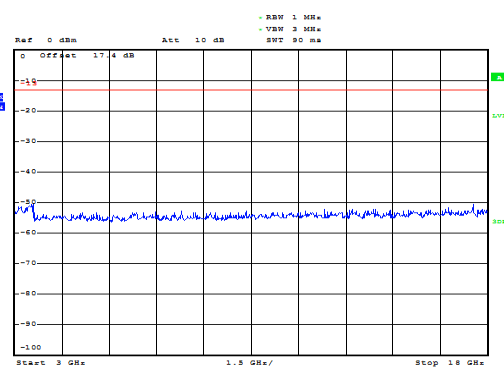
LTE Band 4 1.4MHz CH-Middle 3GHz~18GHz
