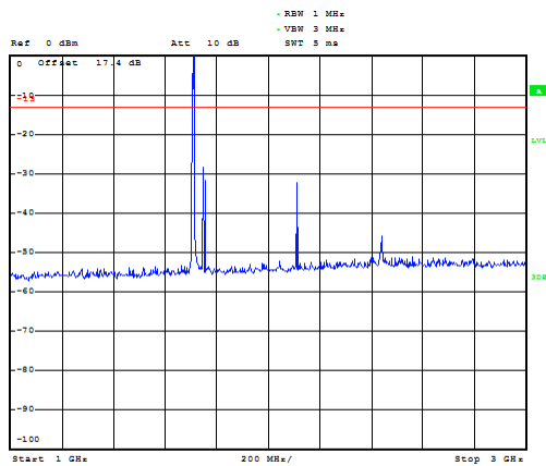
LTE Band 4 1.4MHz CH-Low 1GHz~3GHz
