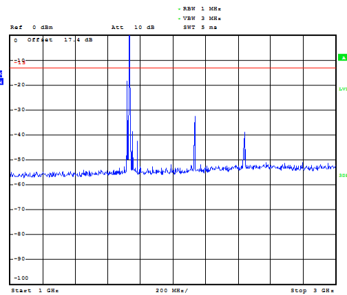
LTE Band 4 1.4MHz CH-Middle 1GHz~3GHz
