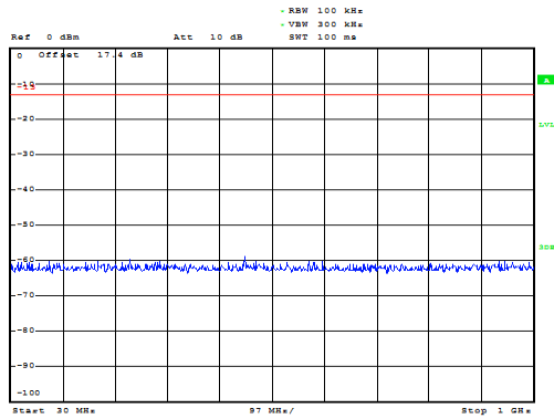
LTE Band 4 1.4MHz CH-Low 30MHz~1GHz
