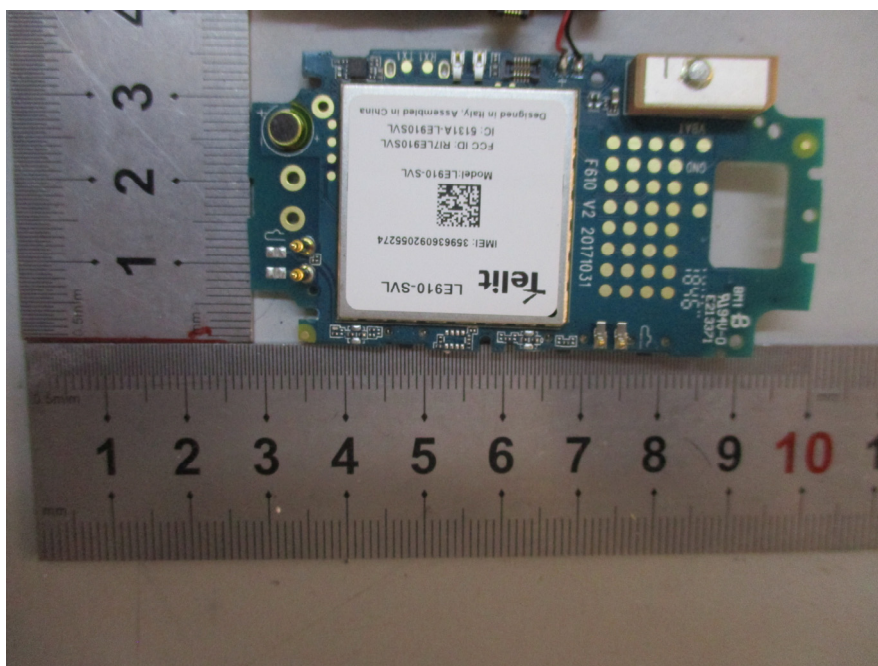
Tracker – PCB Bottom View
