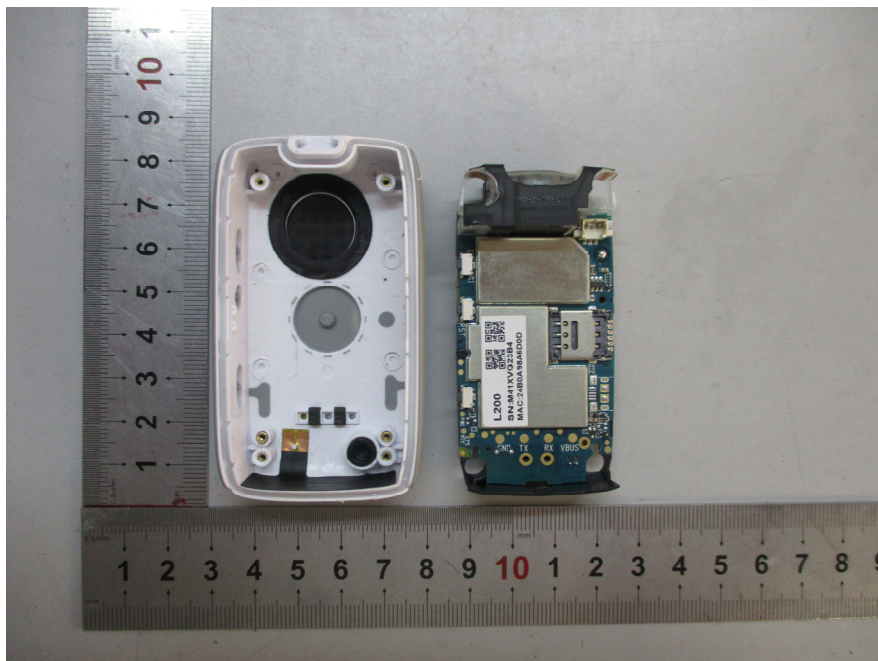
Tracker– Cover off View-3
