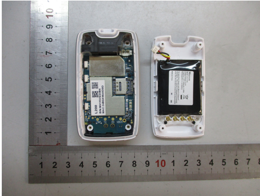
Tracker– Cover off View-2
