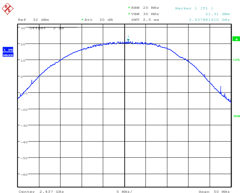
Fig.5 Peak Conducted Output Power CH6, 11b, Rate1
