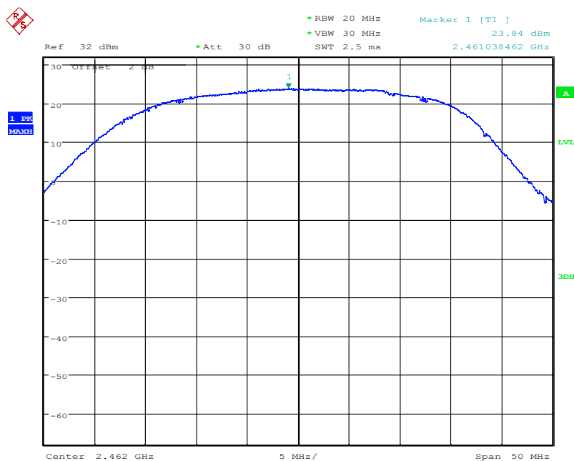
Fig.53 Peak Conducted Output Power CH11, 11n, MCS0
