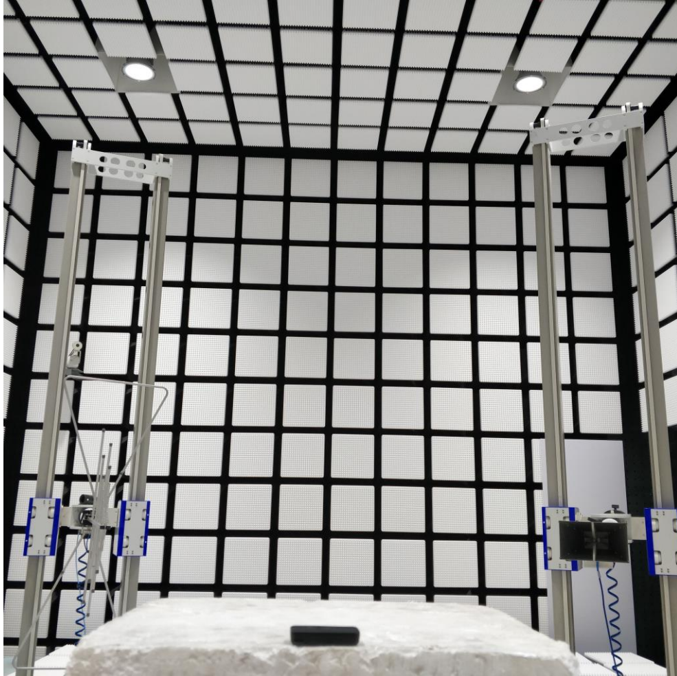
Pic3. Radiated spurious emission (Above 1GHz)
