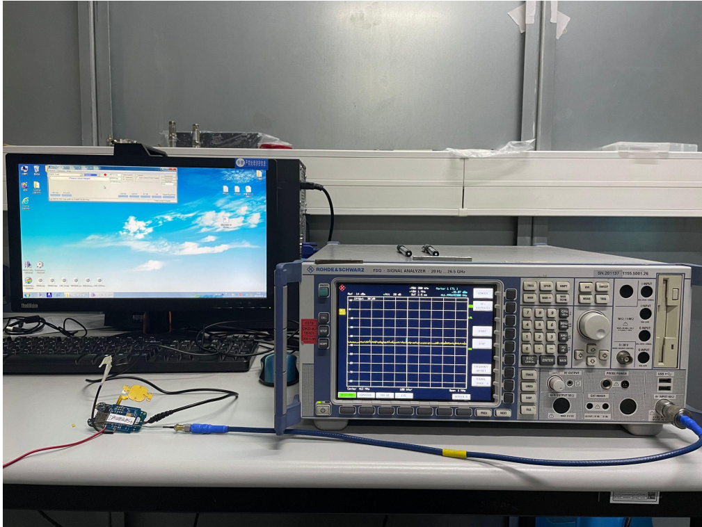
WLAN test setup photo
