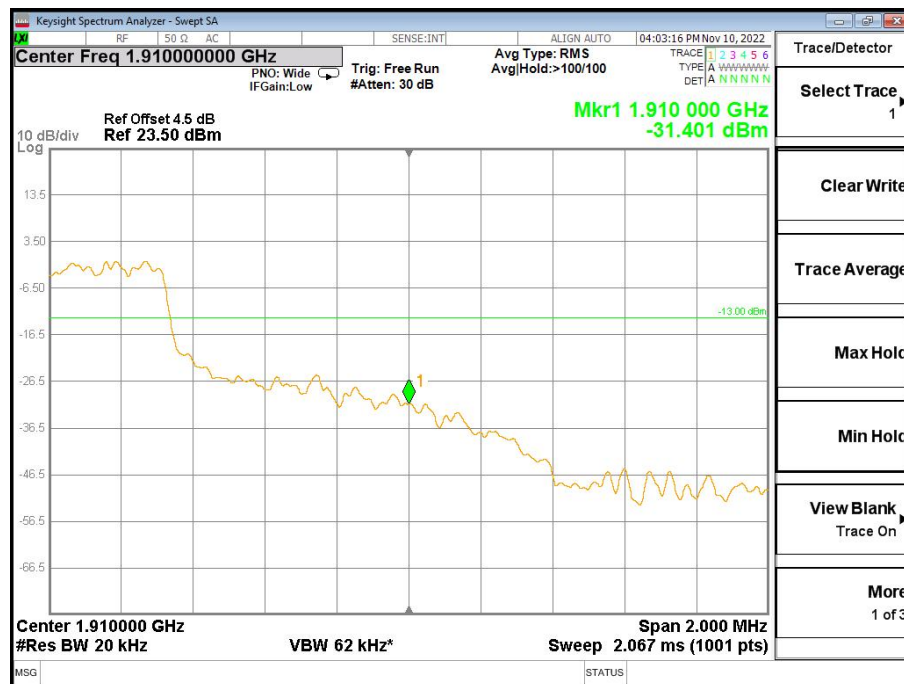
Band2-High Channel-10MHz Bandwidth-6RB-QPSK
