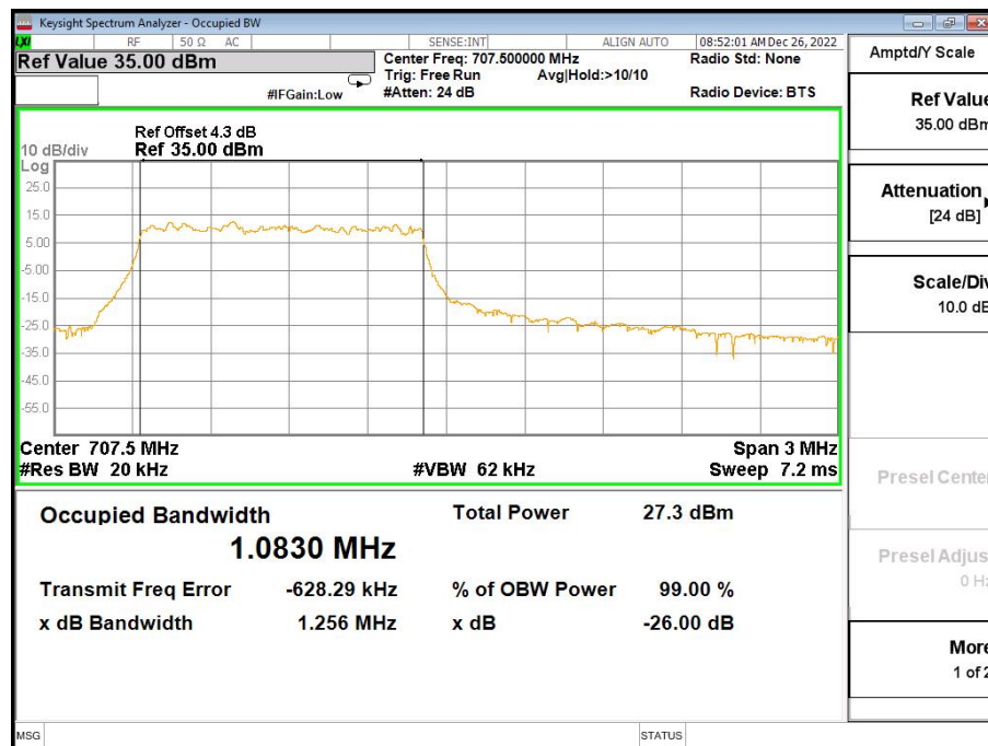
Band12-3MHz Bandwidth-QPSK
