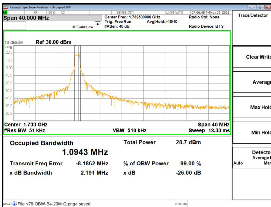
Band4-20MHz Bandwidth-16QAM
