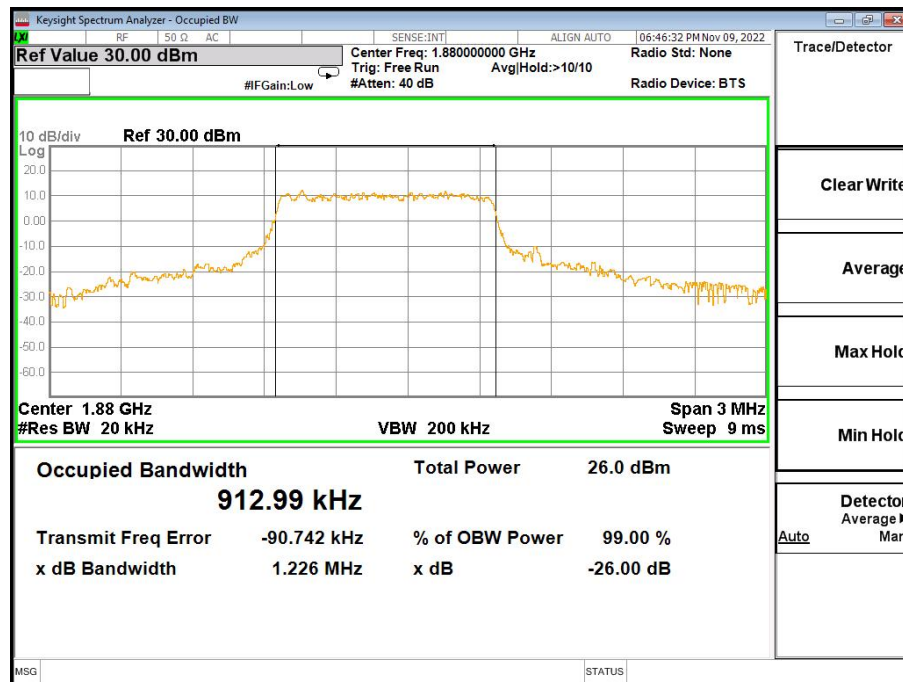
Band2-1.4MHz Bandwidth-16QAM
