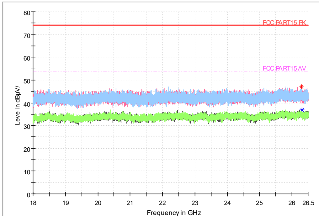
Fig.25 Radiated emission: 18 GHz - 26.5 GHz
