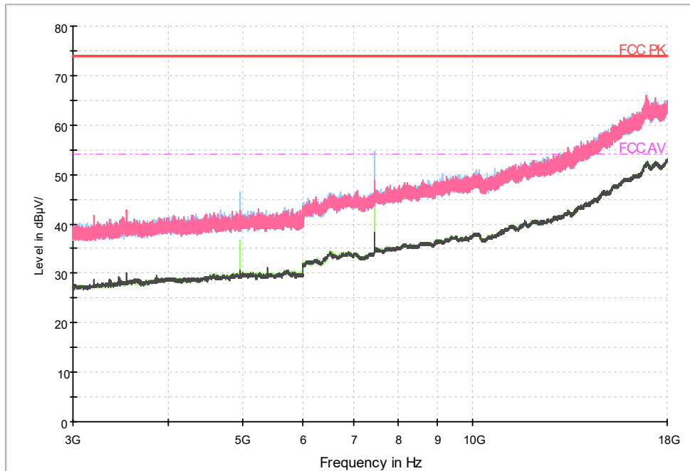
Fig.24 Radiated emission: Ch39, 1M 3GHz-18GHz
