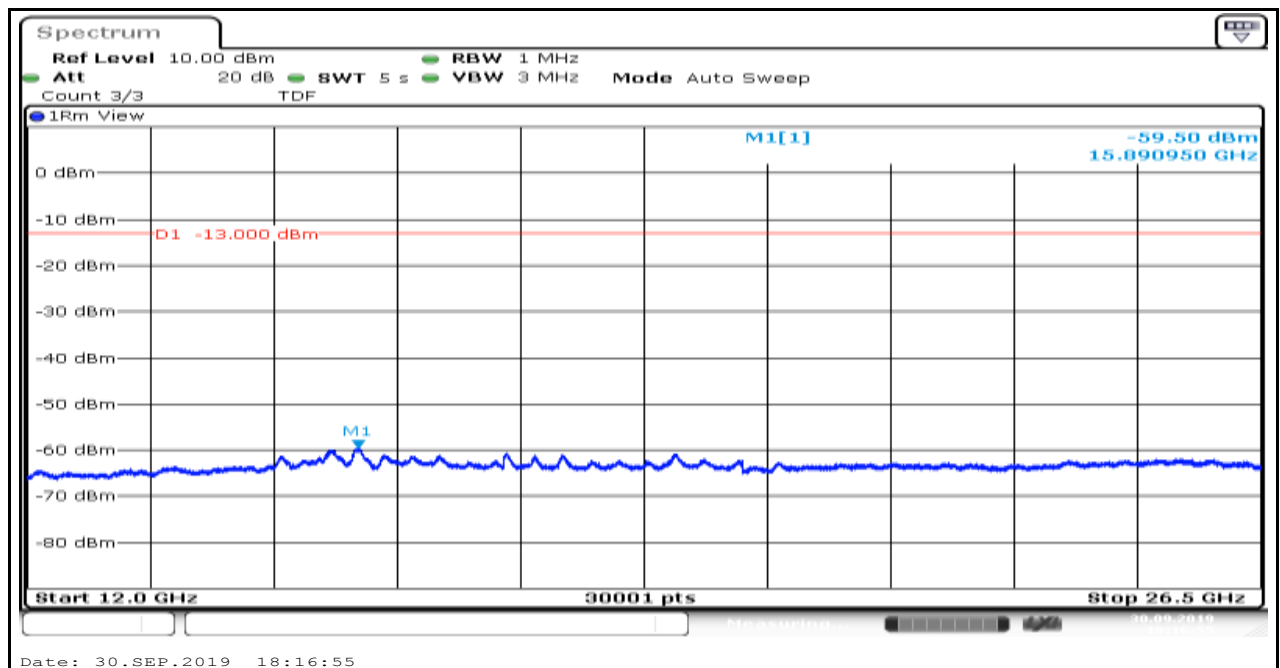
Band85_5MHz_QPSK_134157_3
