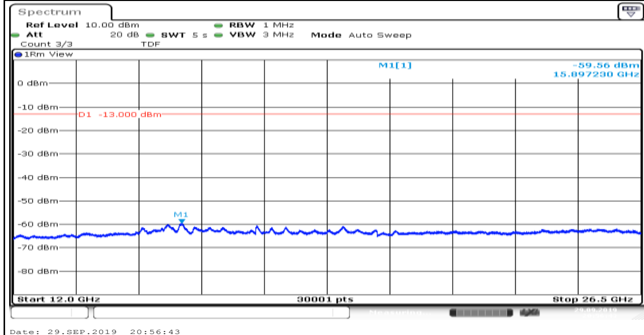
Band4_1.4MHz_16QAM_19957_1
