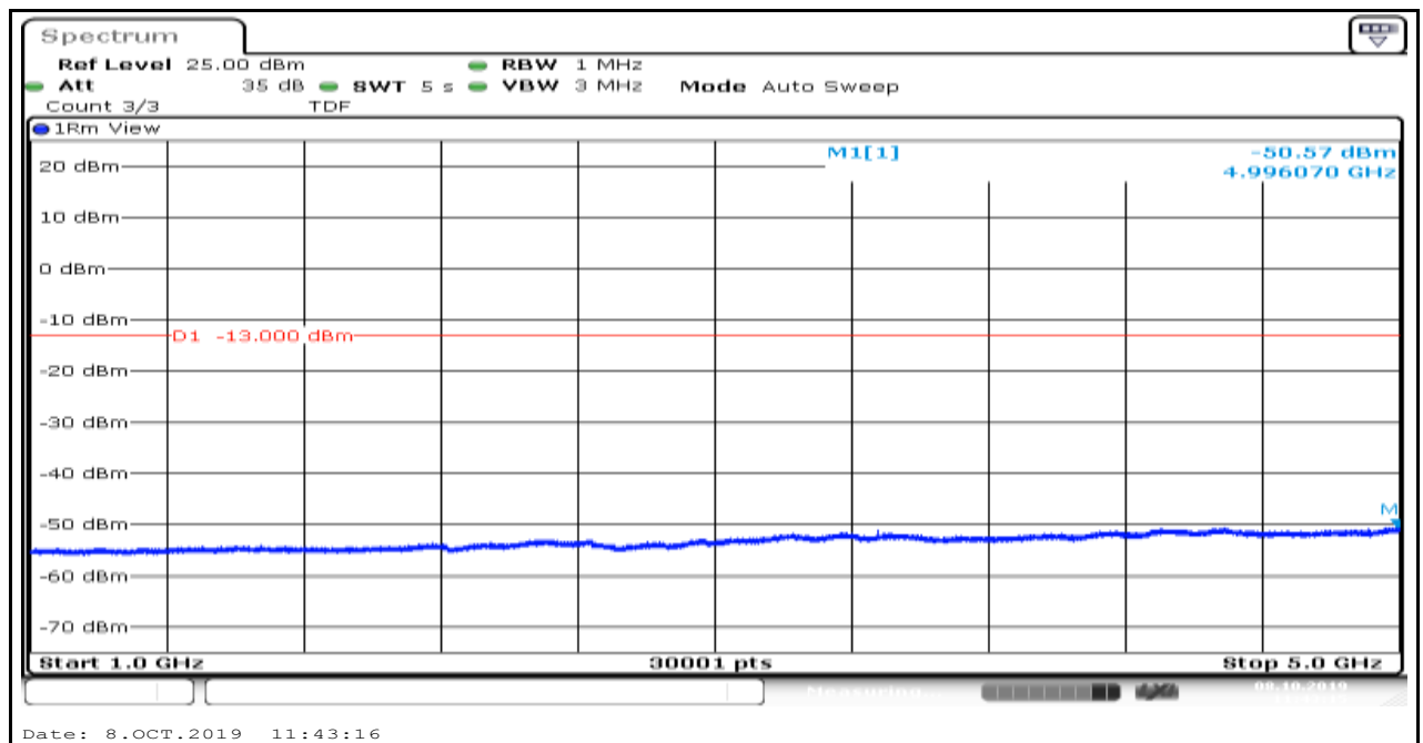
Band5_1.4MHz_QPSK_20525_1
