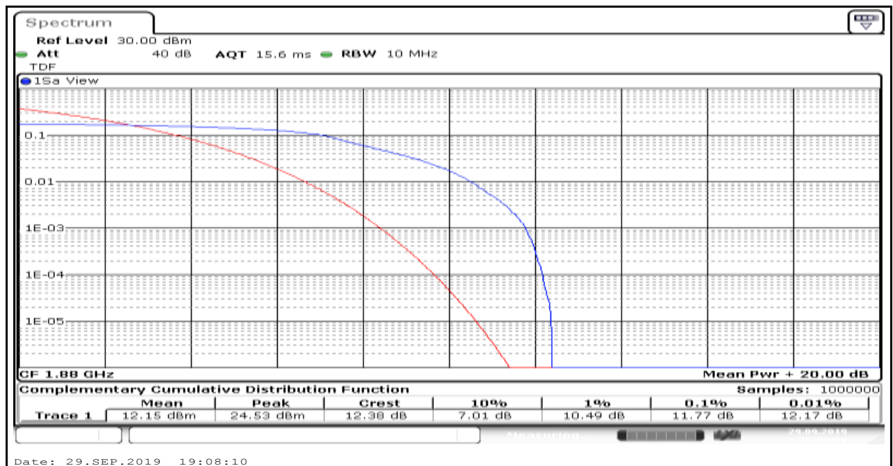
Band2_3MHz_16QAM_18900_6
