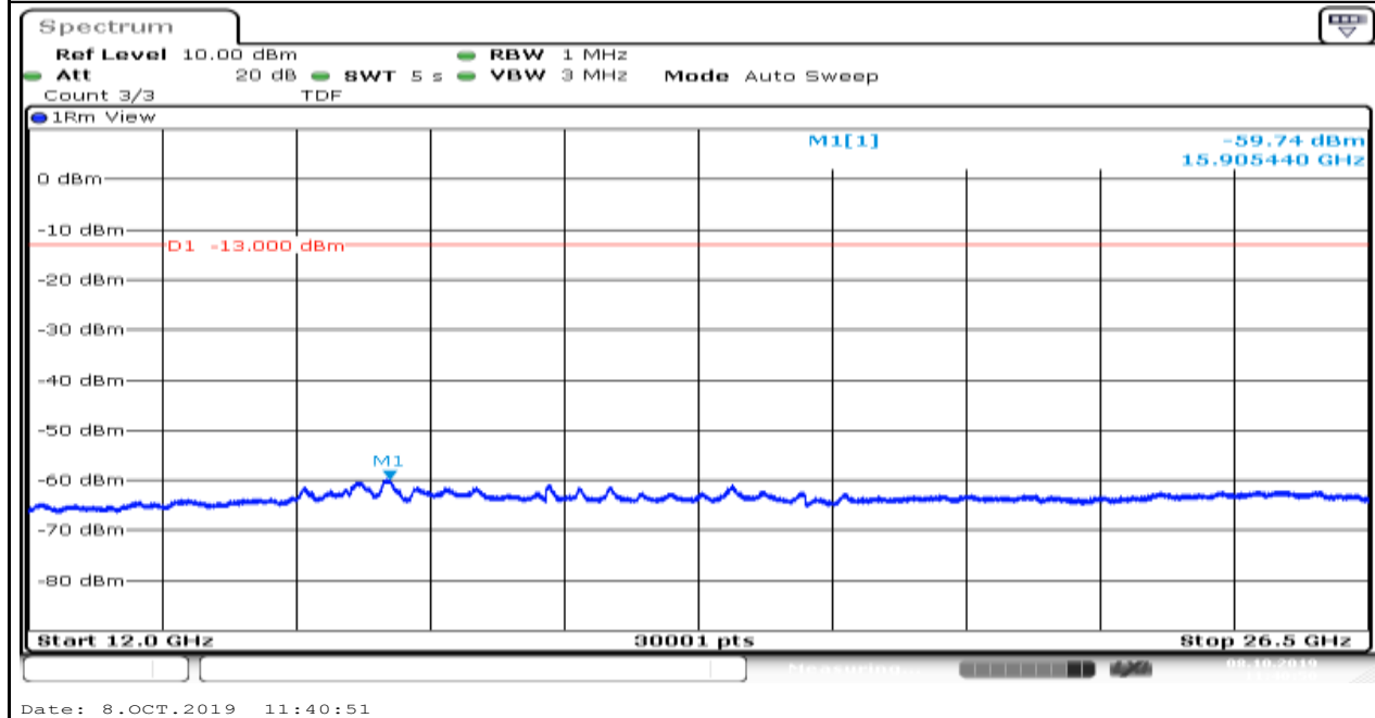
Band5_1.4MHz_QPSK_20525_1
