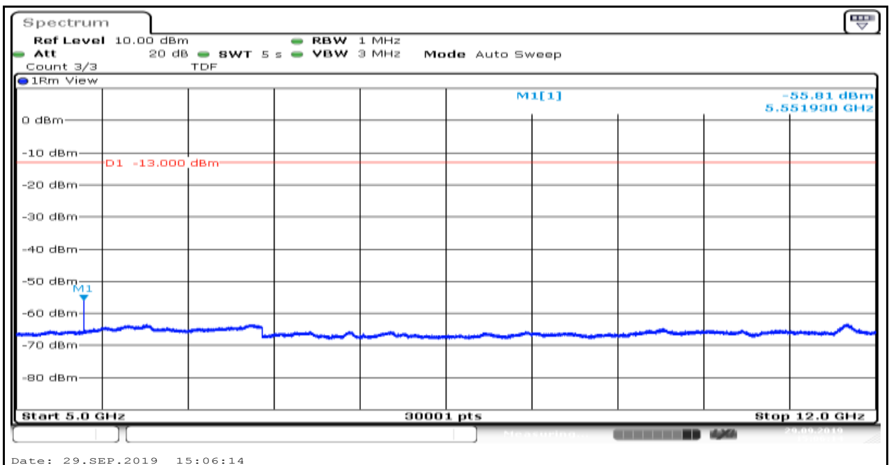
Band2_1.4MHz_16QAM_18607_6
