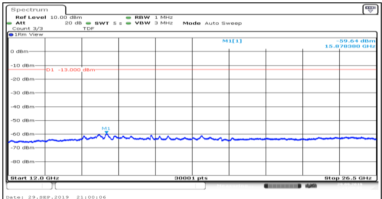
Band4_1.4MHz_16QAM_20175_6
