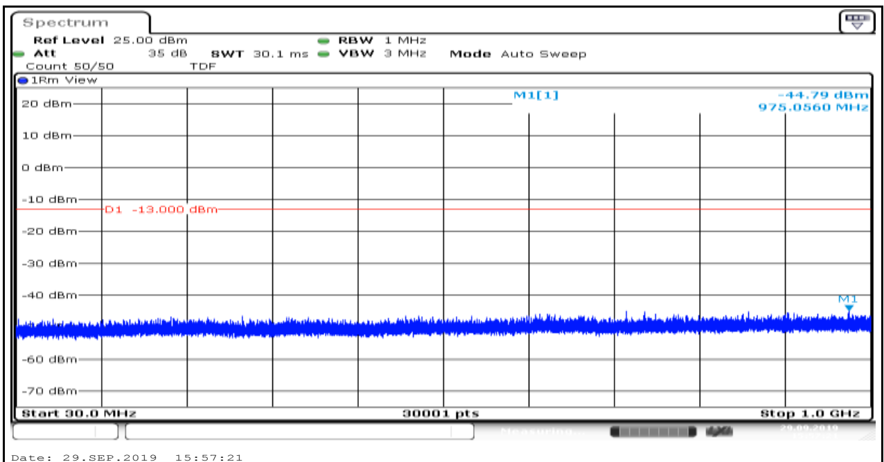
Band2_1.4MHz_16QAM_18900_6
