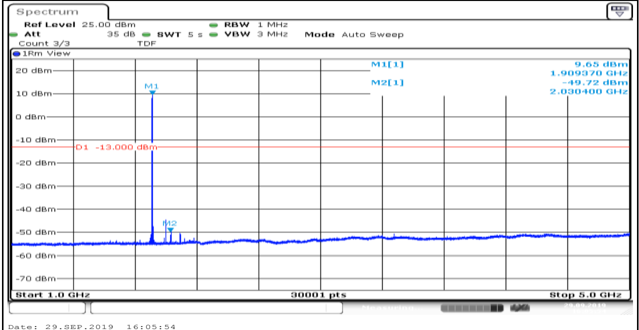
Band2_1.4MHz_QPSK_19193_1
