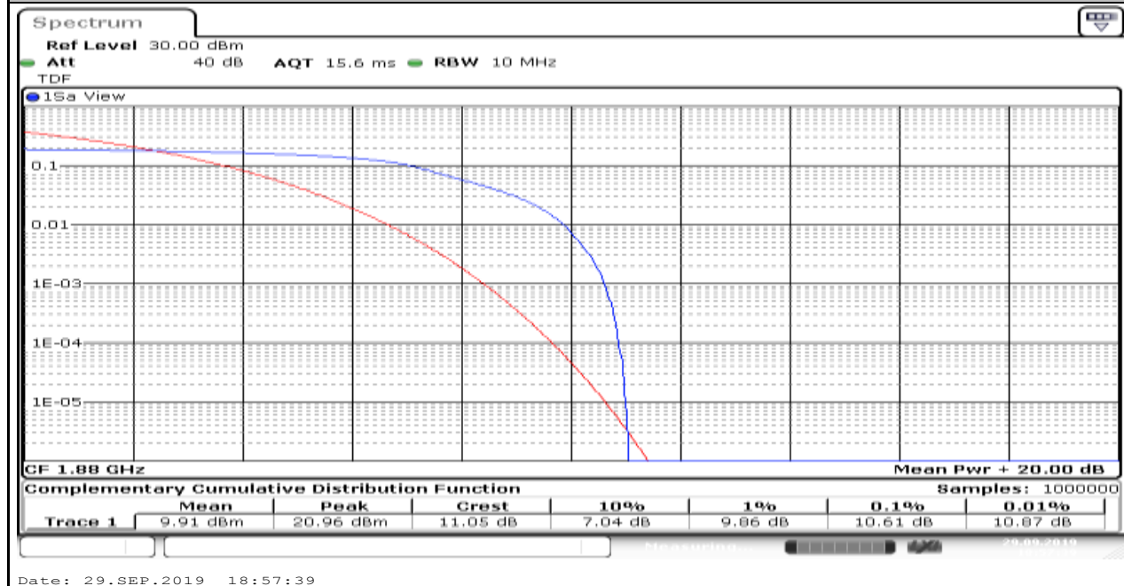
Band2_10MHz_16QAM_18900_6
