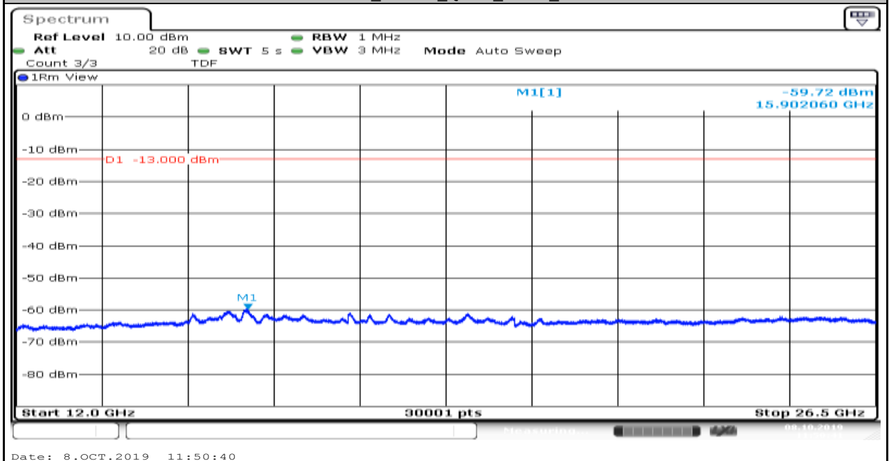
Band5_1.4MHz_QPSK_20525_6
