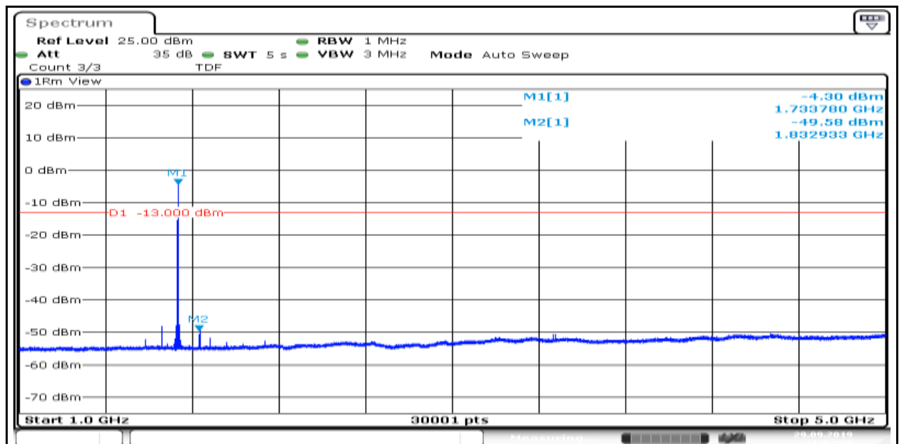
Band4_1.4MHz_16QAM_20175_6
