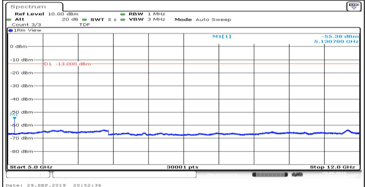
Band4_1.4MHz_16QAM_19957_1
