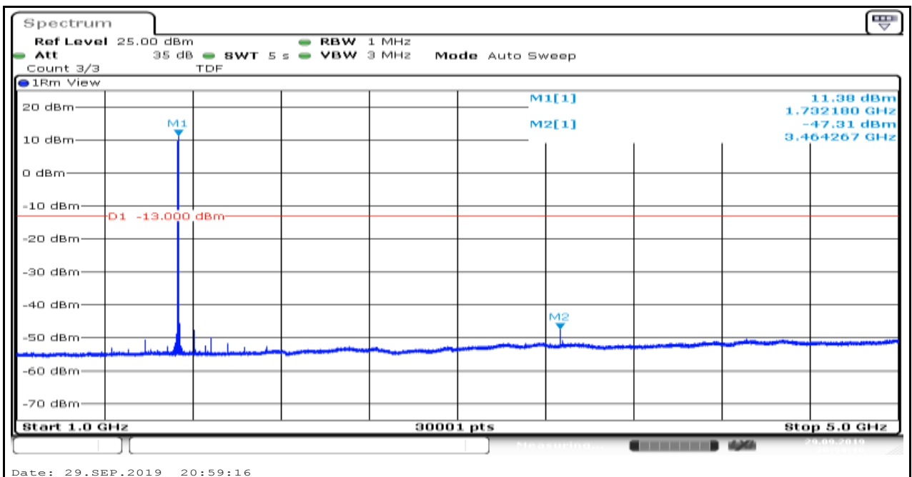
Band4_1.4MHz_16QAM_20393_1
