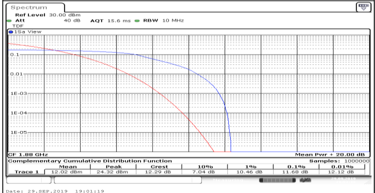
Band2_20MHz_16QAM_18900_6
