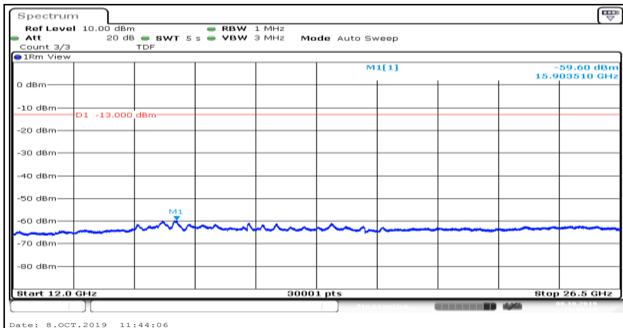
Band5_1.4MHz_QPSK_20525_1
