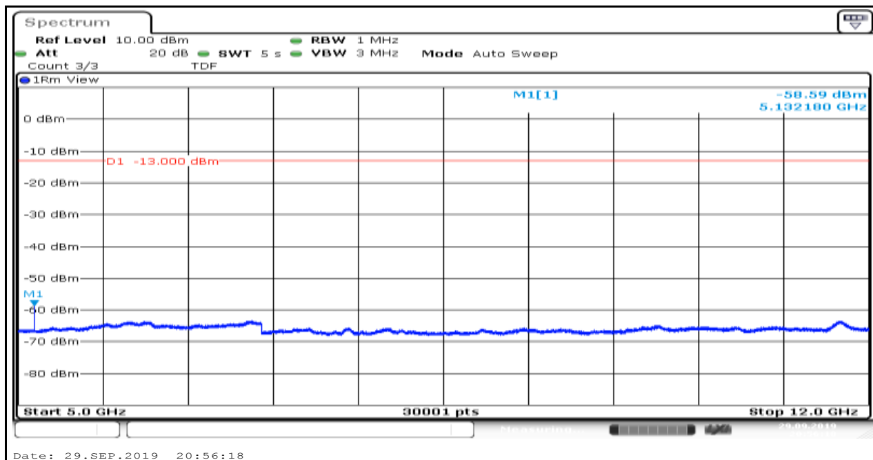
Band4_1.4MHz_16QAM_19957_6
