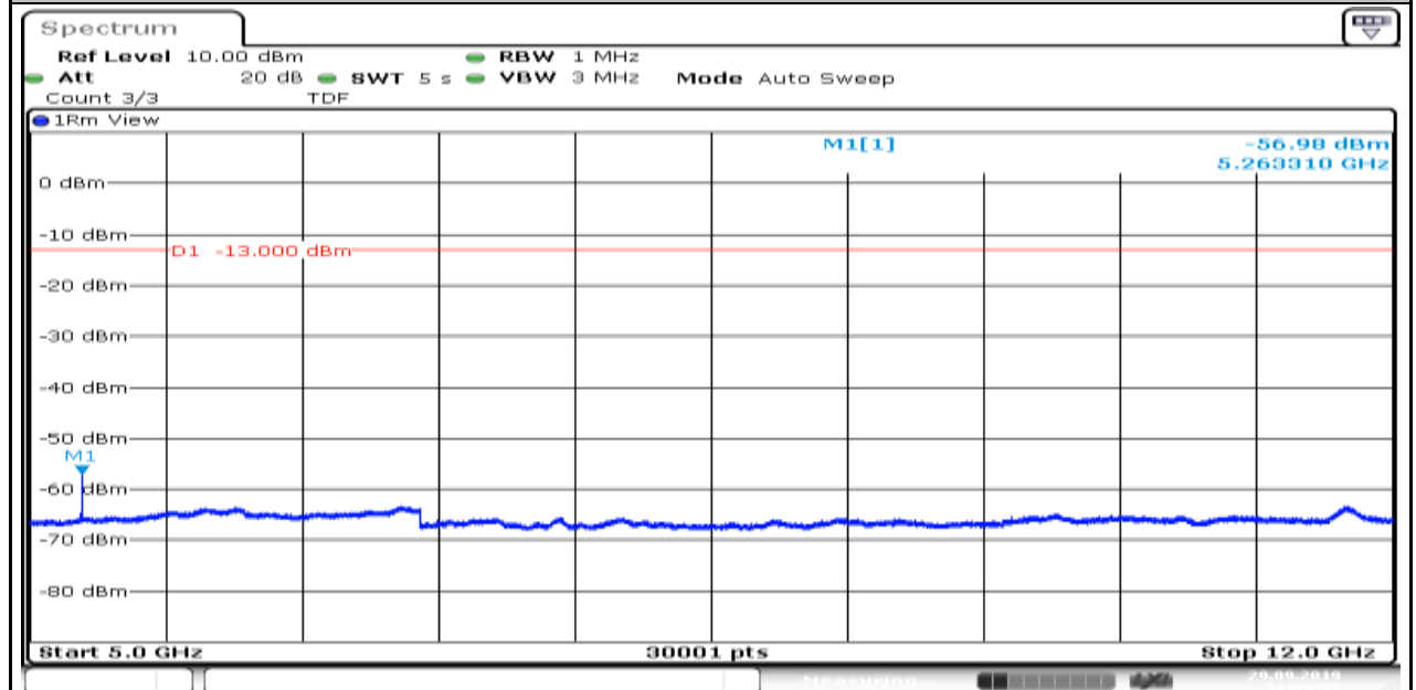
Band4_1.4MHz_QPSK_20393_5
