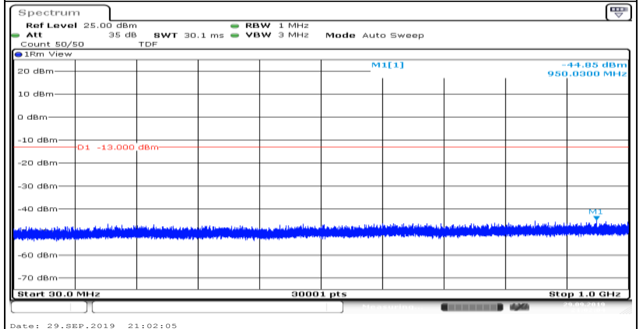
Band4_1.4MHz_16QAM_20175_1
