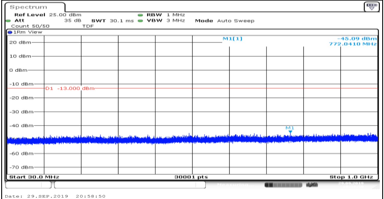
Band4_1.4MHz_16QAM_20175_6
