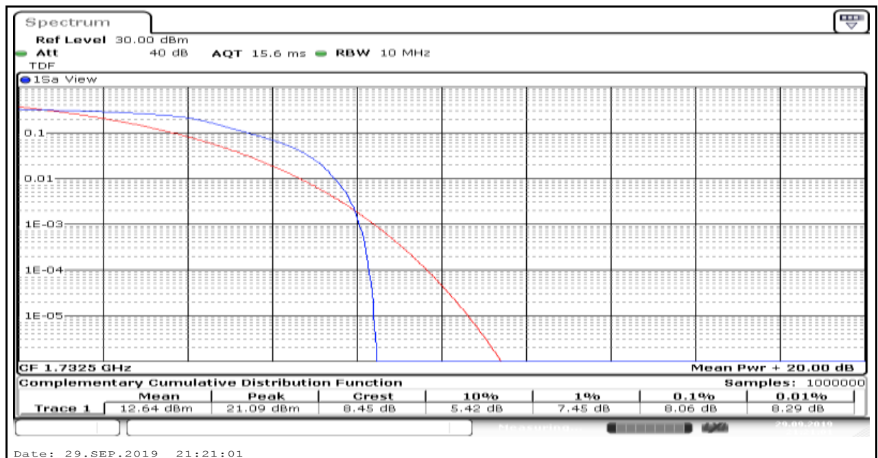
Band4_10MHz_16QAM_20175_6
