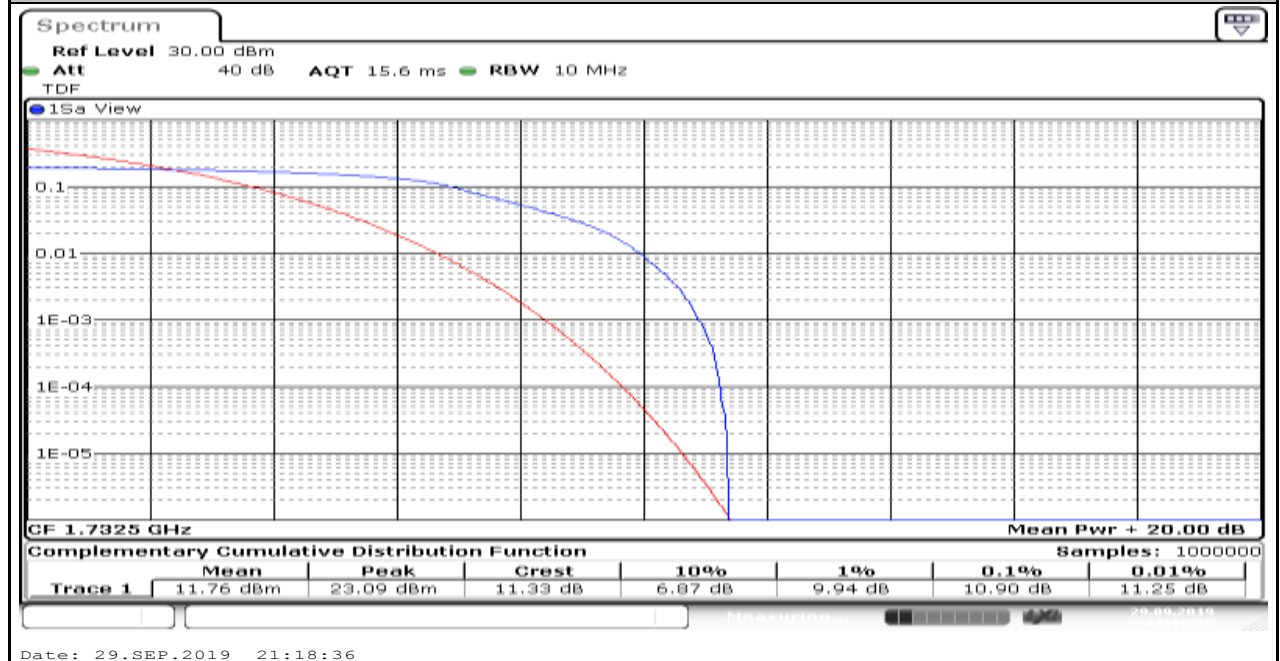
Band4_20MHz_16QAM_20175_6
