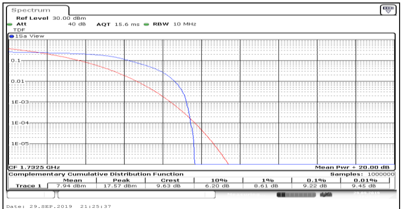
Band4_15MHz_QPSK_20175_6
