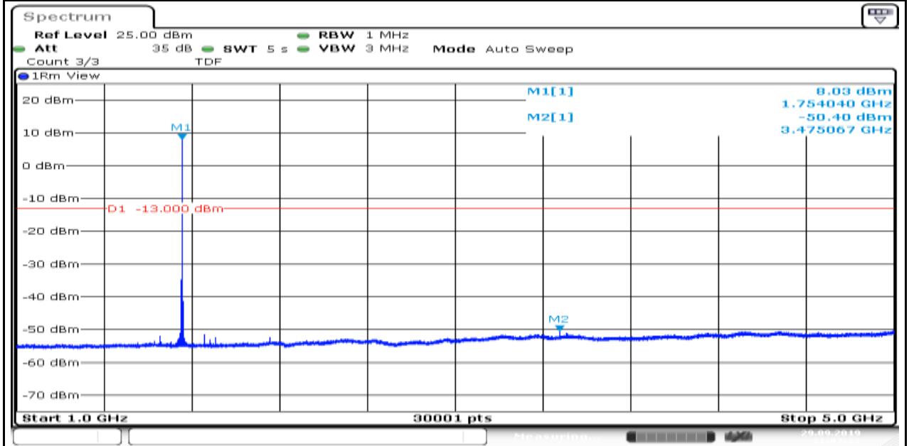
Band4_1.4MHz_QPSK_20393_6
