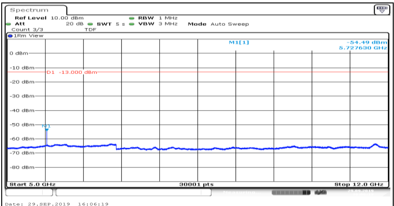
Band2_1.4MHz_QPSK_19193_6
