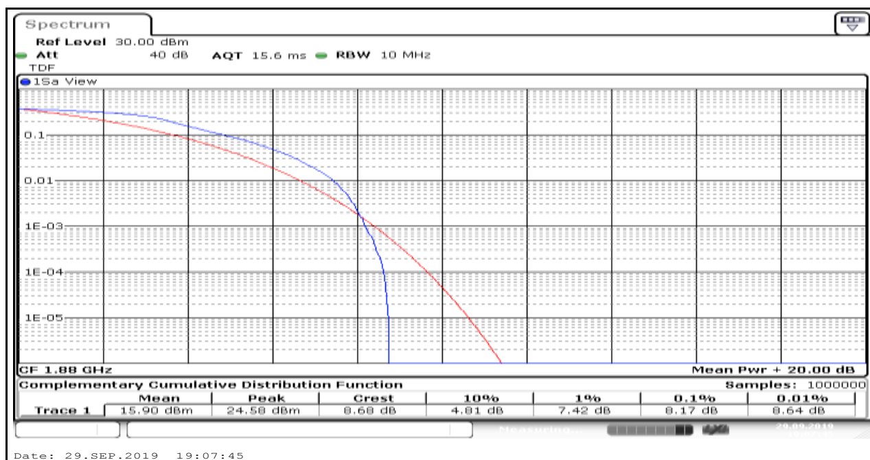
Band2_15MHz_16QAM_18900_6
