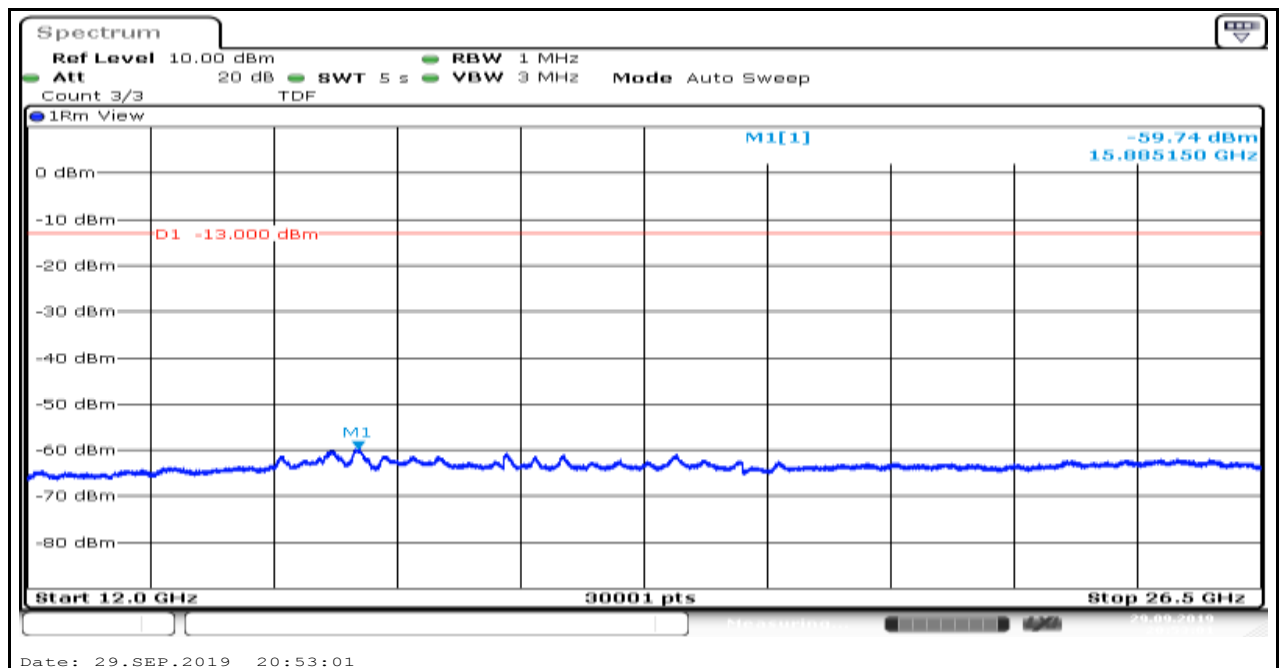
Band4_1.4MHz_16QAM_19957_1
