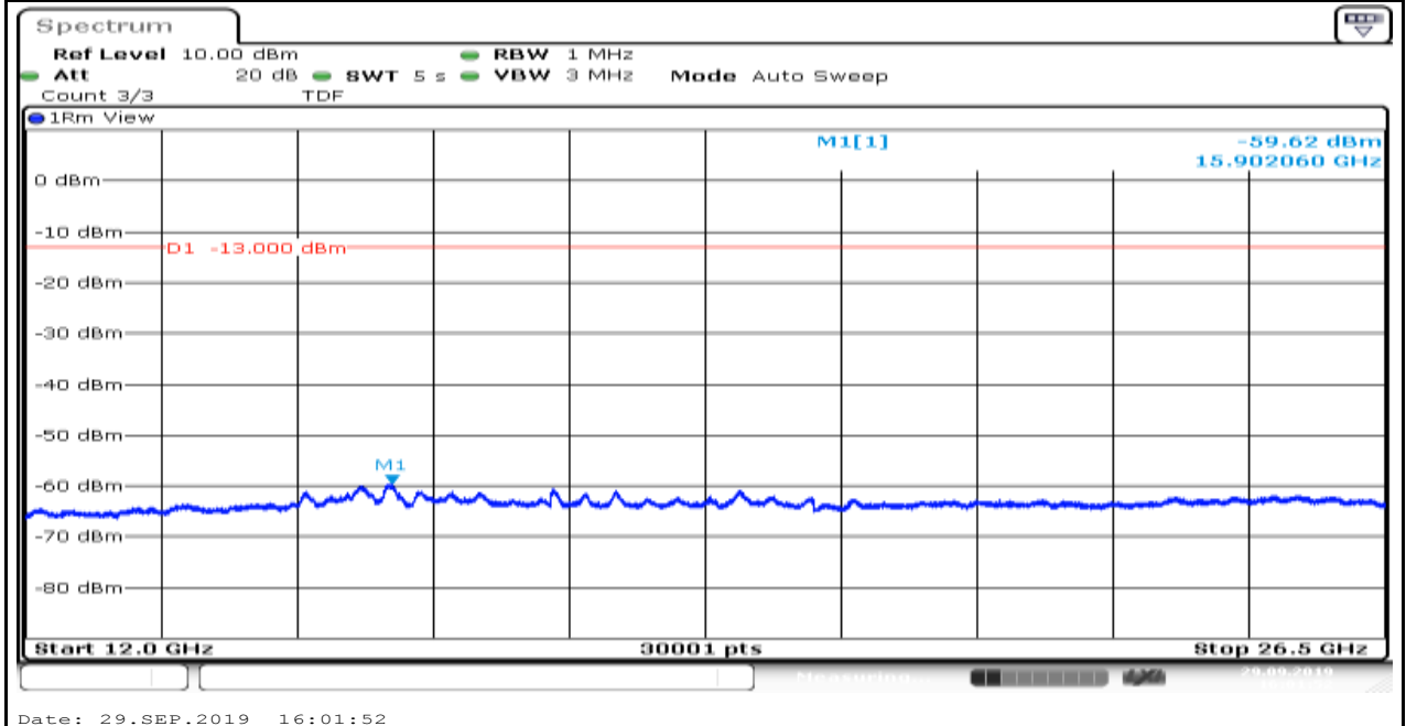
Band2_1.4MHz_16QAM_18900_6
