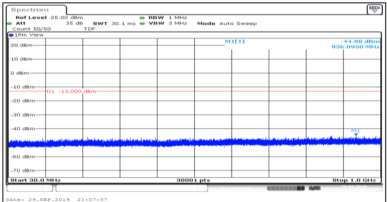
Band4_1.4MHz_QPSK_20393_5
