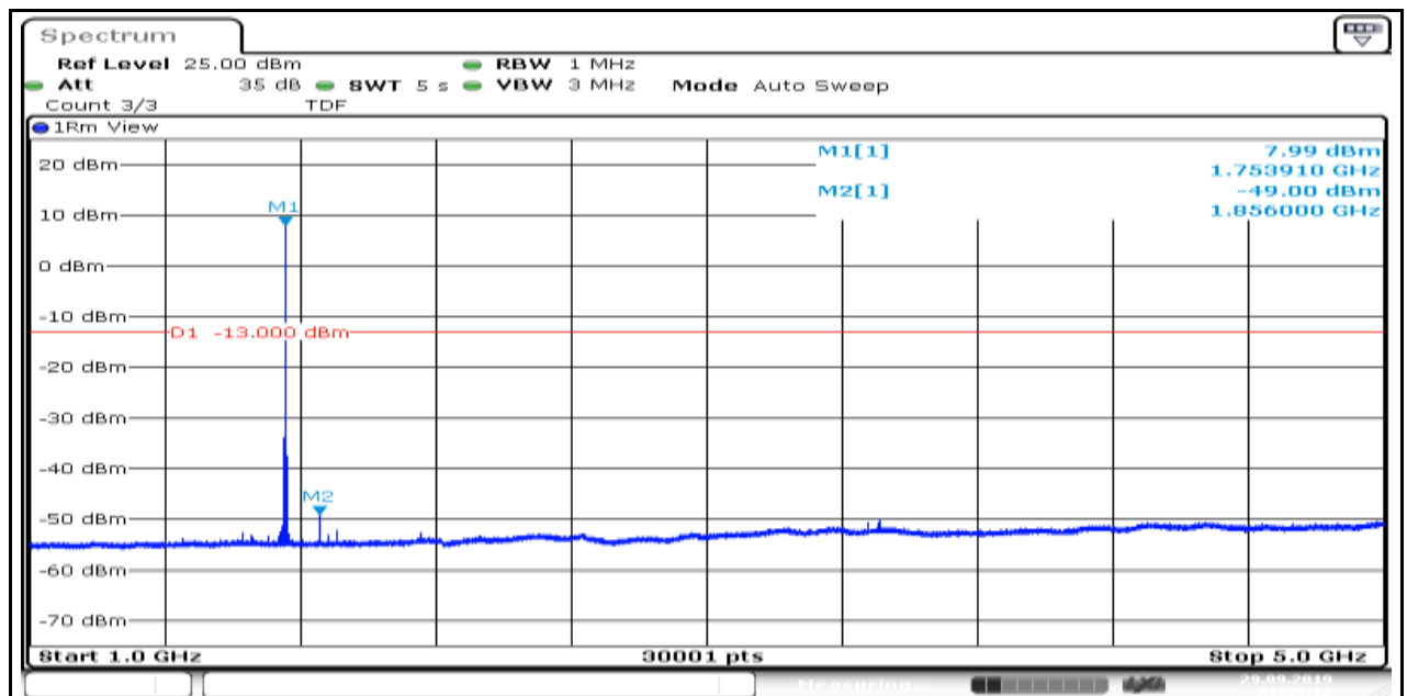
Band4_1.4MHz_QPSK_20393_5
