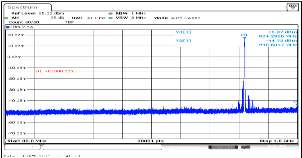
Band5_1.4MHz_QPSK_20407_6
