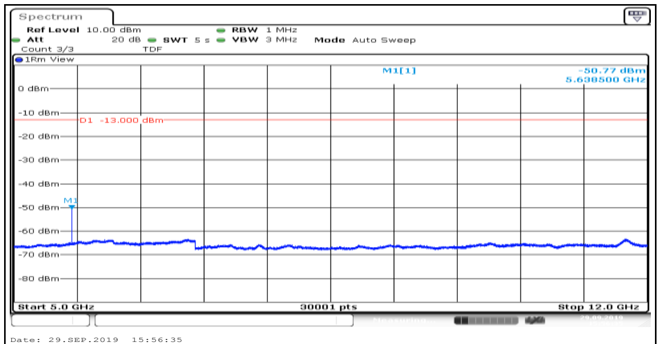
Band2_1.4MHz_QPSK_18900_1
