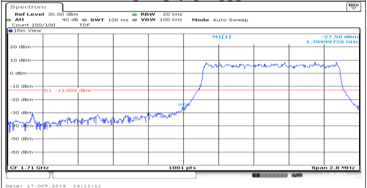
Band4_1.4MHz_16QAM_19957_1_0_Low
