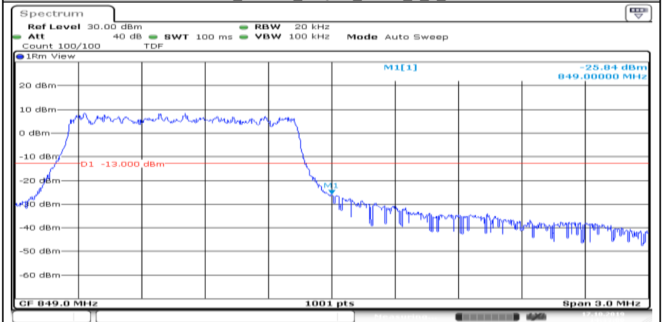
Band5_1.4MHz_16QAM_20643_6_0_Low
