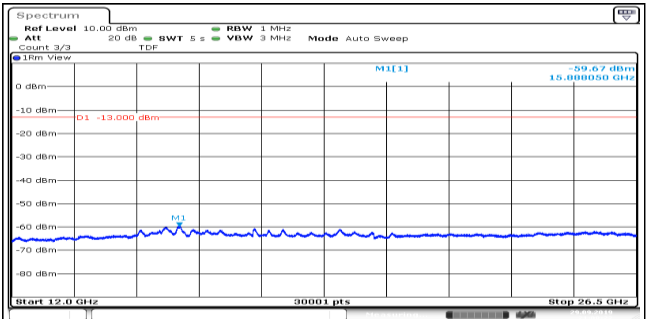
Band4_1.4MHz_QPSK_20393_6
