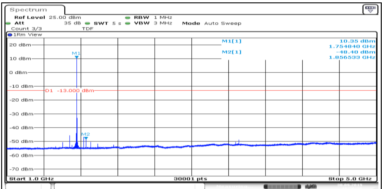
Band4_1.4MHz_16QAM_20393_1
