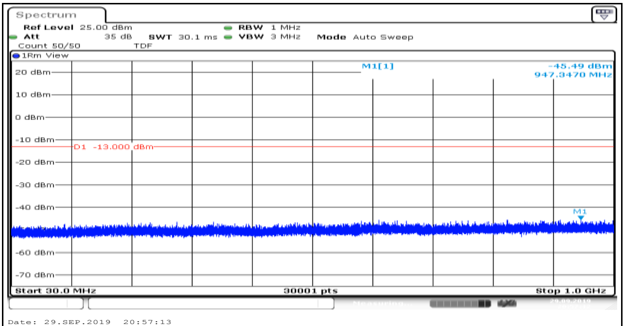
Band4_1.4MHz_QPSK_20175_6
