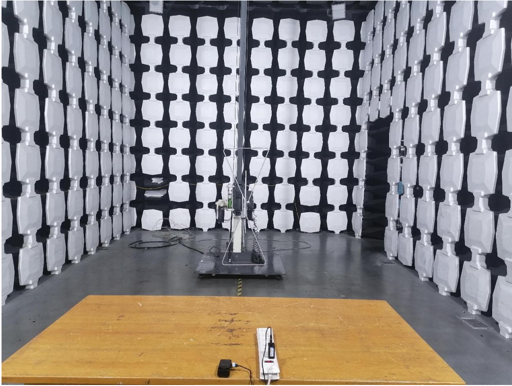
RE_30M-1GHz
