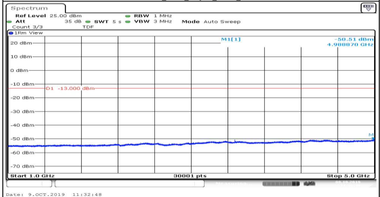
Band13_5MHz_16QAM_23230_1
