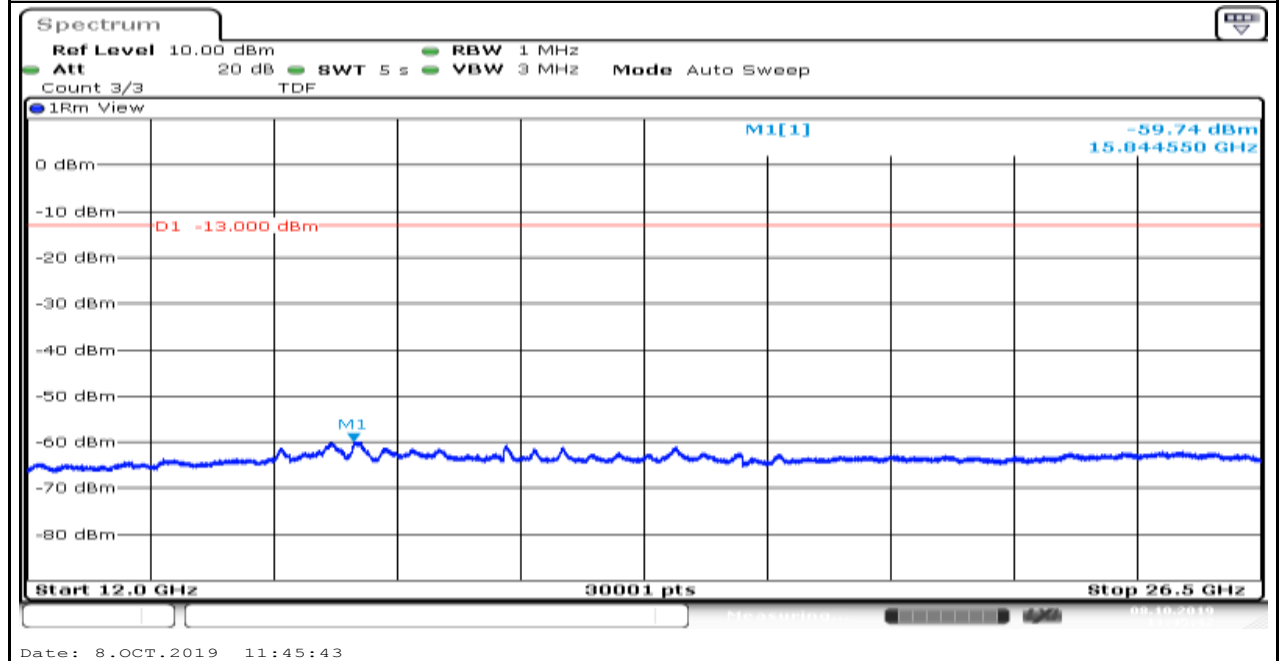
Band5_1.4MHz_16QAM_20525_6
