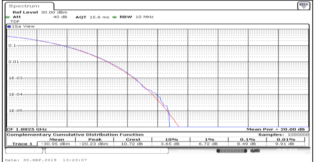
Band25_1.4MHz_QPSK_26365_6
