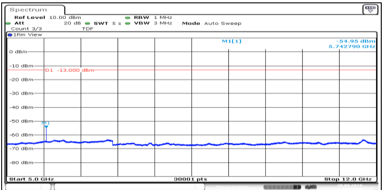
Band25_1.4MHz_QPSK_26683_6
