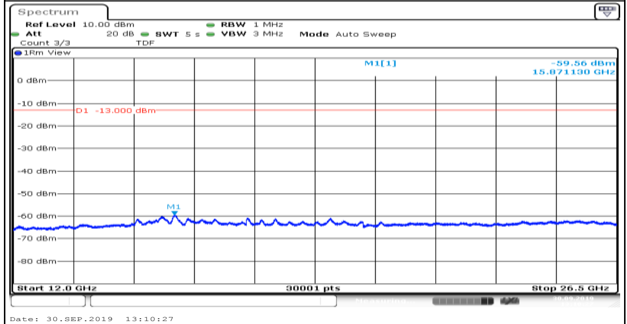
Band25_1.4MHz_QPSK_26683_6
