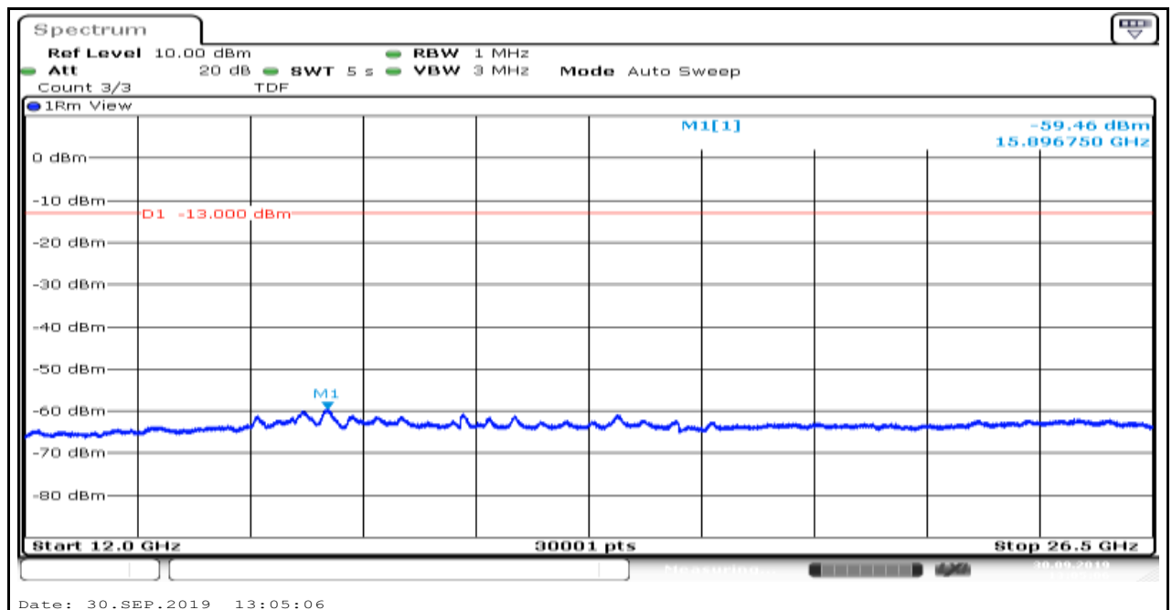
Band25_1.4MHz_QPSK_26683_6
