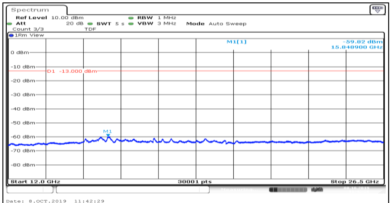
Band5_1.4MHz_16QAM_20525_1
