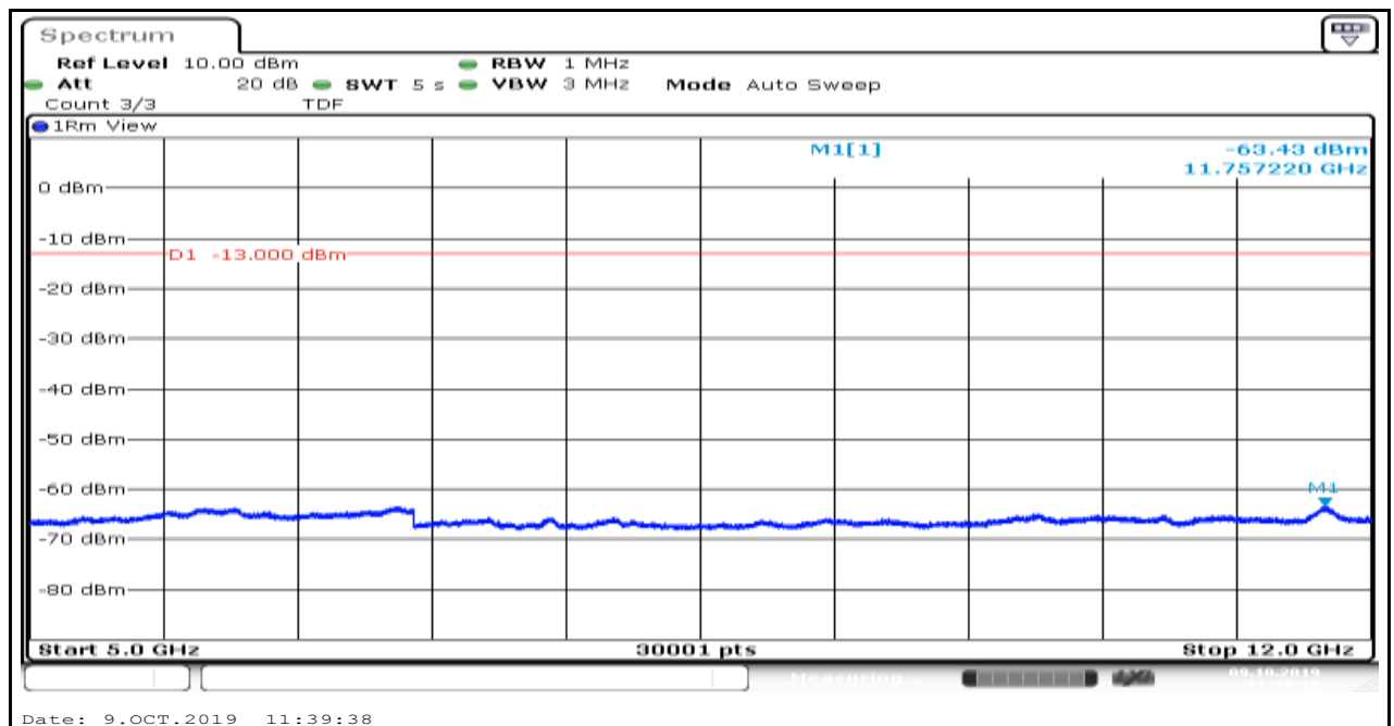
Band13_5MHz_16QAM_23255_1
