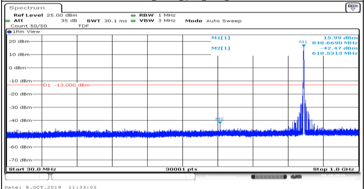
Band5_1.4MHz_QPSK_20643_6
