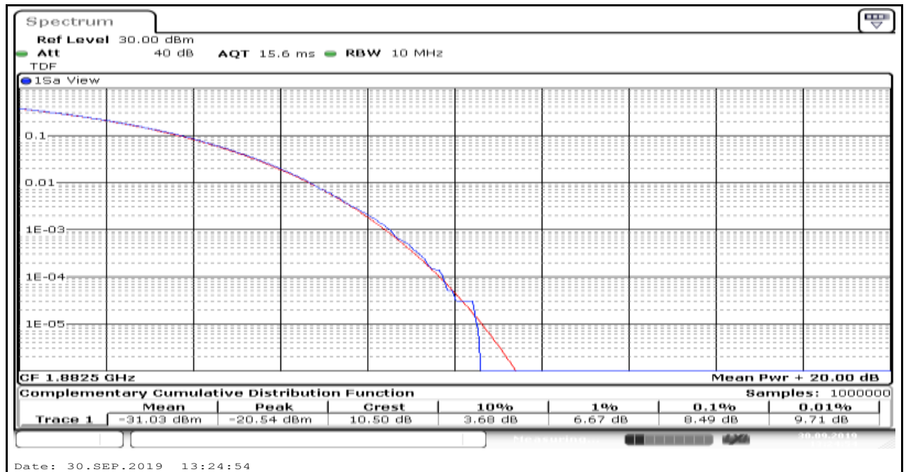
Band25_3MHz_QPSK_26365_6
