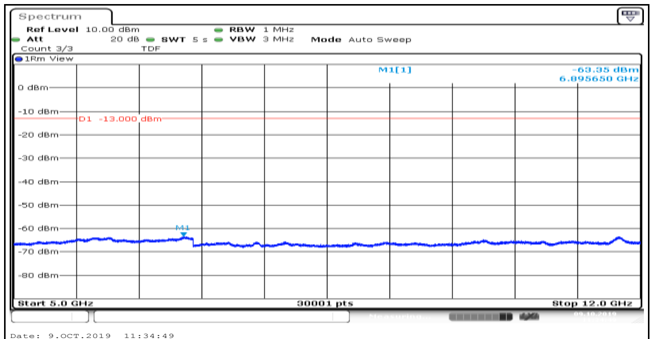
Band13_5MHz_QPSK_23230_6
