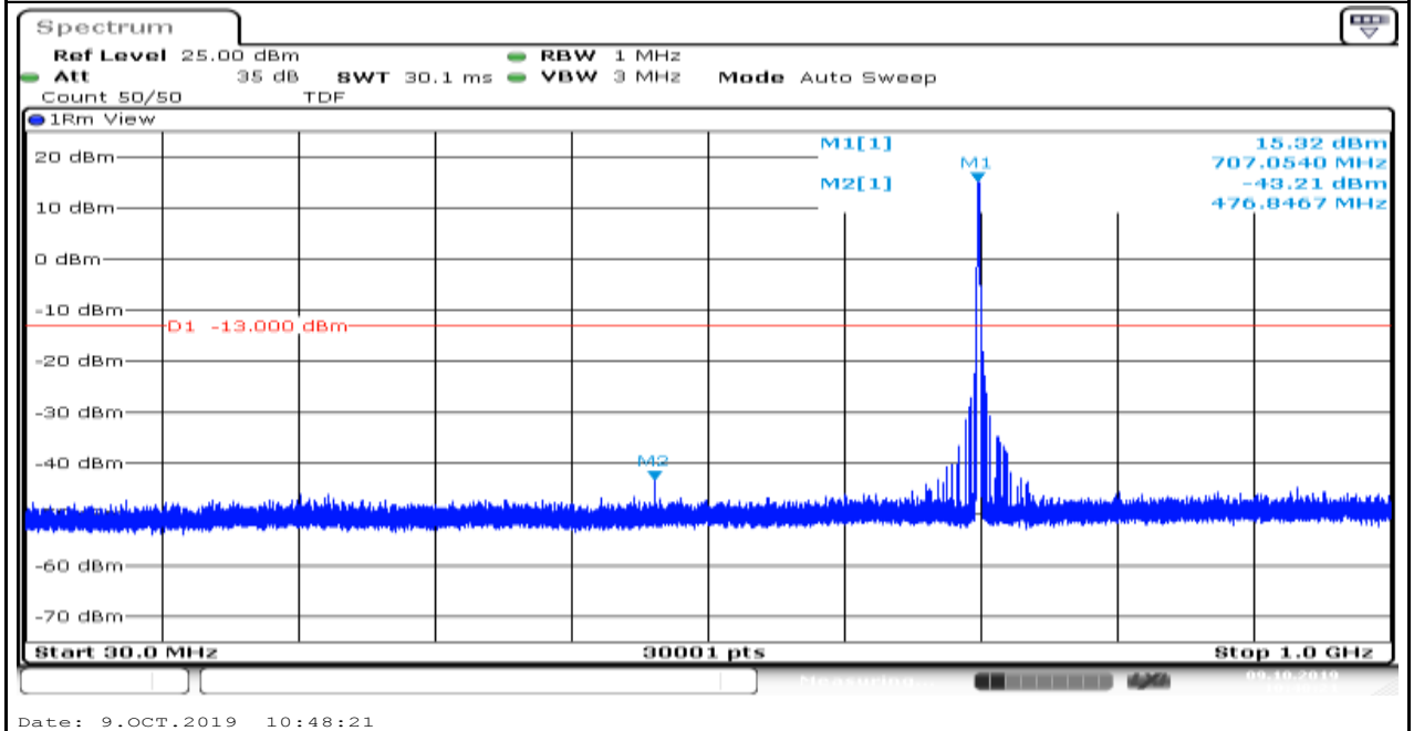
Band12_1.4MHz_QPSK_23095_6
