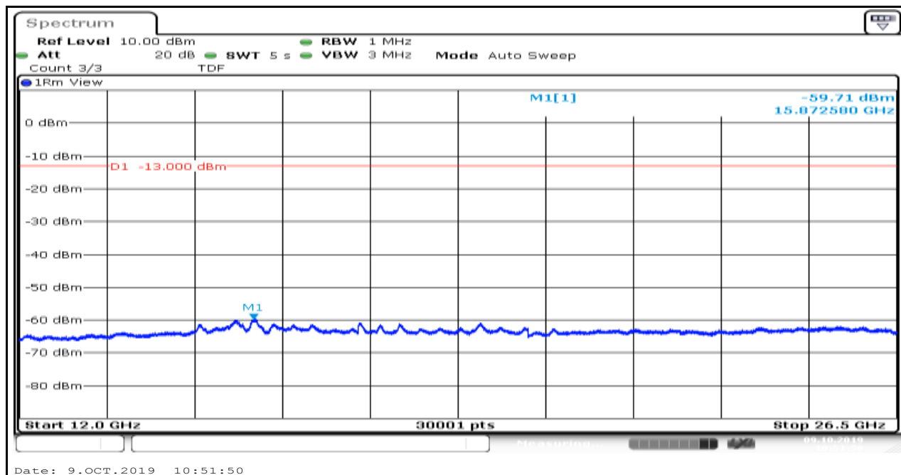
Band12_1.4MHz_16QAM_23095_1
