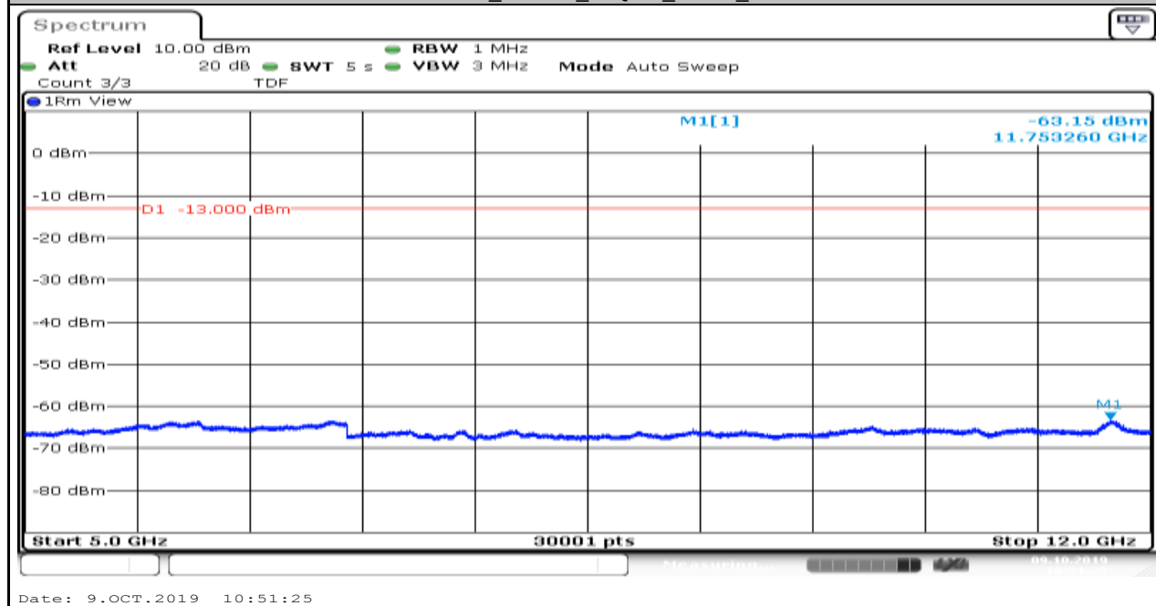
Band12_1.4MHz_16QAM_23173_1
