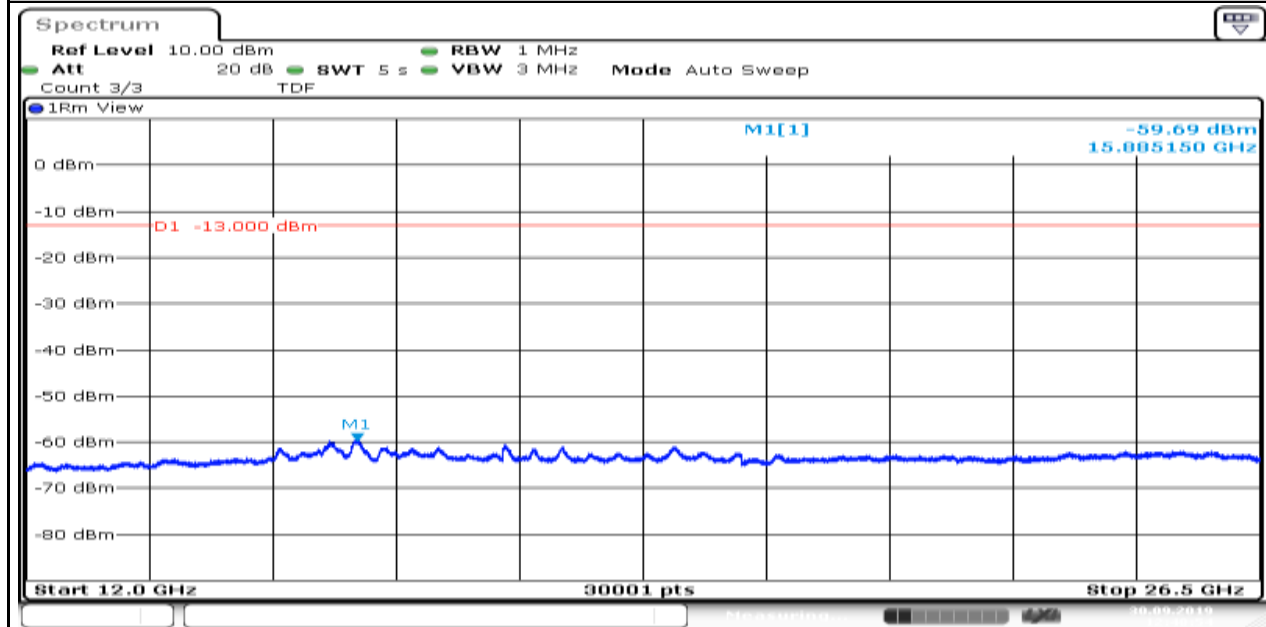
Band25_1.4MHz_QPSK_26047_1
