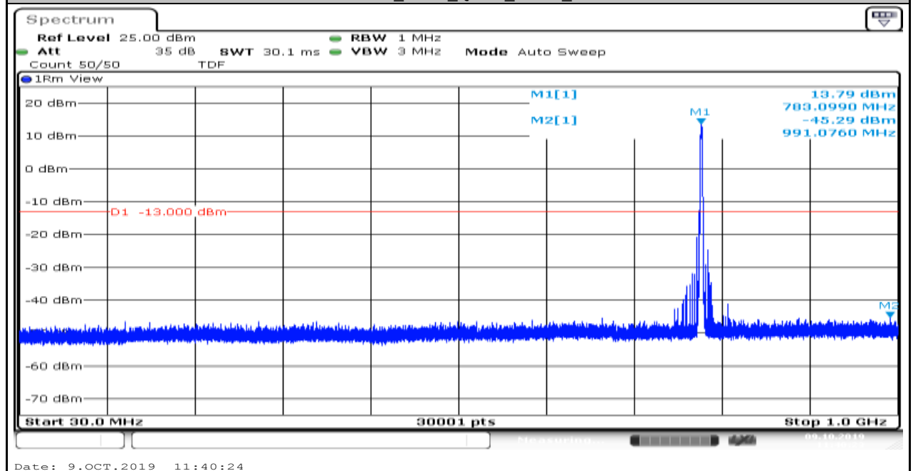
Band13_5MHz_QPSK_23255_1
