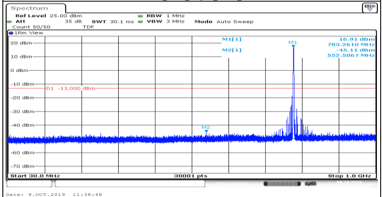
Band13_5MHz_16QAM_23255_6
