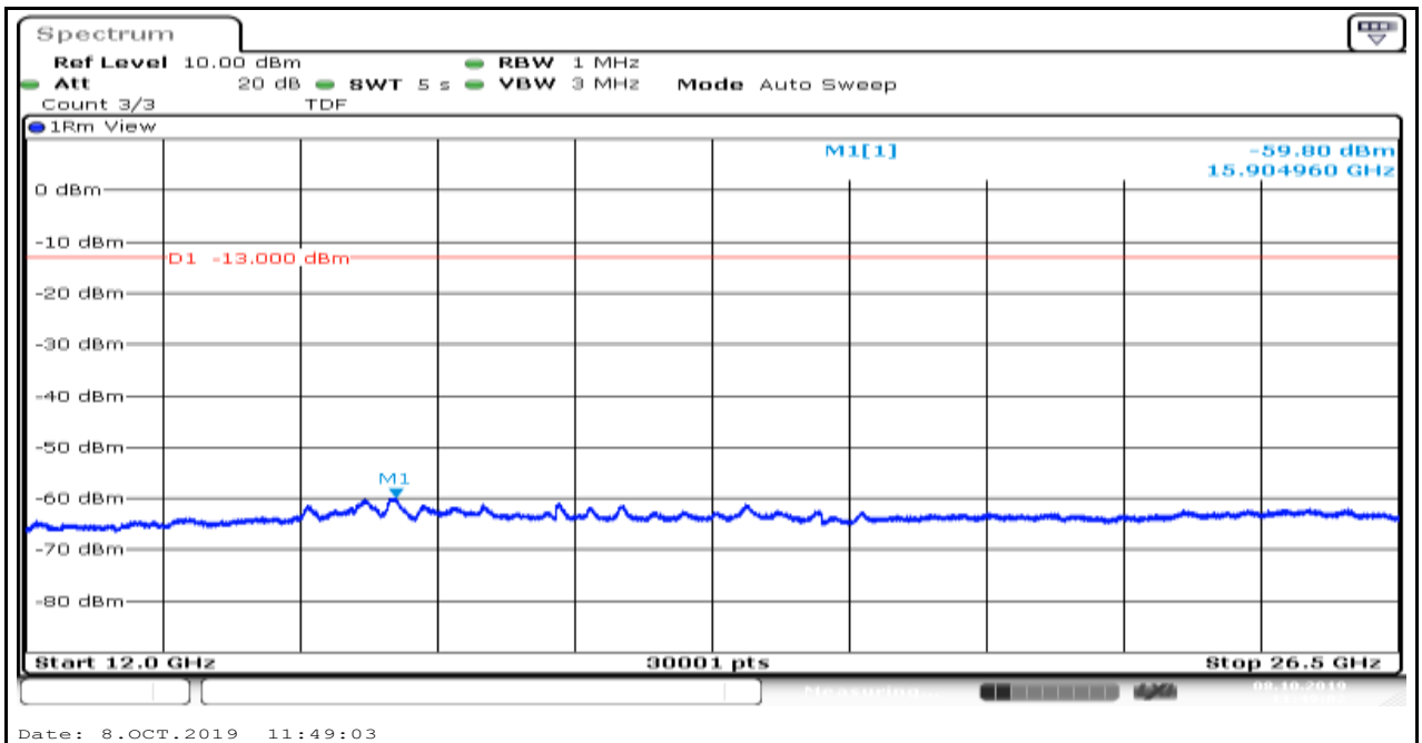
Band5_1.4MHz_16QAM_20407_6
