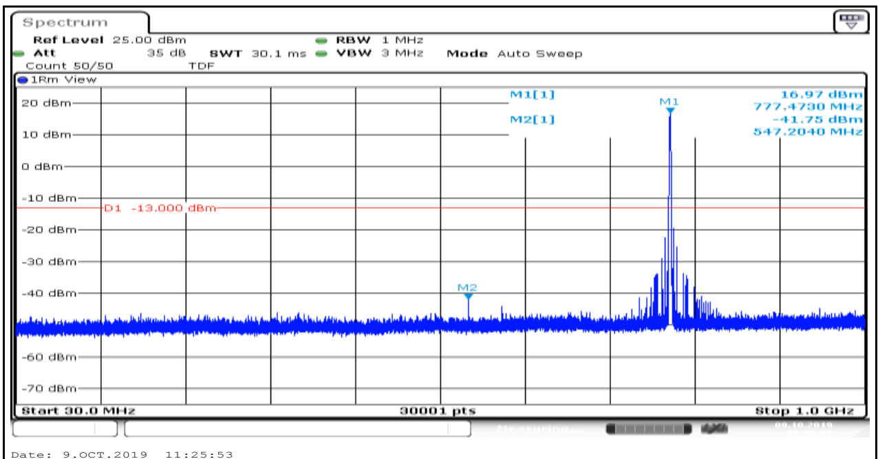
Band13_5MHz_16QAM_23205_6
