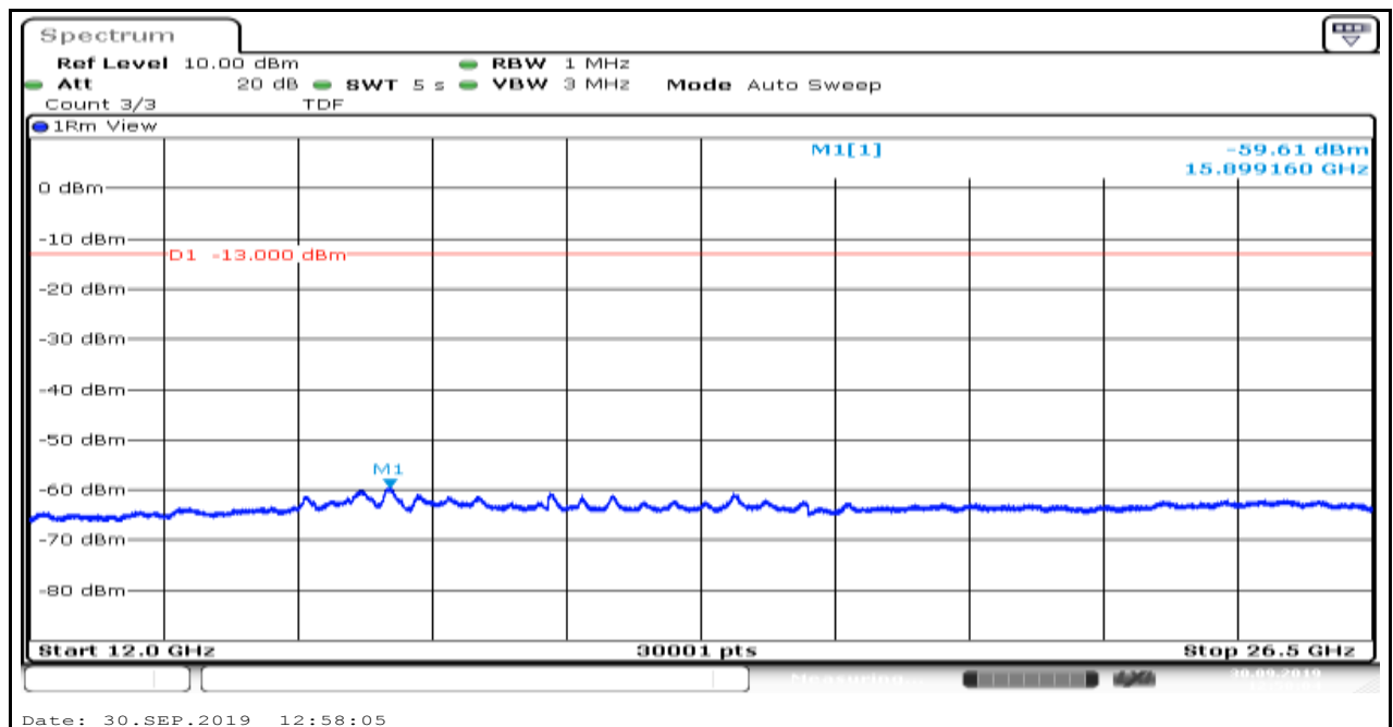
Band25_1.4MHz_16QAM_26365_6
