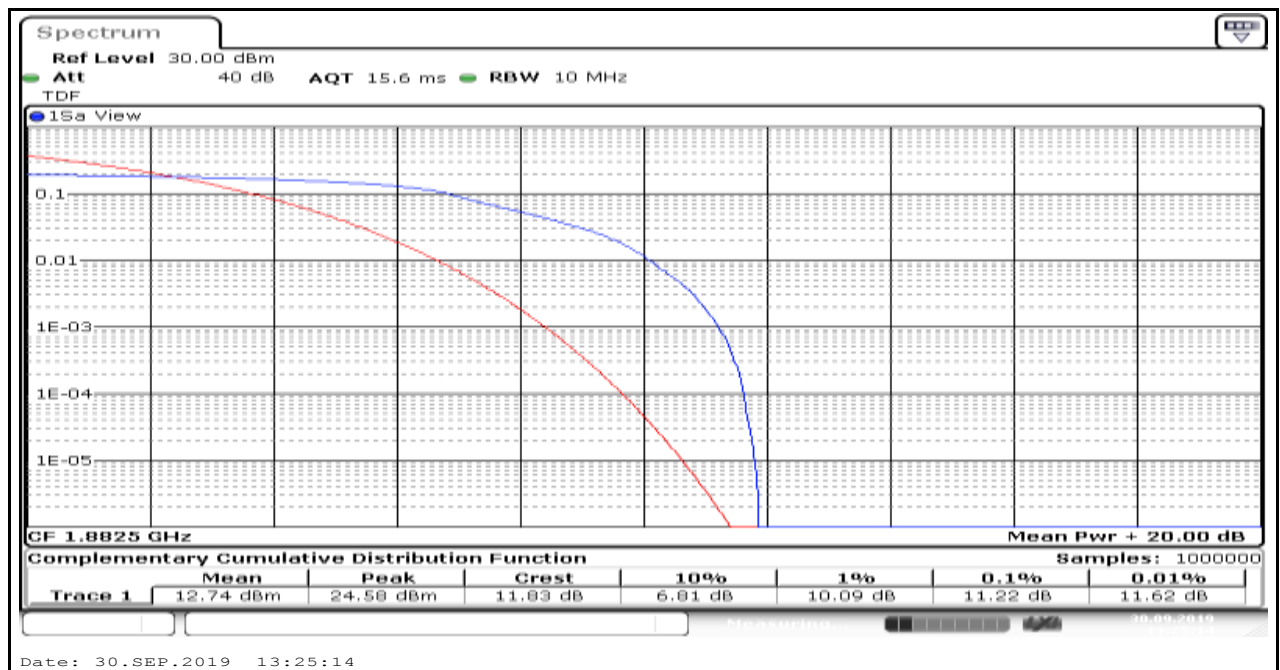
Band25_3MHz_16QAM_26365_6
