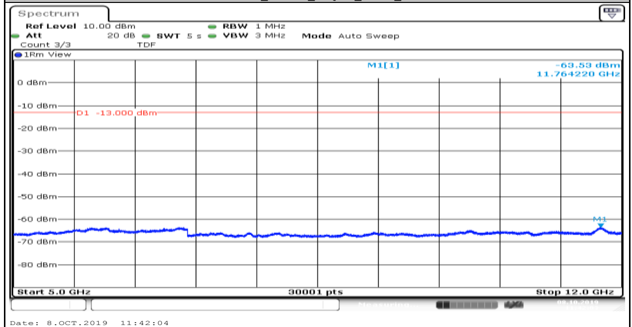
Band5_1.4MHz_16QAM_20643_1
