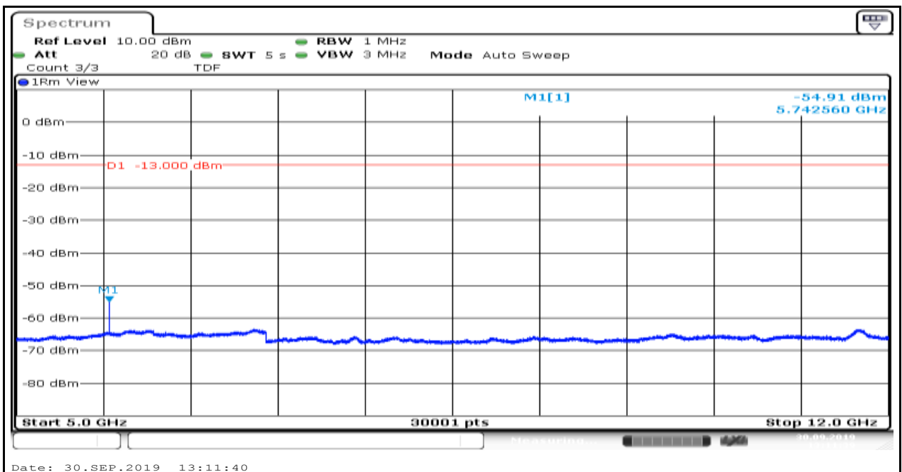
Band25_1.4MHz_16QAM_26683_6
