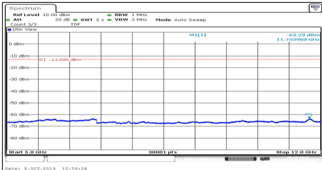
Band12_1.4MHz_QPSK_23017_1
