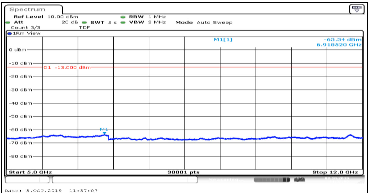
Band5_1.4MHz_QPSK_20643_1
