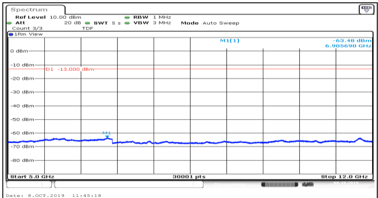
Band5_1.4MHz_16QAM_20525_6
