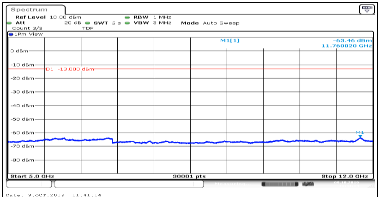
Band13_5MHz_QPSK_23255_6
