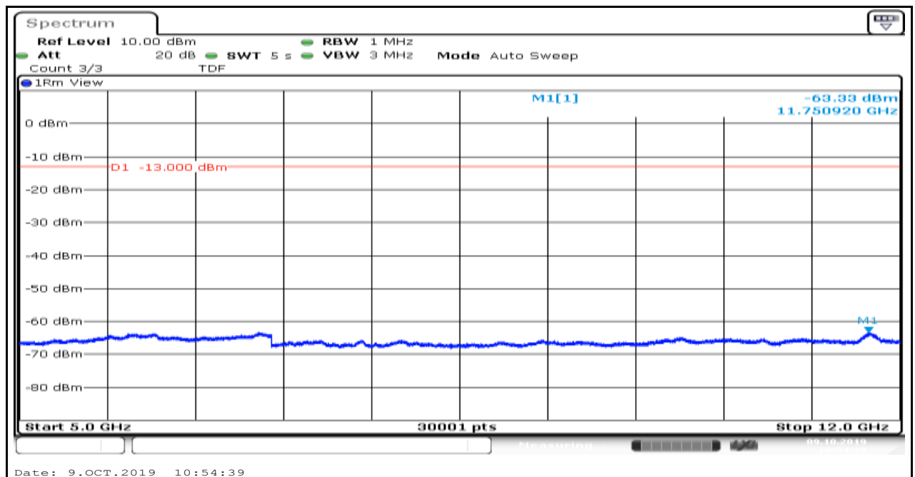
Band12_1.4MHz_16QAM_23095_6
