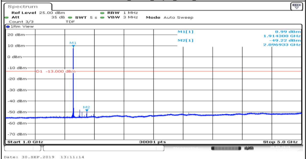
Band25_1.4MHz_16QAM_26683_6
