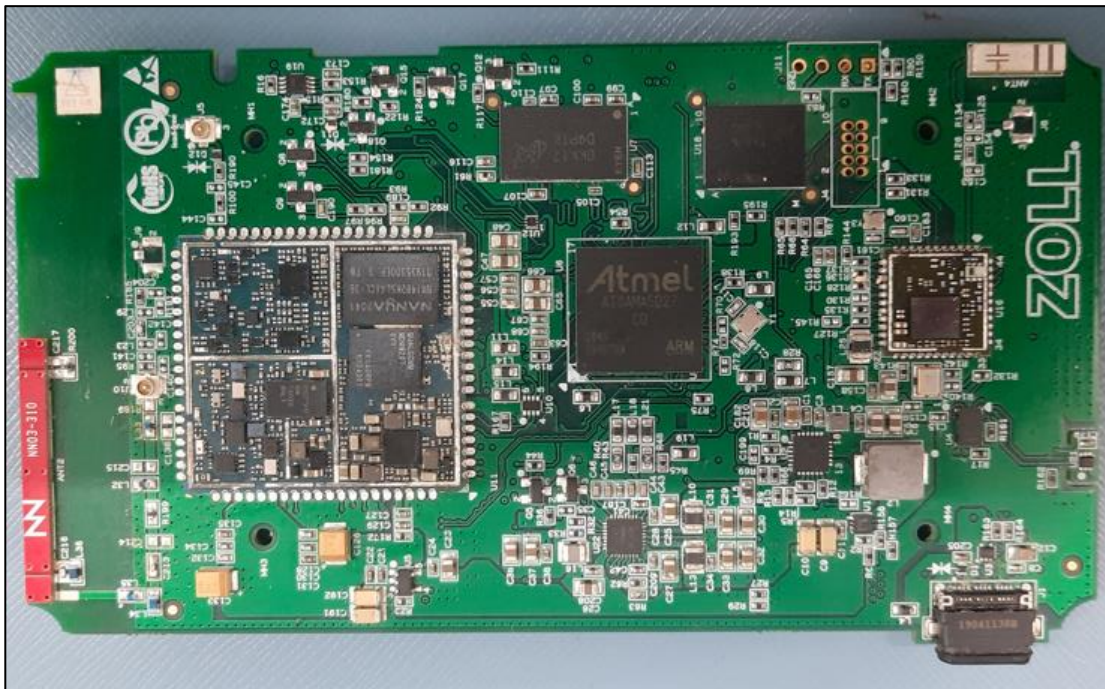
Photo 6: Module Shield open view
