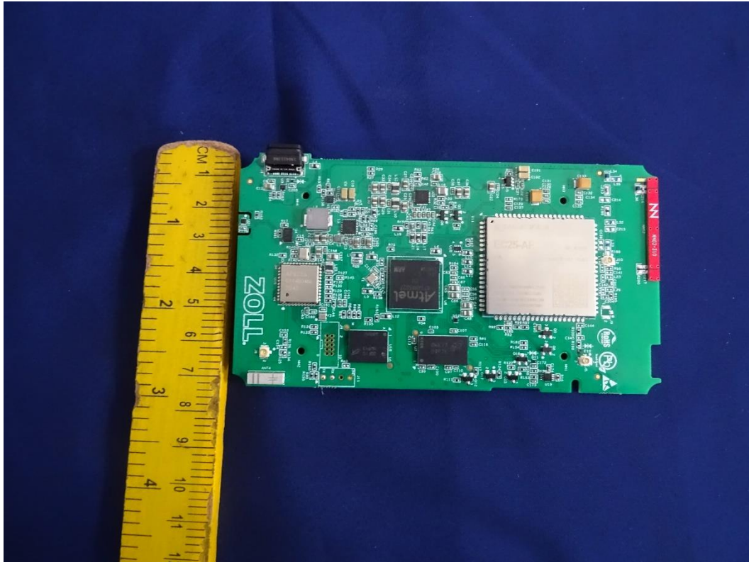
Photo 10: PCB Dimensional view
