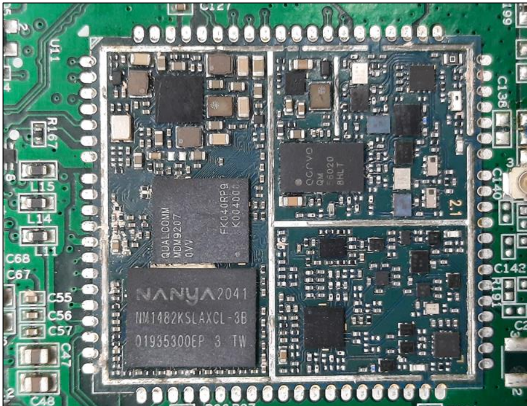
Photo 8: LTE Module Shield open view
