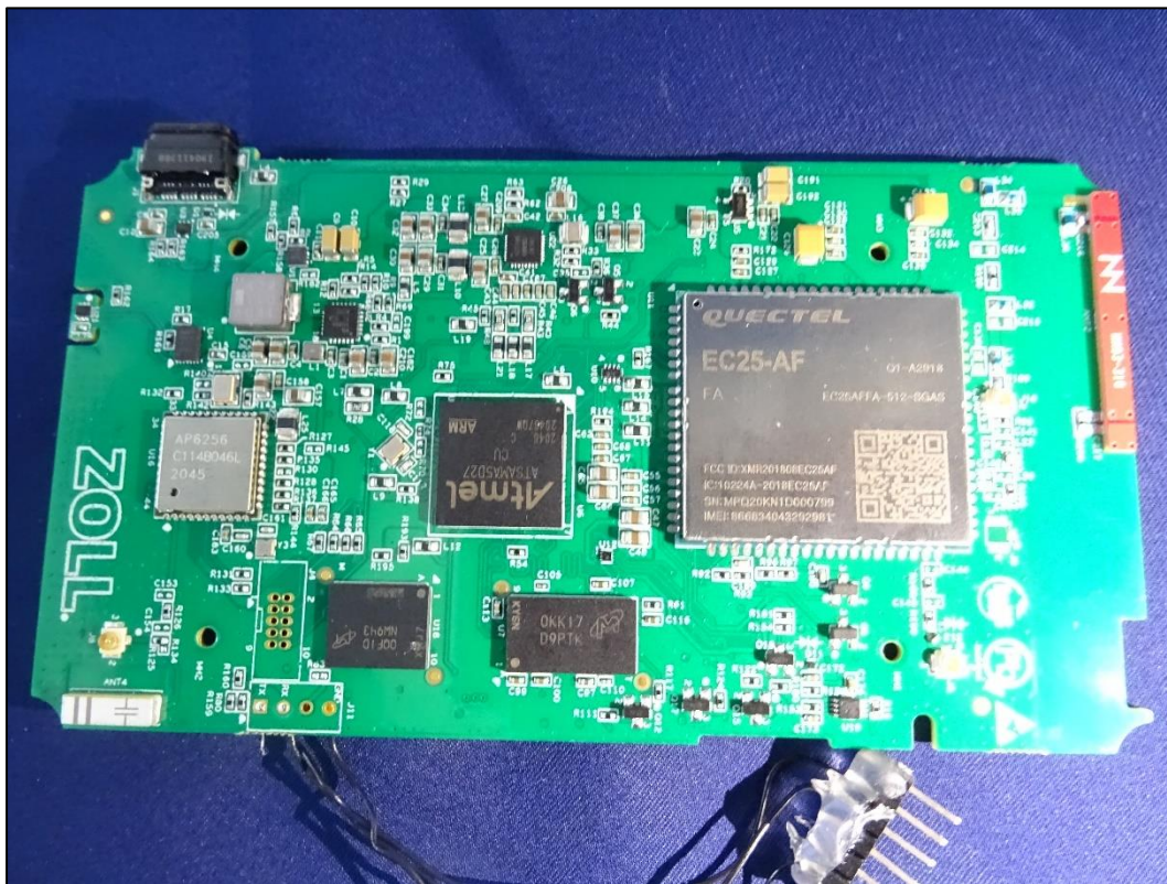
Photo 4: PCB Top view
