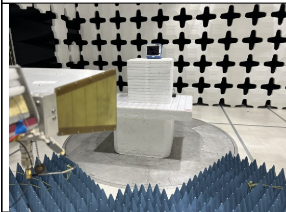
RE Test above 1GHz Front View
