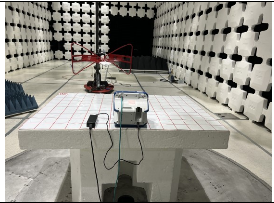
RE Test below 1GHz Rear View
