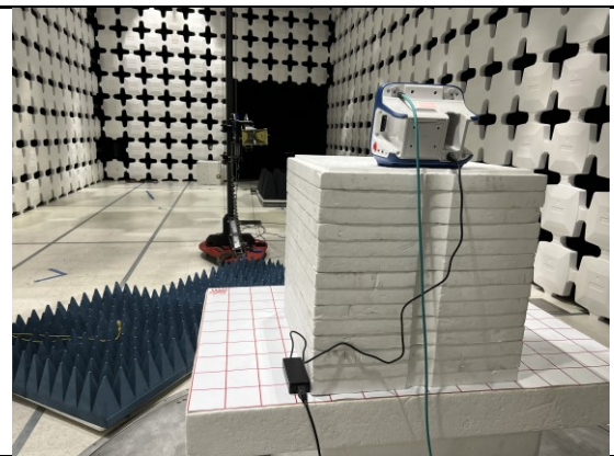
RE Test above 1GHz Rear View
