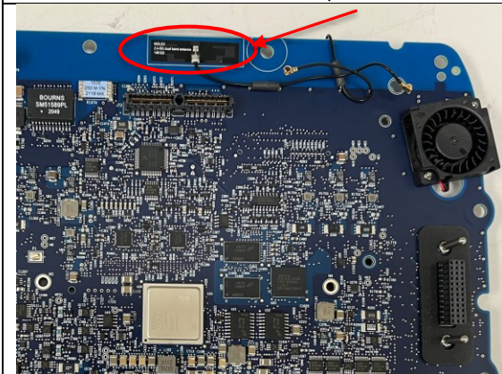
Secondary Antenna View (Ant2)
