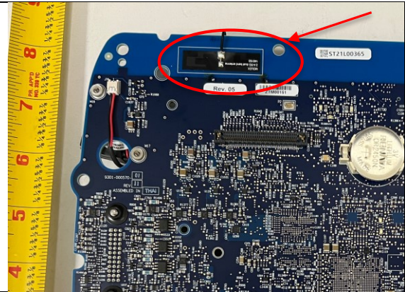
Primary Antenna View (Ant1)
