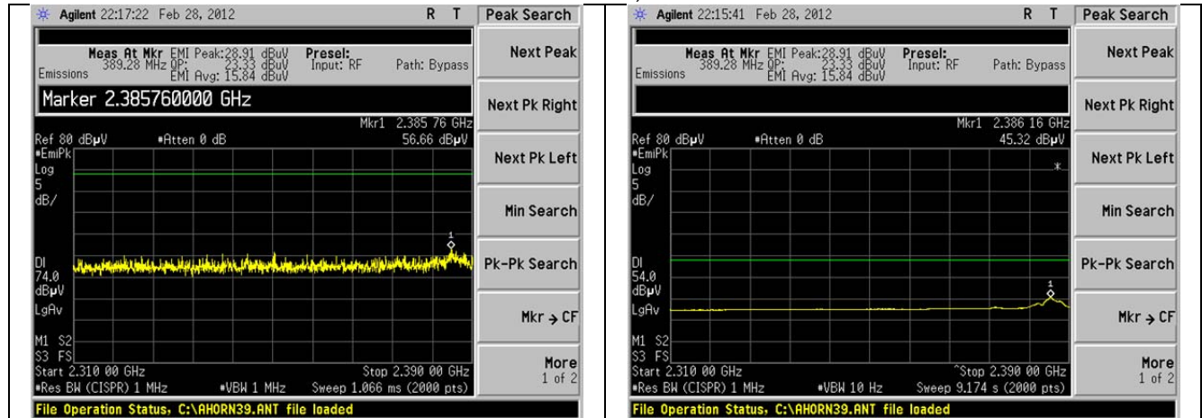
2.4 GHz WLAN 1Mbps. Peak
