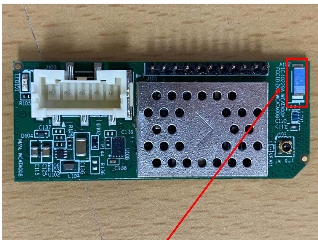
TX Antenna
