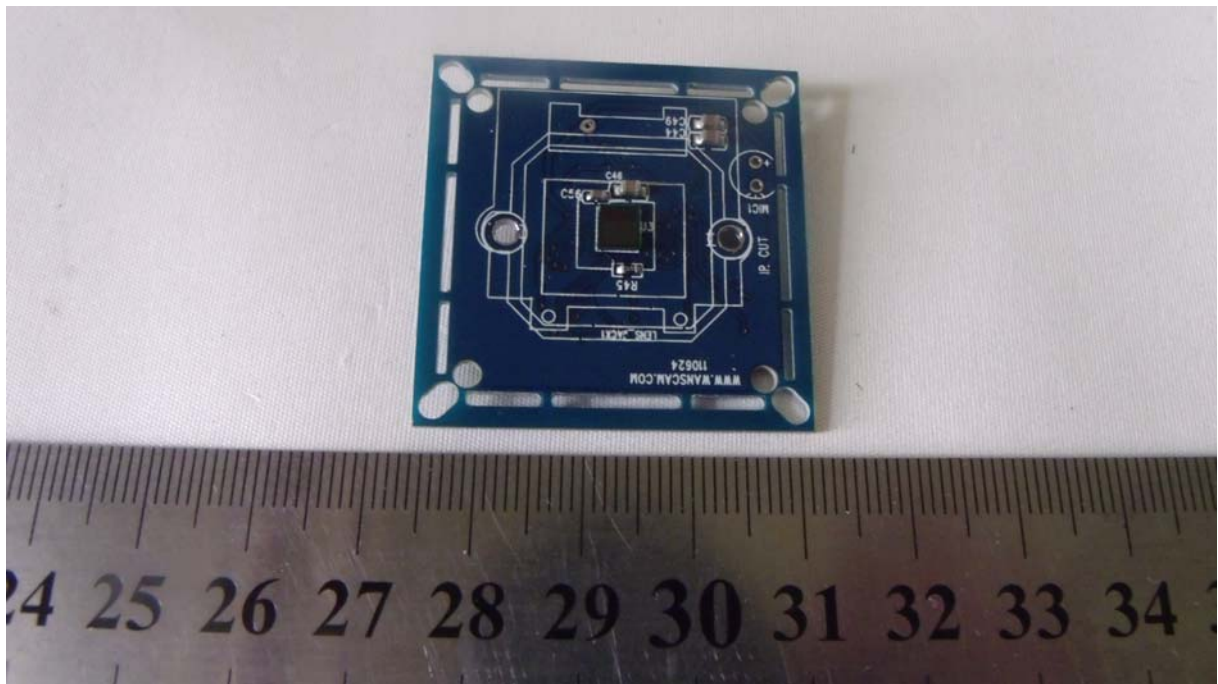
Camera Board Top Lens off View
