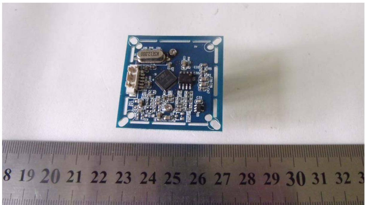
Camera Board Bottom View
