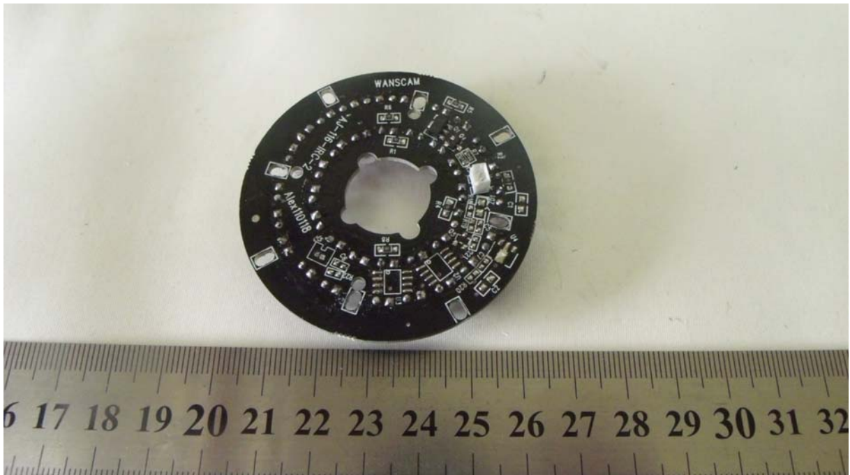
LED Board Bottom View
