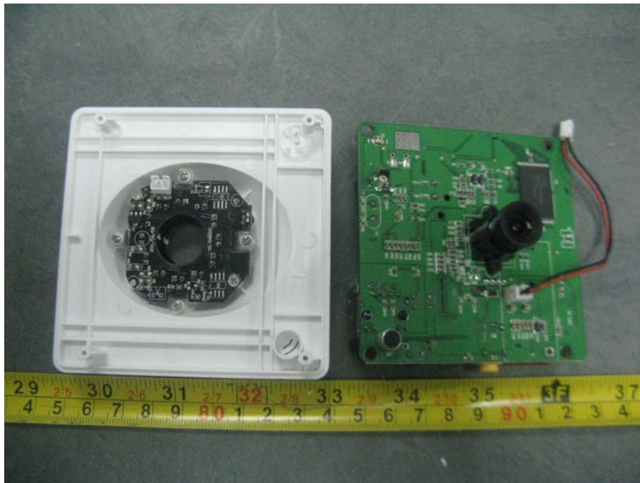
EUT-Internal View 2
