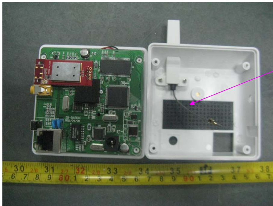
EUT-Internal View 1
