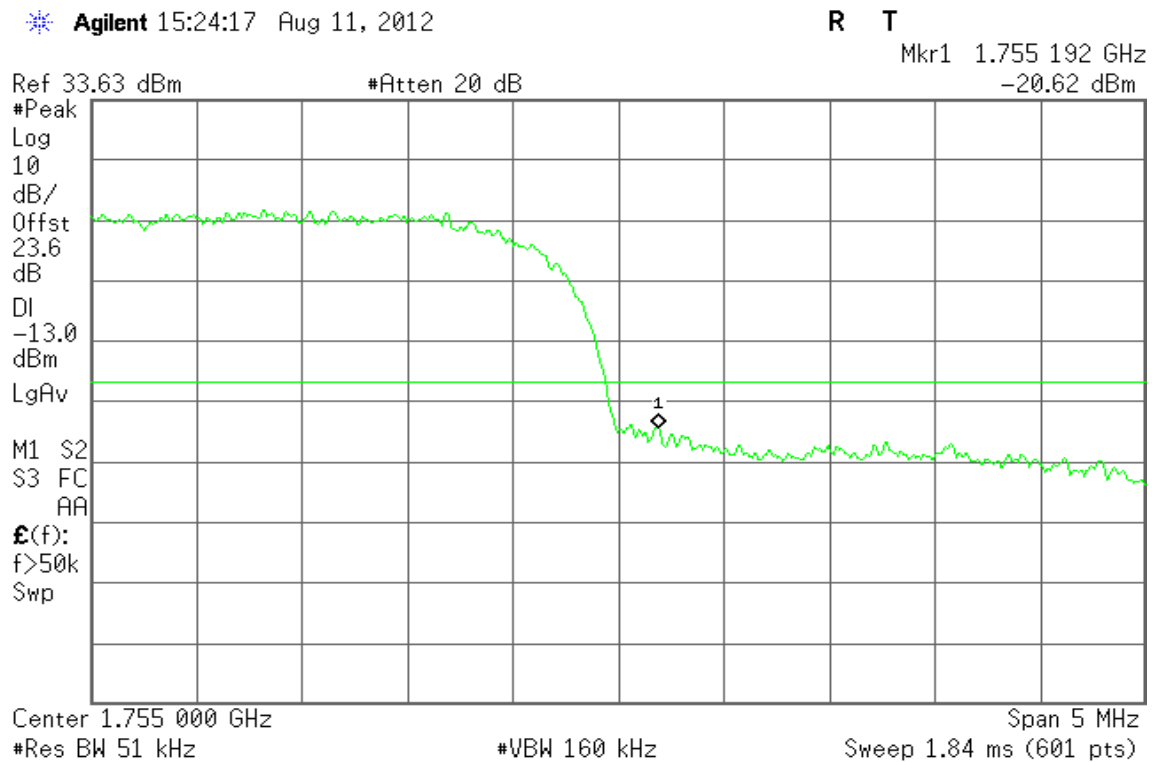
Figure 12-2: Band Edge emissions –HSUPA Band IV CH High
