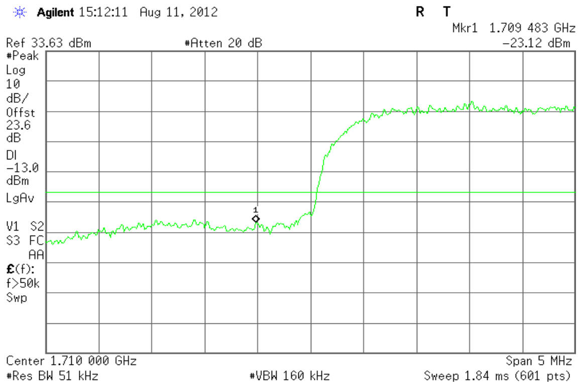
Figure 8-1: Band Edge emissions –WCDMA Band IV CH Low
