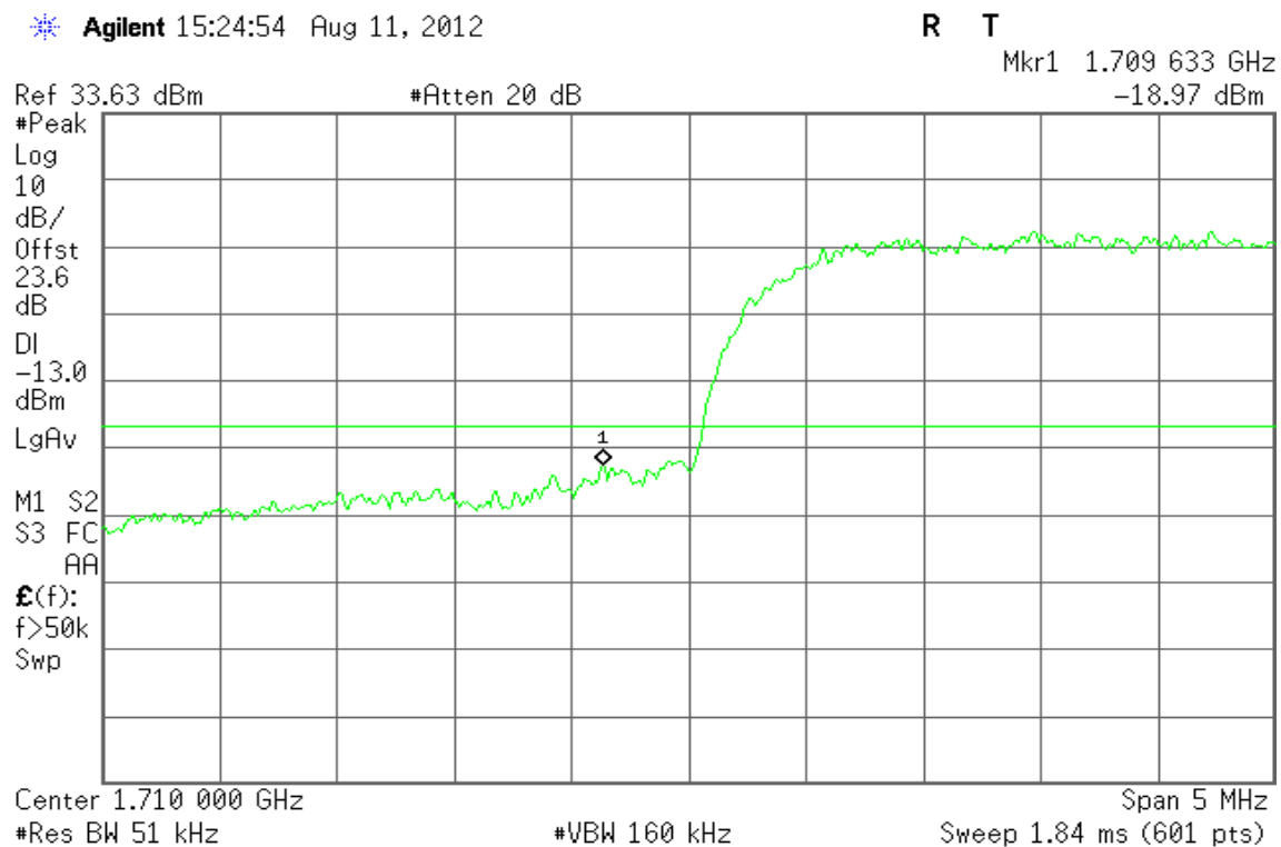
Figure 12-1: Band Edge emissions –HSUPA Band IV CH Low
