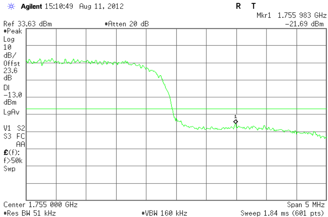
Figure 8-2: Band Edge emissions –WCDMA Band IV CH High
