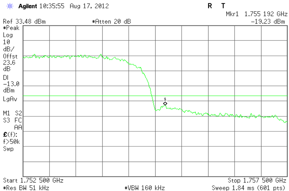
Figure 14-2: Band Edge emissions –HSUPA Band IV CH High
