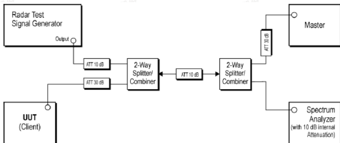
Figure 7-1. Test Setup
