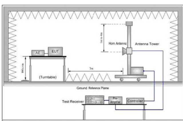
Figure 3. Above 1 GHz
